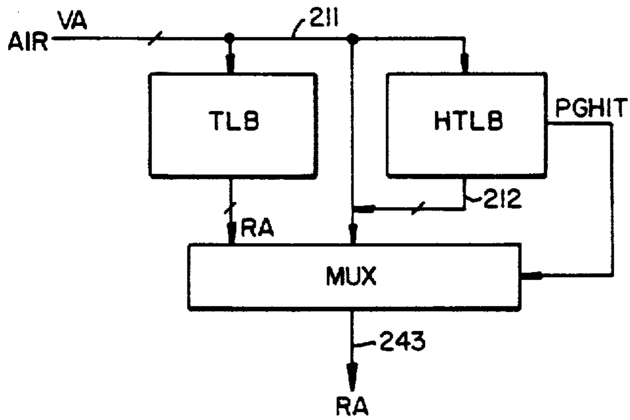
TLB SUBSYSTEM
