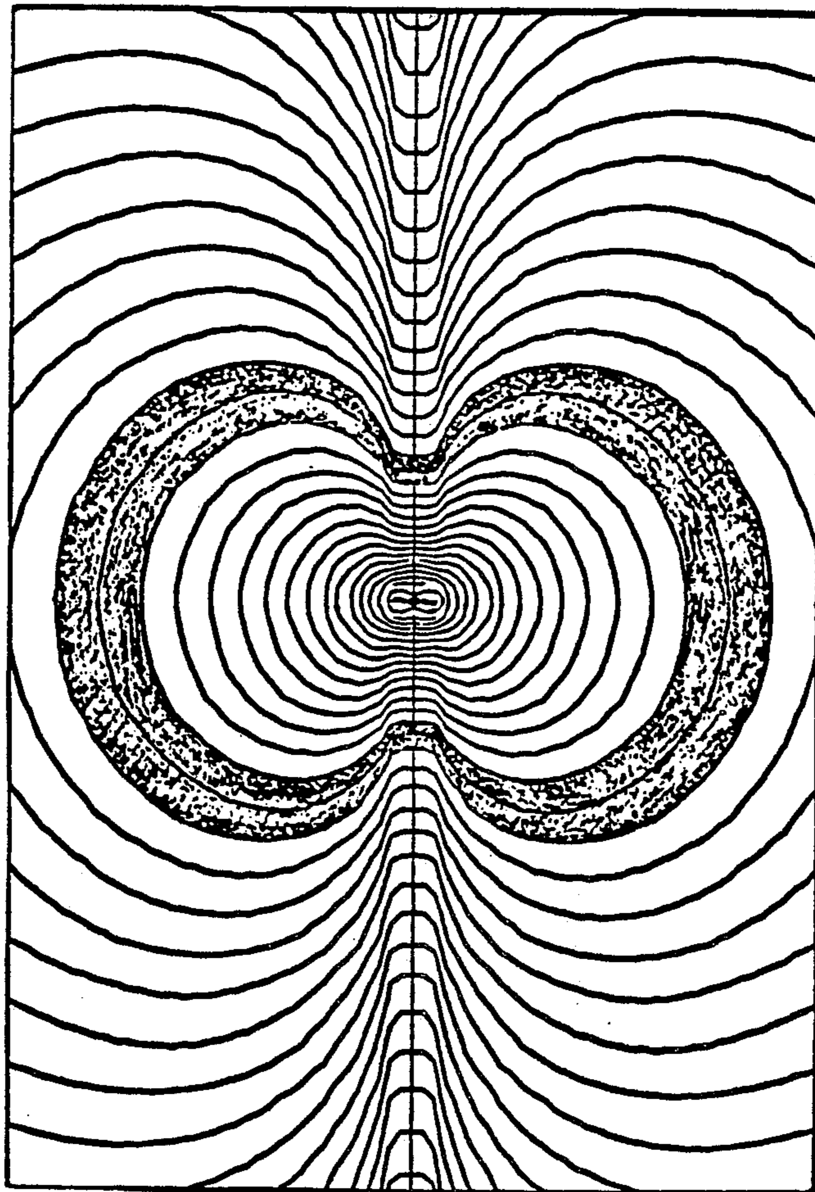
LINES OF CONSTANT AMPLITUDE AROUND A SOURCE
