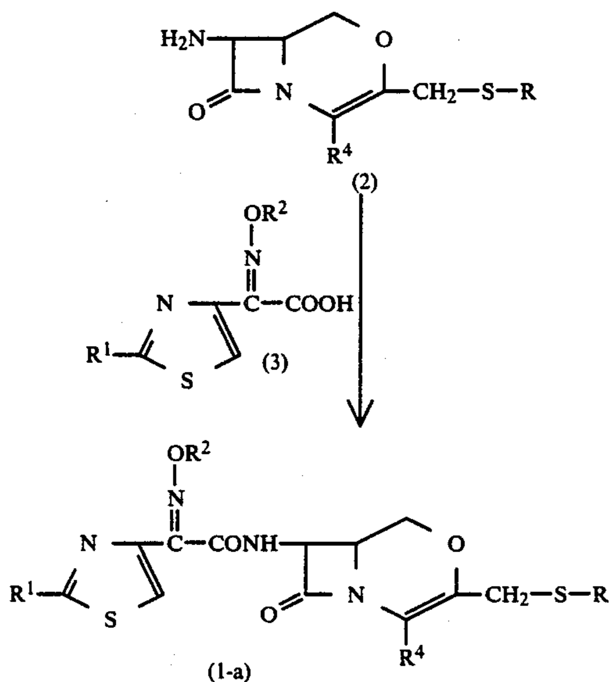
Reaction scheme-1
