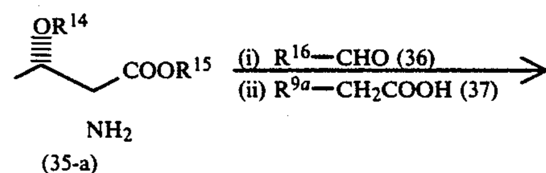
Reaction scheme-12
