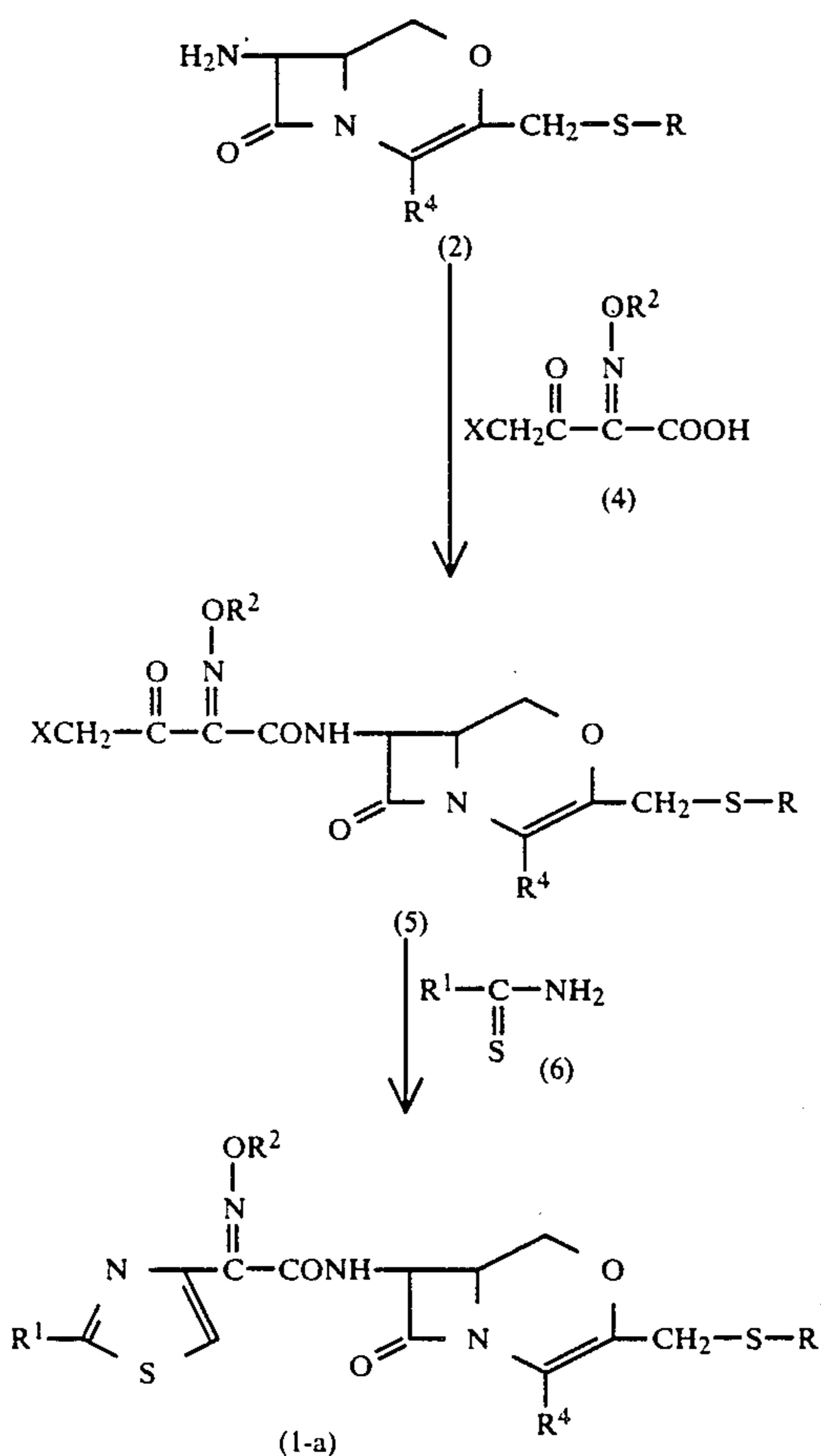
Reaction scheme-2
