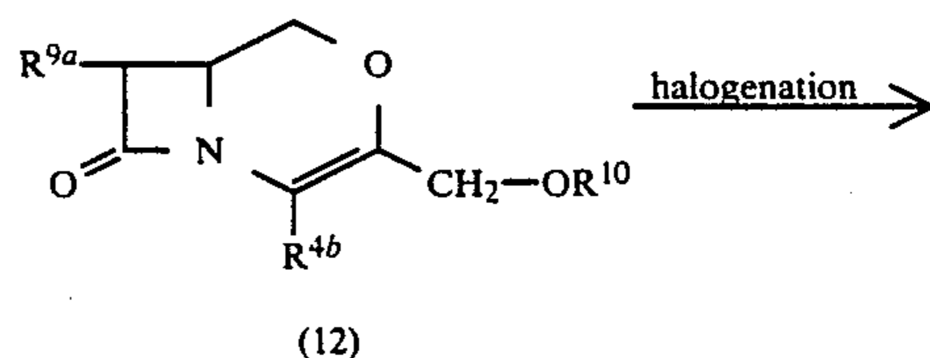
Reaction scheme-8
