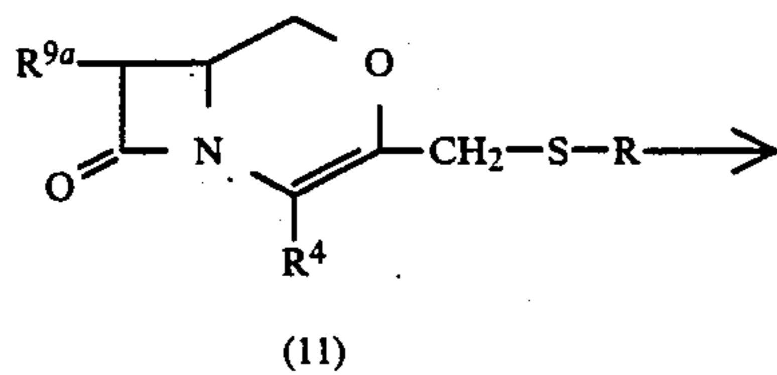
Reaction scheme-7
