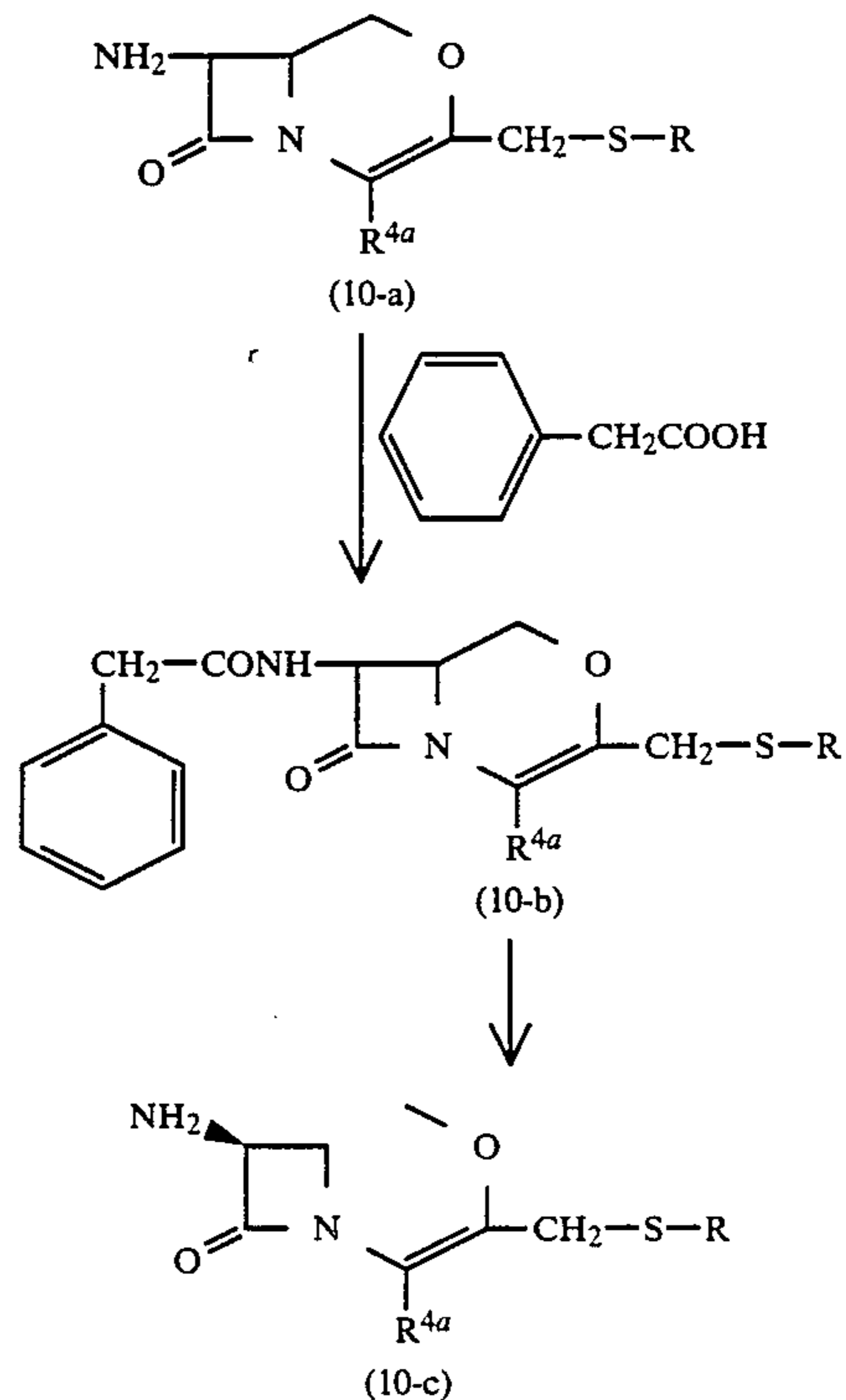
Reaction scheme-9
