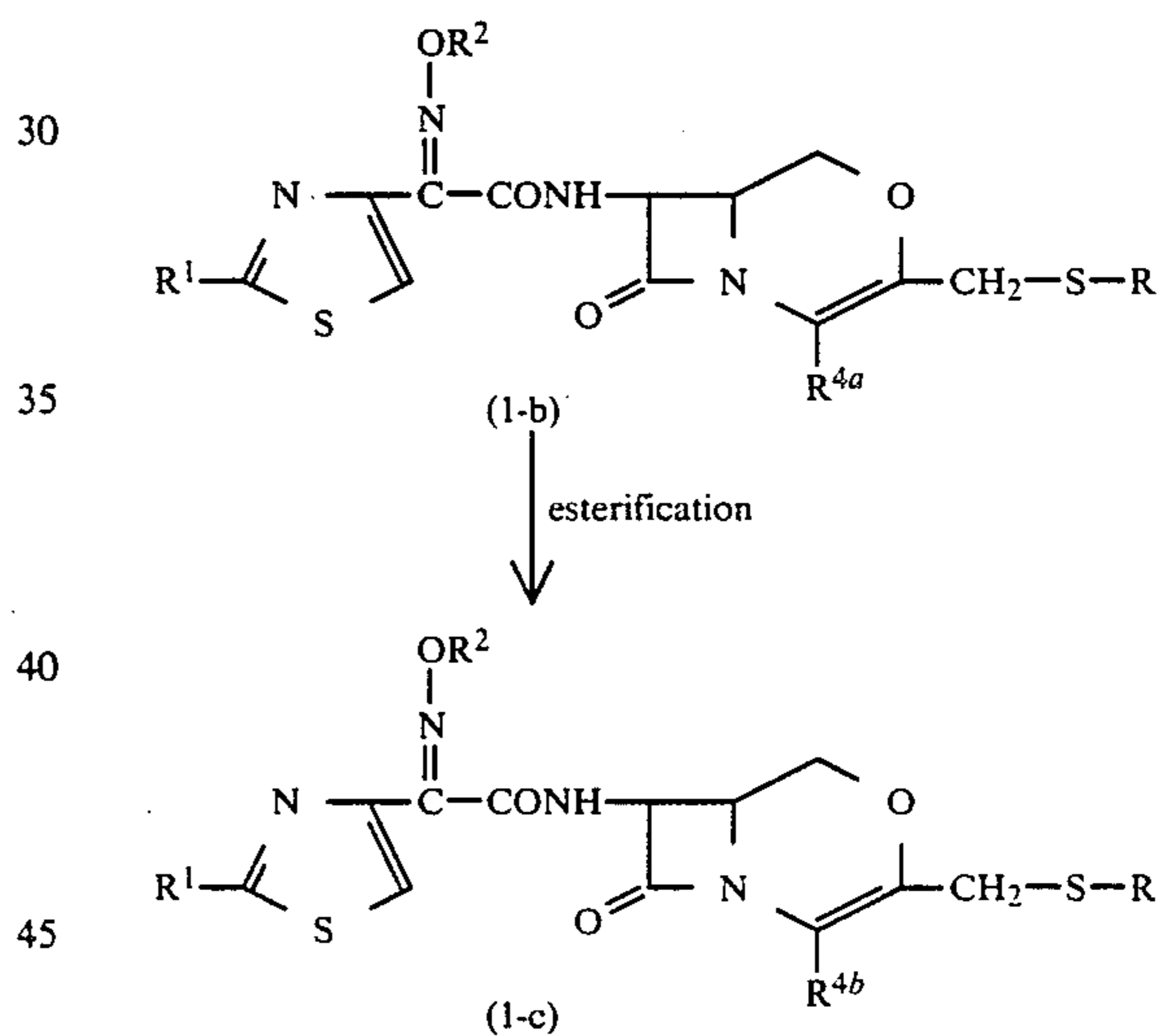
Reaction scheme-3
