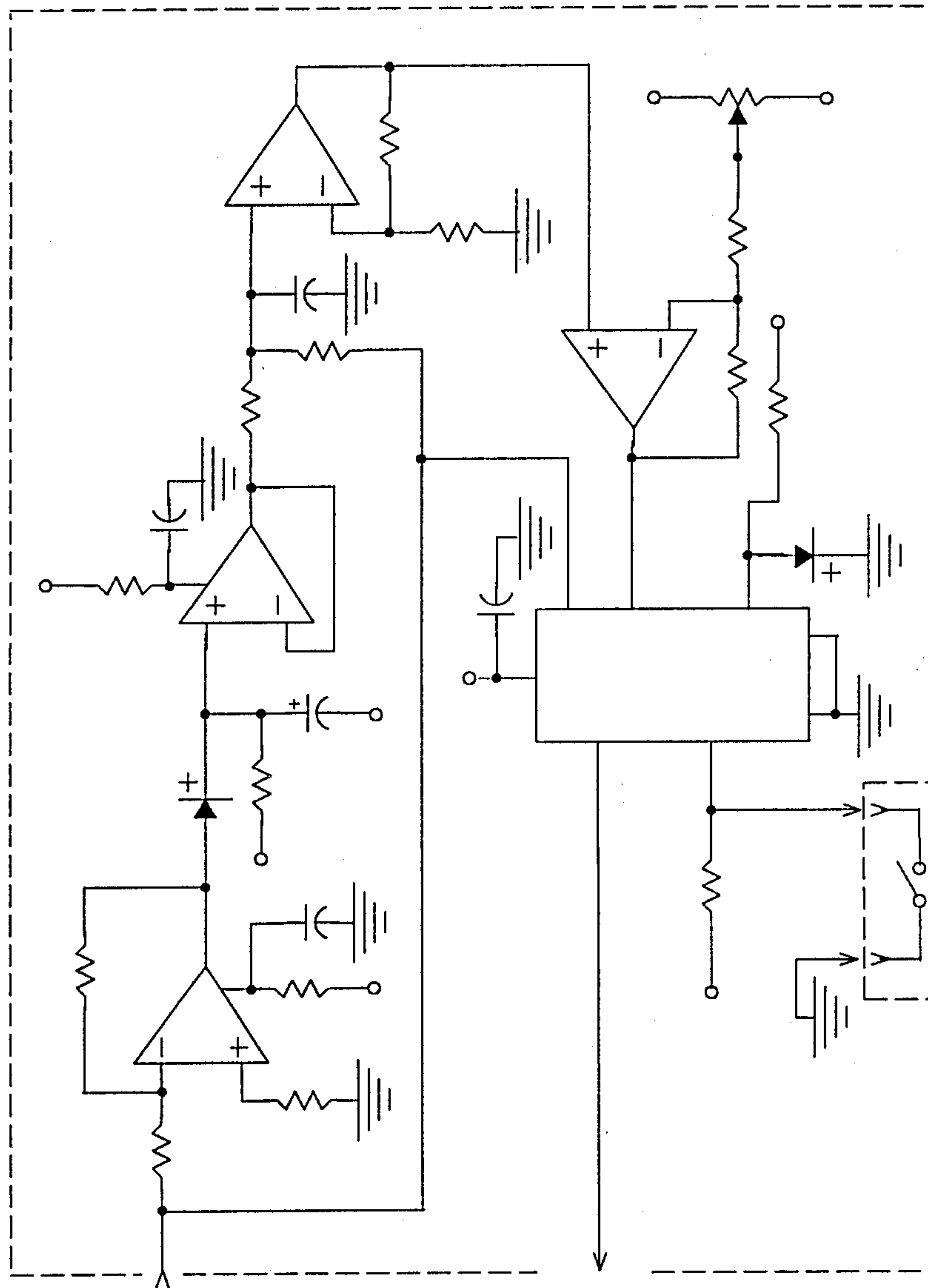
AUTO-POSITION CONTROL CIRCUIT
