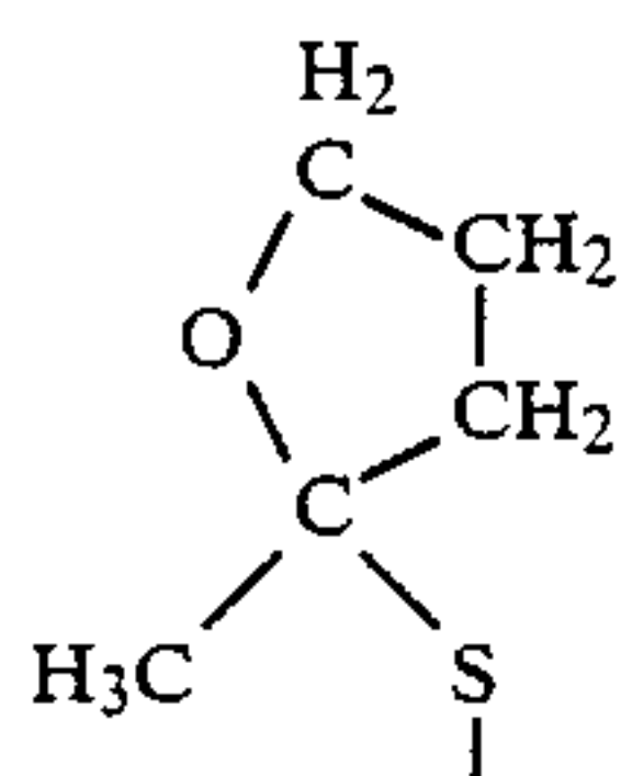
2-methyl tetrahydrofuran
