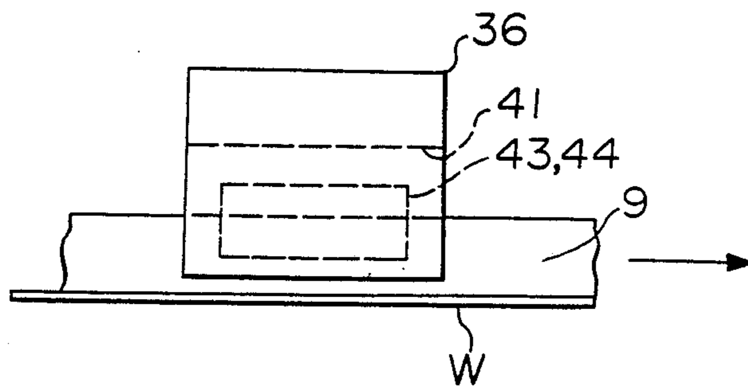
FIGURE 7B
