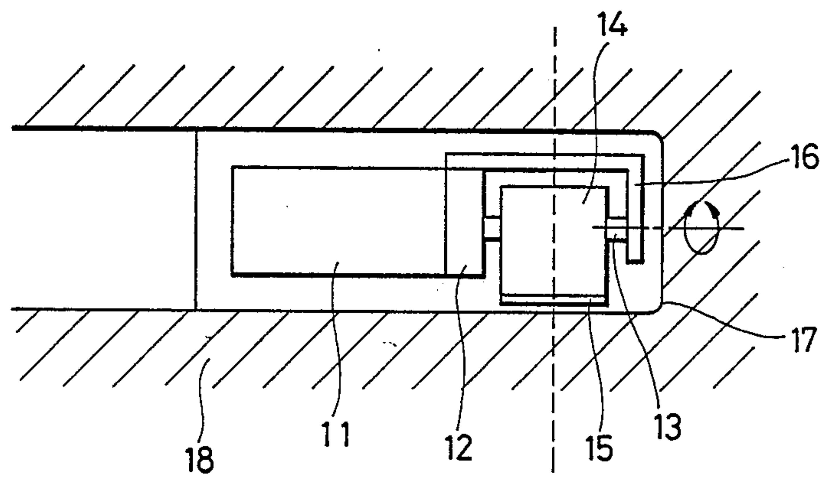
FIG. 2 PRIOR ART
