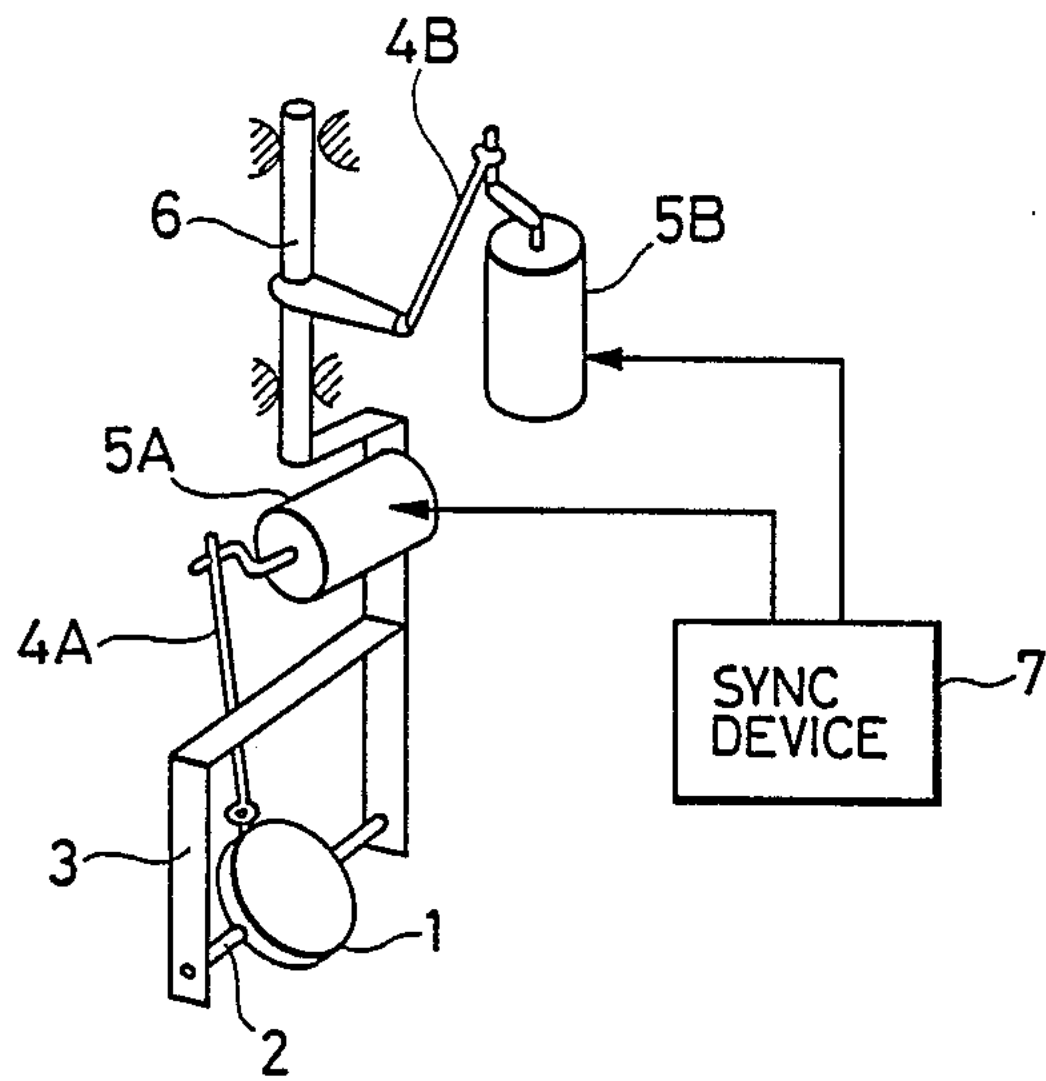
FIG. 1 PRIOR ART
