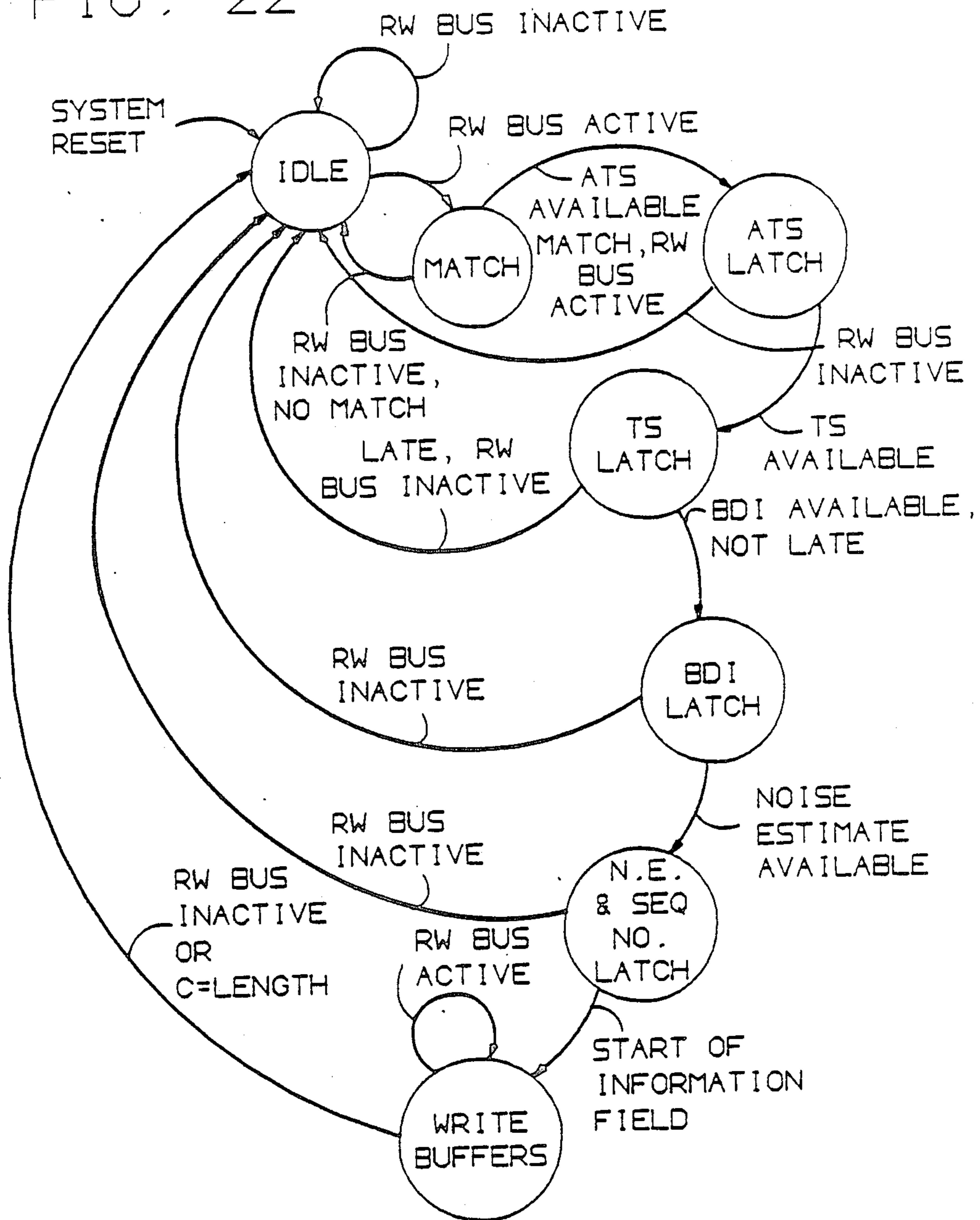
RECEIVE PACKET BUS SEQUENCER 1910
