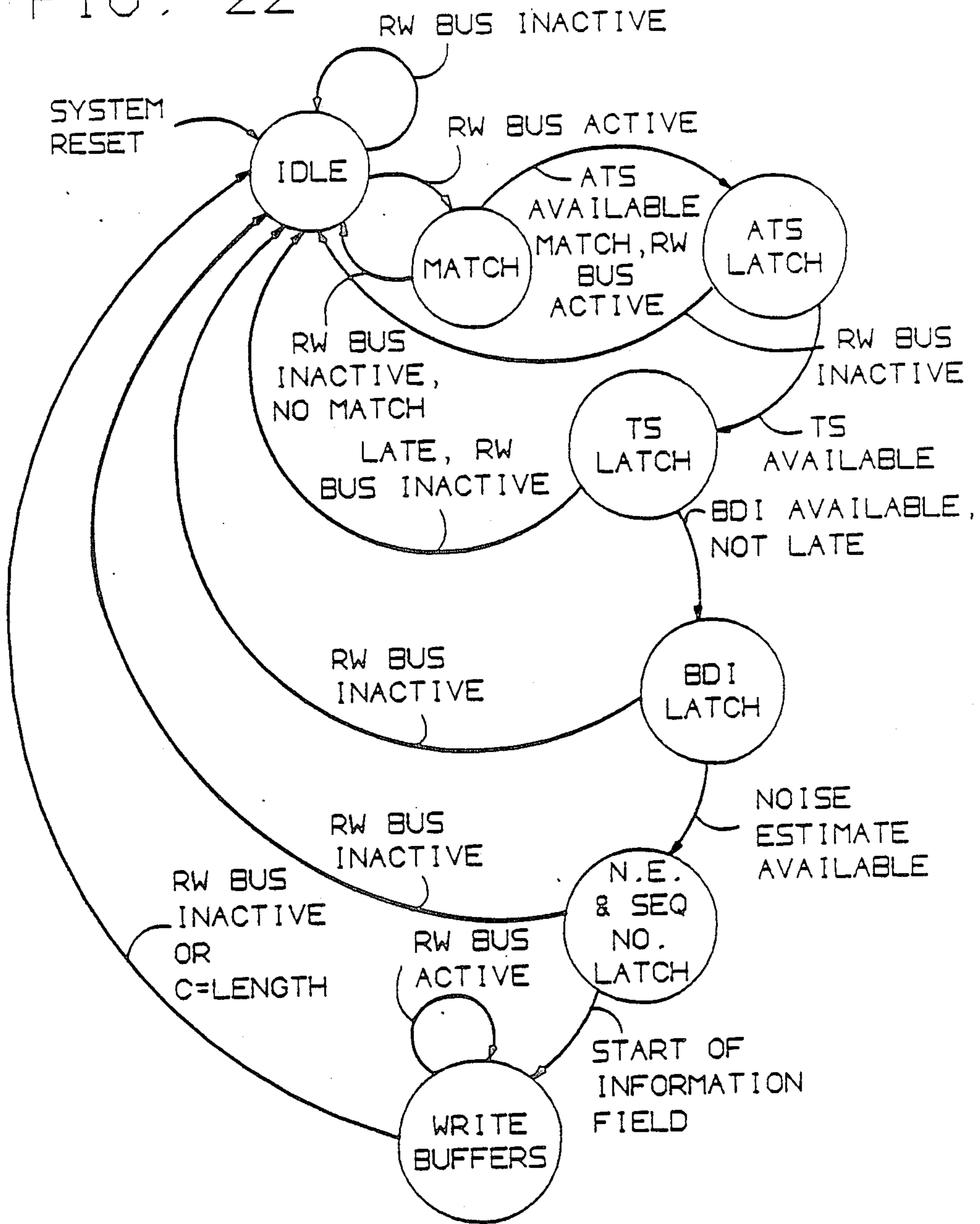
RECEIVE PACKET BUS SEQUENCER 1910
