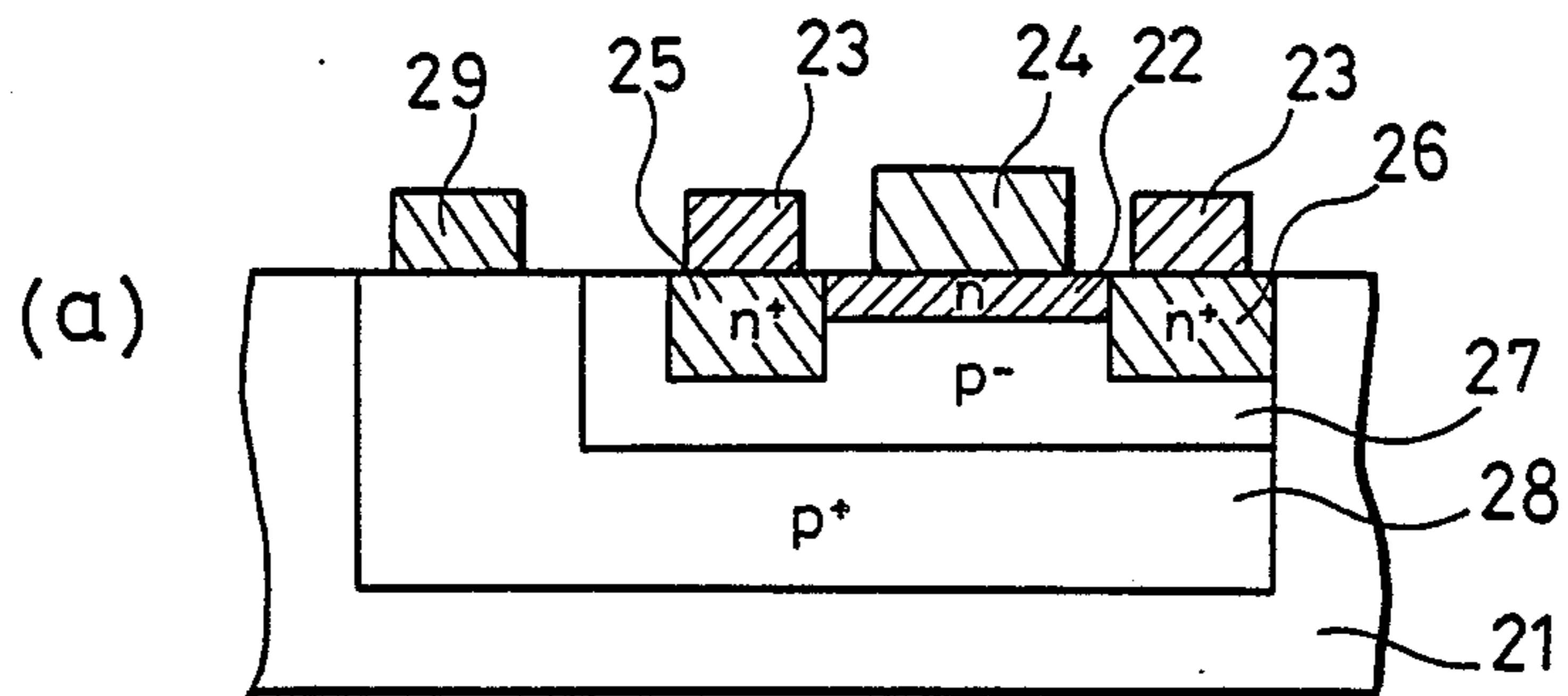
FIG. 7. (PRIOR ART)
