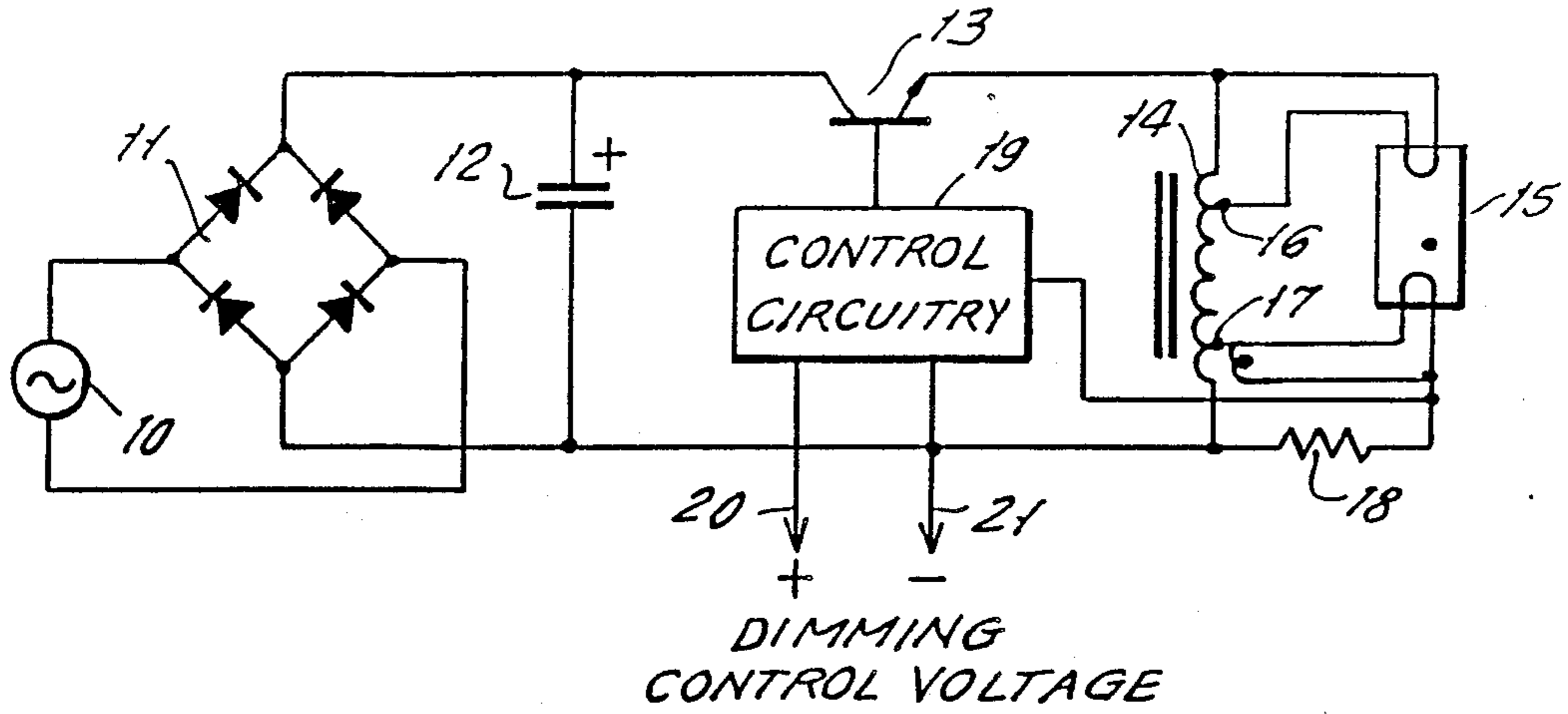
FIG. 1. (PRIOR ART)
