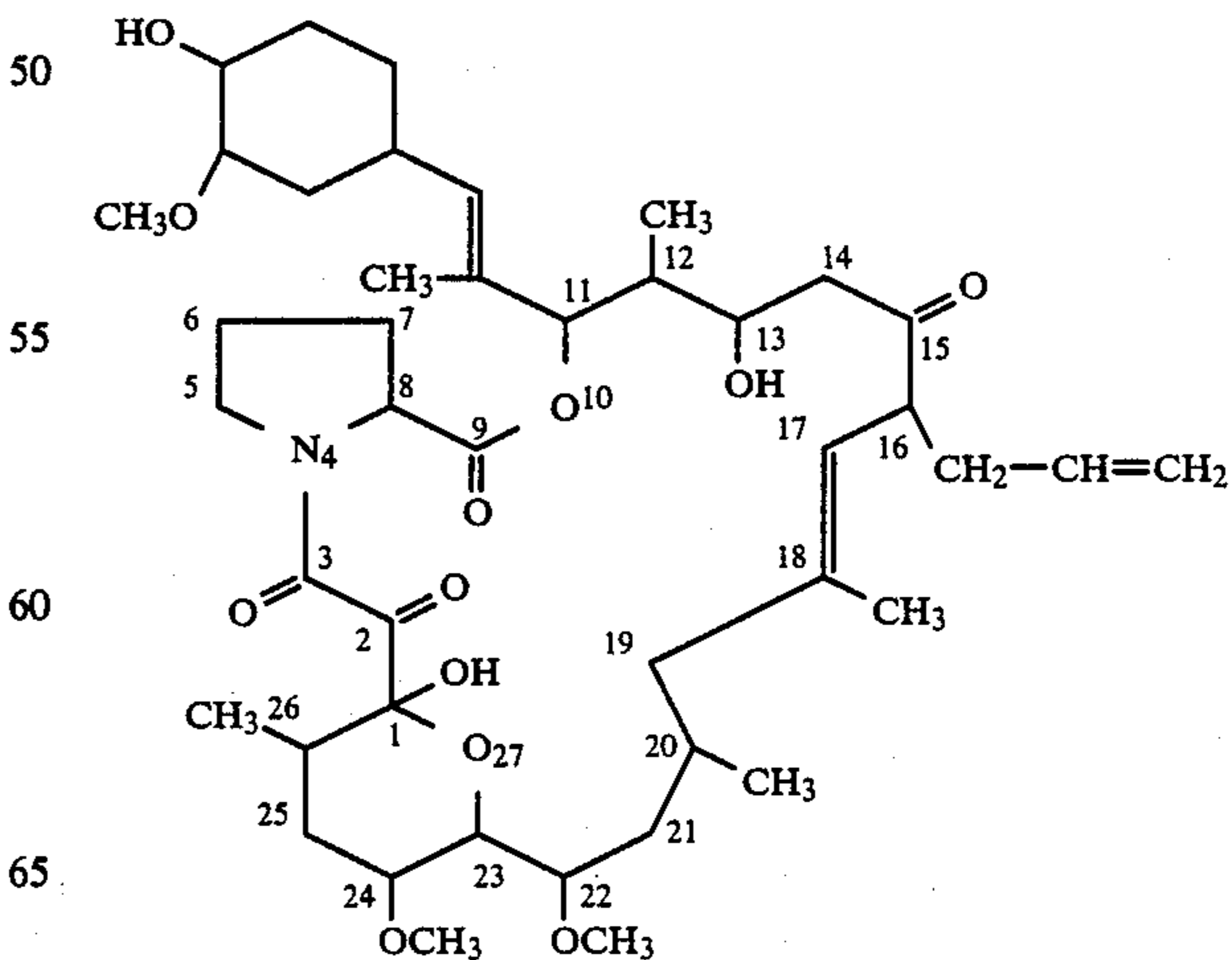
16-Allyl-1,13-dihydroxy-11-[2-(4-hydroxy-3-
