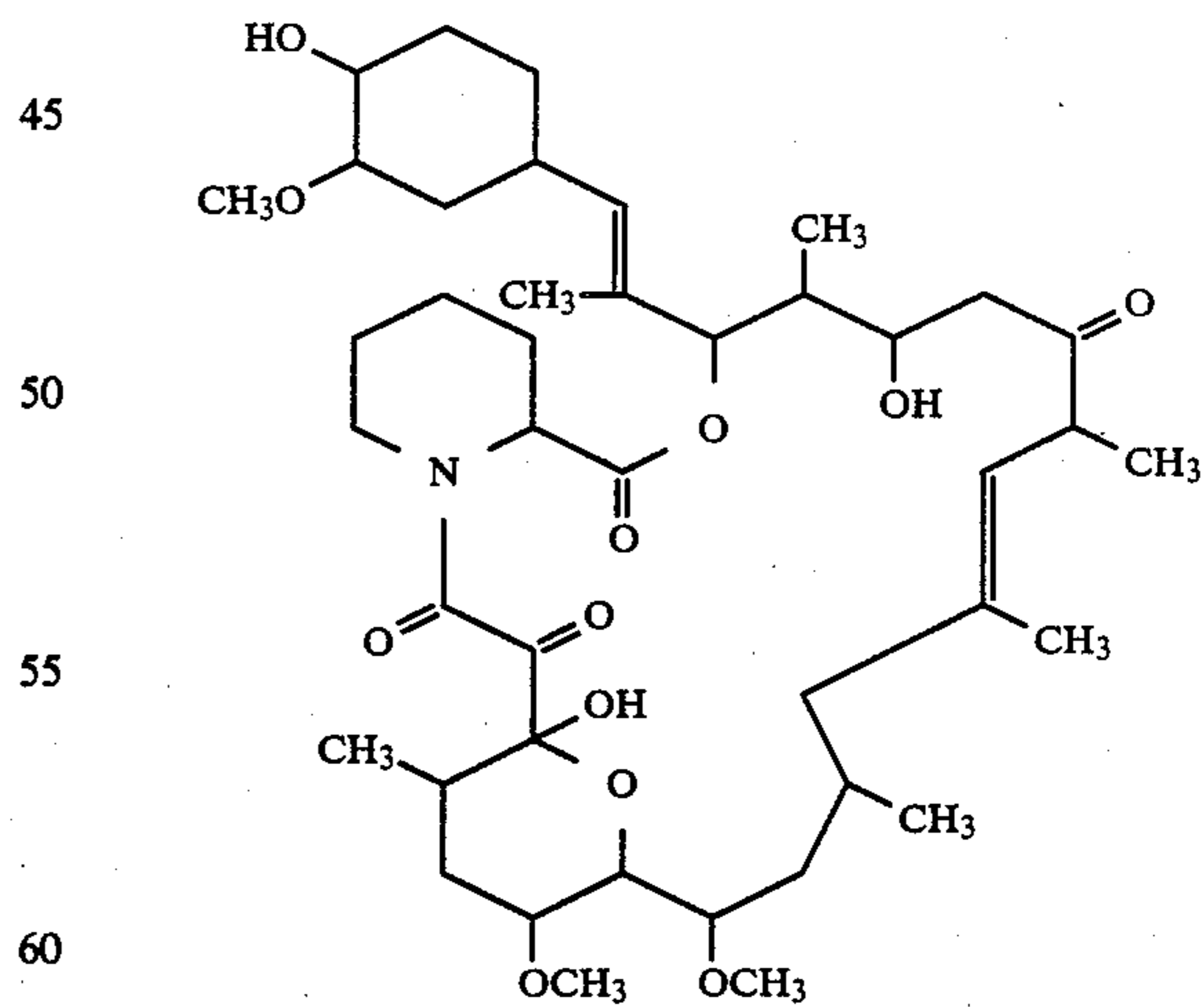
1,14-Dihydroxy-12-[2-(4-hydroxy-3-methoxycyclohexyl)-1-methylvinyl]-23,25-dimethoxy-13,19,17,21,27-pentamethyl-11,28-dioxo-4-azatricyclo[22.3.1.0 4,9 ]-octacos-18-ene-2,3,10,16-tetraone
