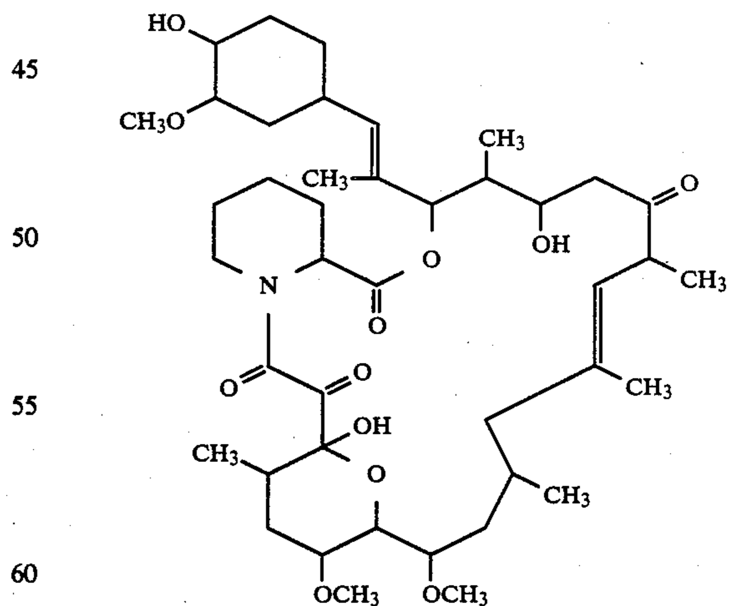
1,14-Dihydroxy-12-[2-(4-hydroxy-3-methoxycyclohexyl)-1-methylvinyl]-23,25-dimethoxy-13,19,17,21,27-pentamethyl-11,28-dioxo-4-azatricyclo[22.3.1.0 4,9 ]-octacos-18-ene-2,3,10,16-tetraone
