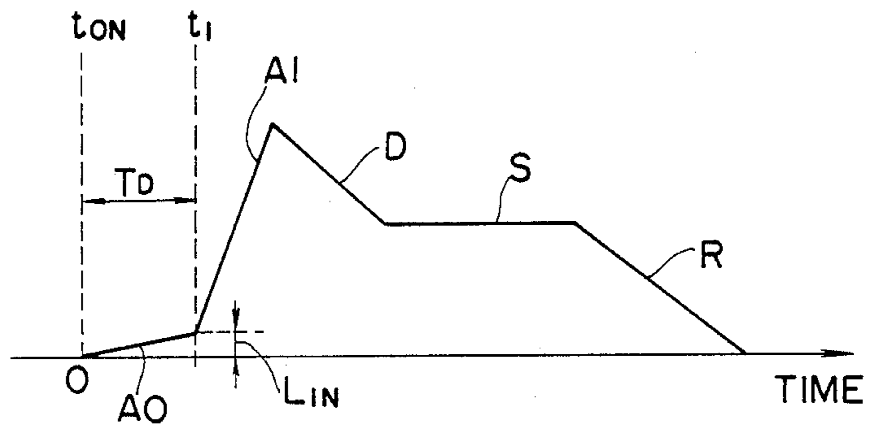
FIG. 11 (PRIOR ART)
