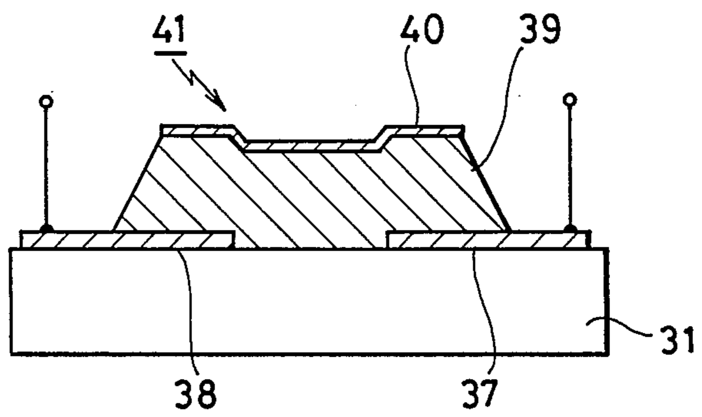
FIG.2 (PRIOR ART)
