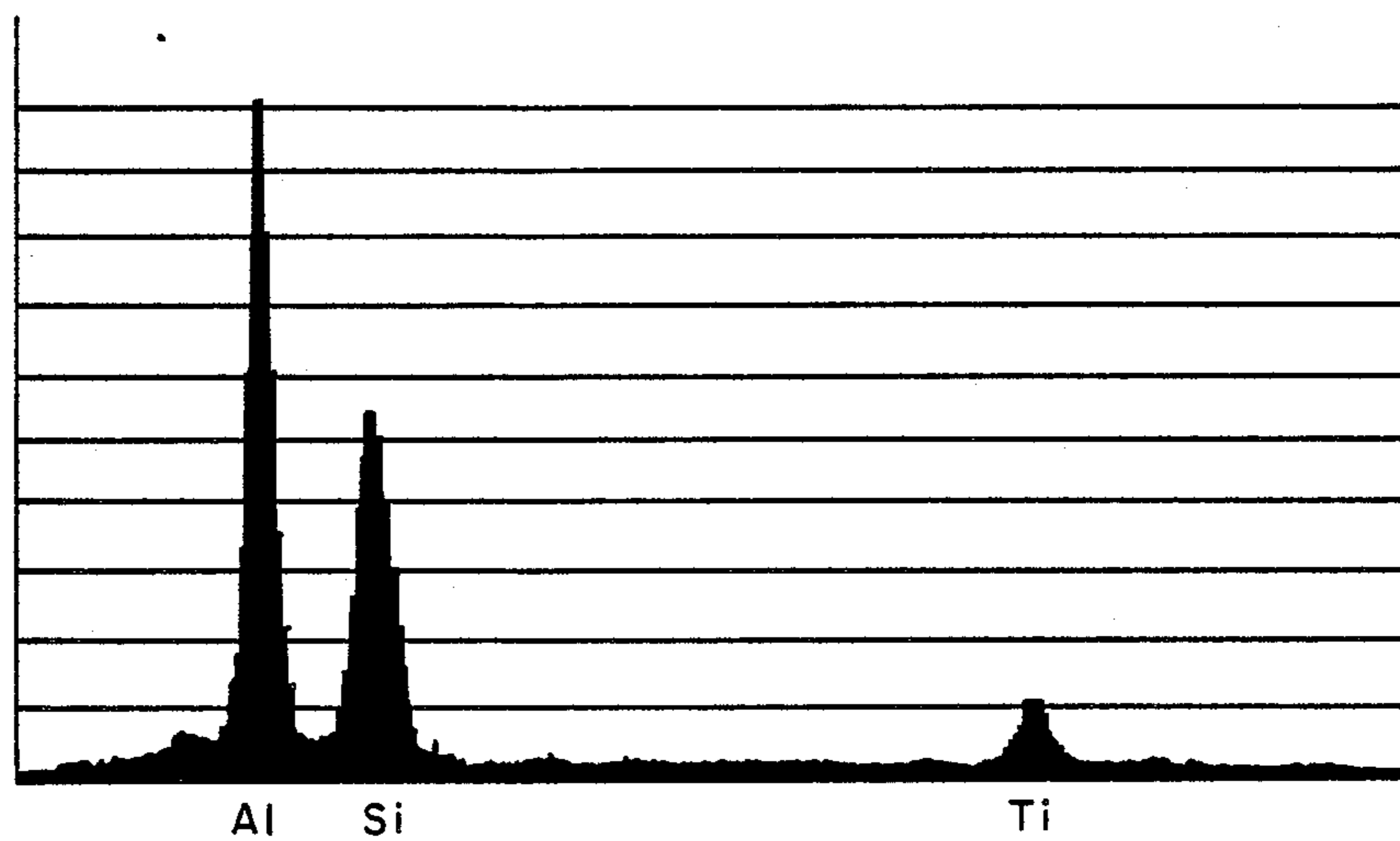
SPOT PROBE AT POINT J OF FIG. 3
