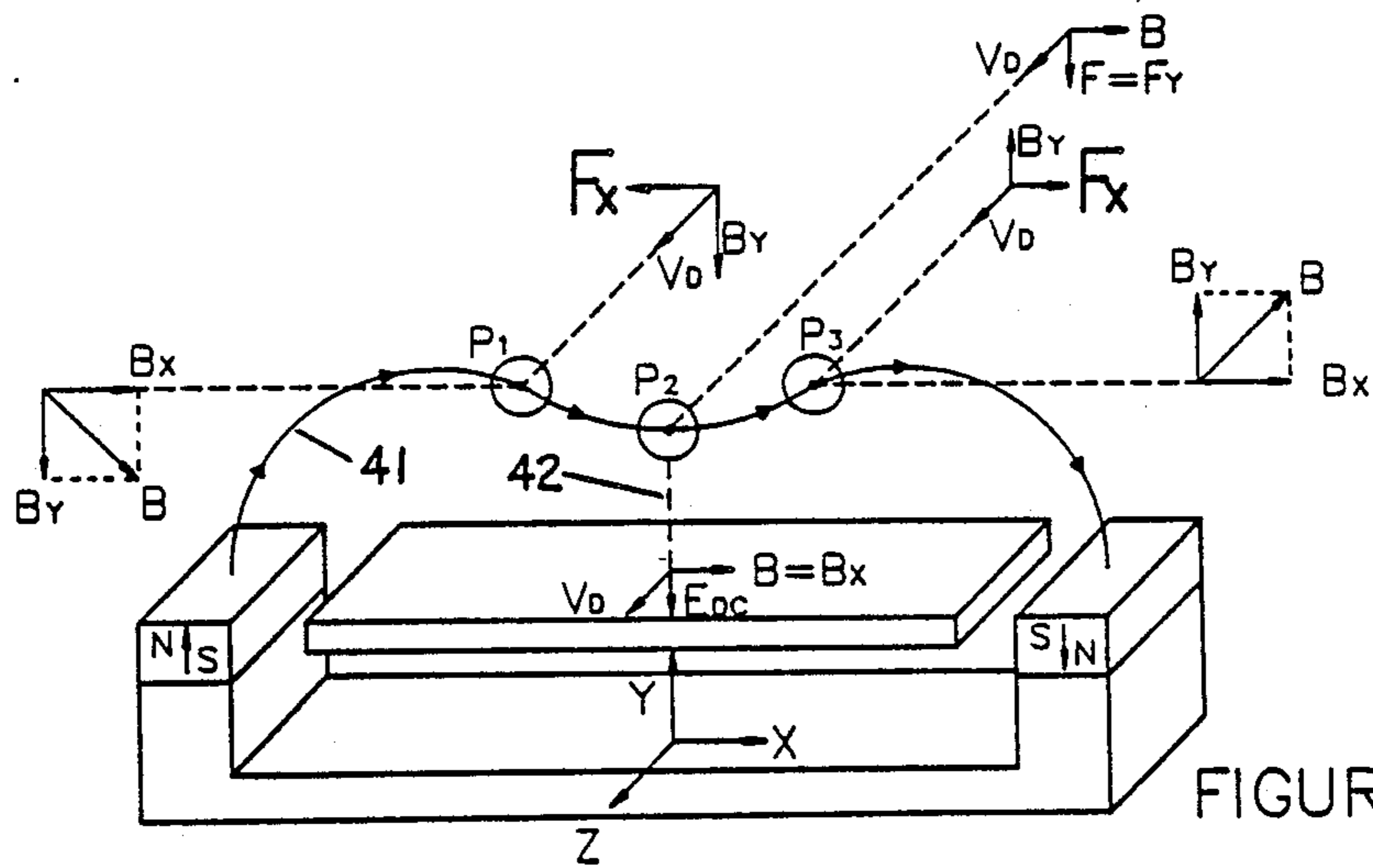
FIGURE 4A (PRIOR ART)
