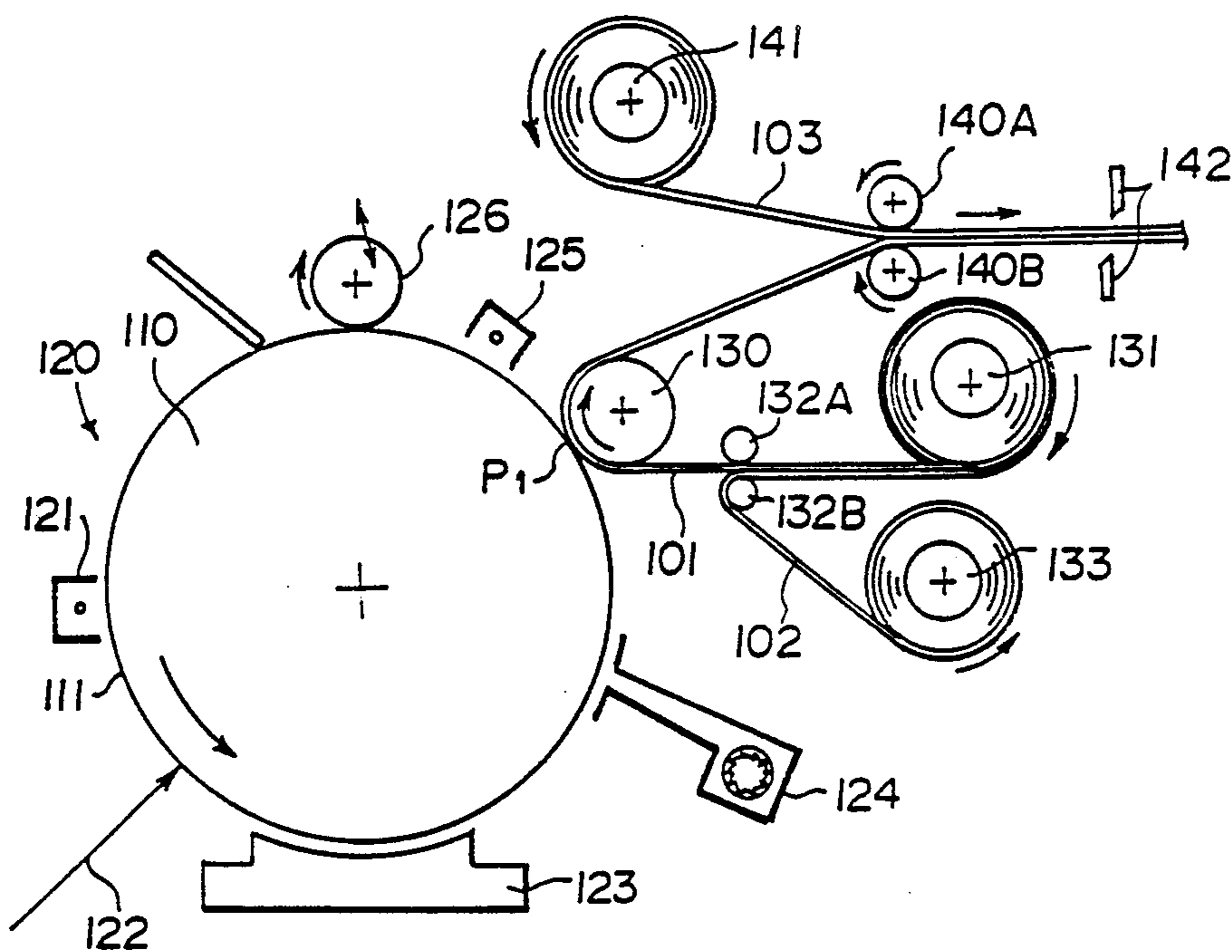
FIG. 8 PRIOR ART
