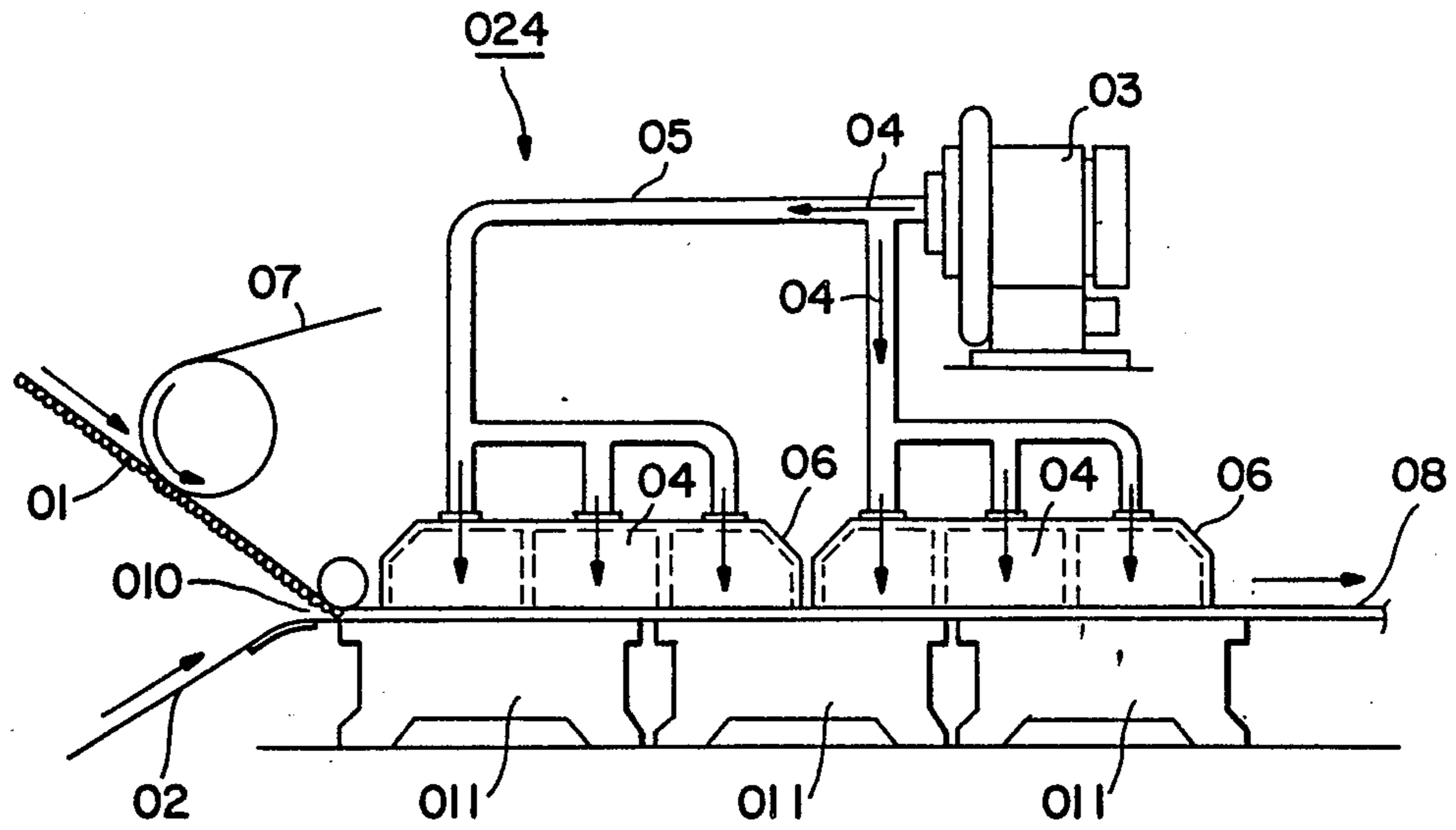
FIG. 5 PRIOR ART
