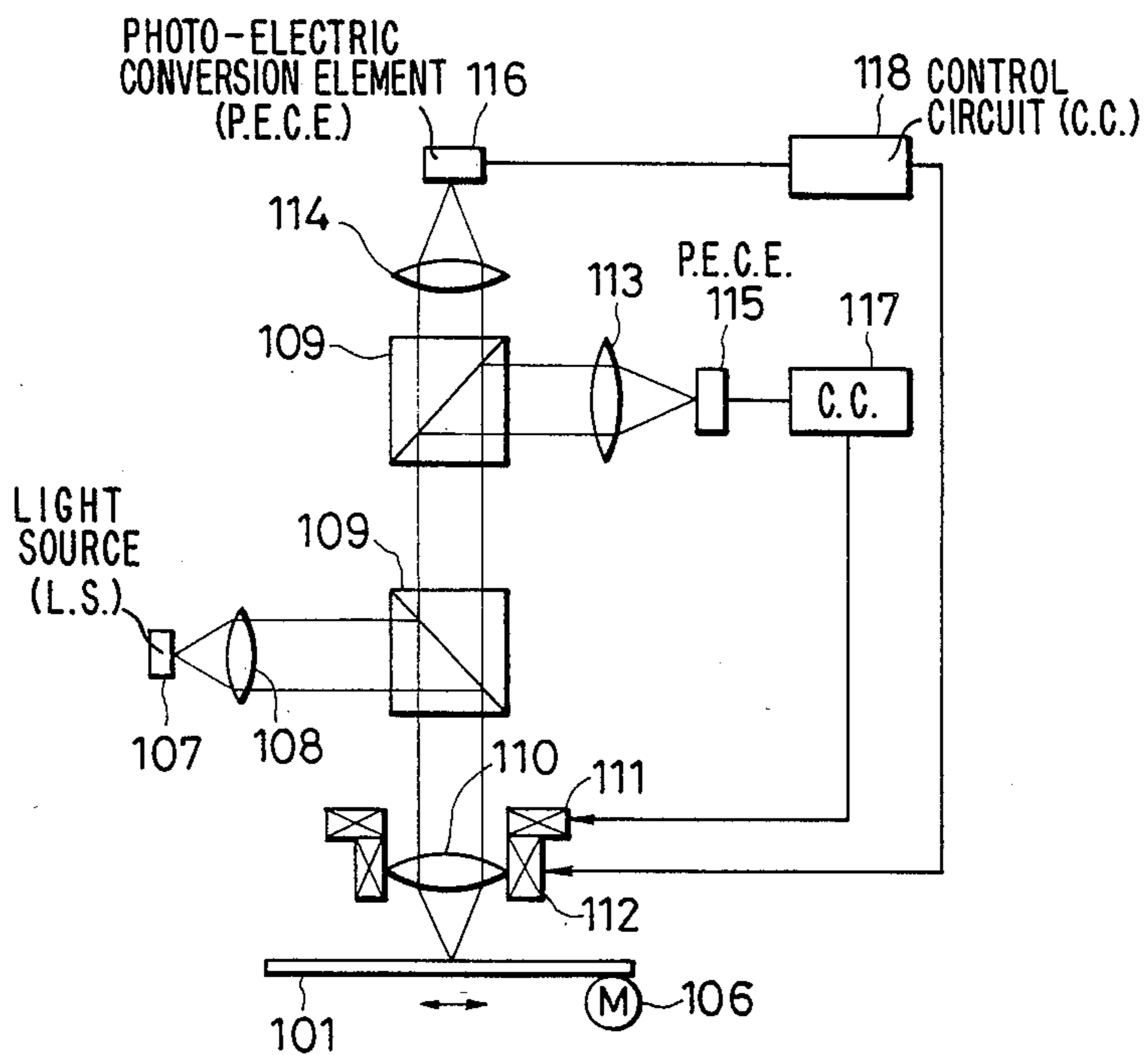
FIG. 2 PRIOR ART
