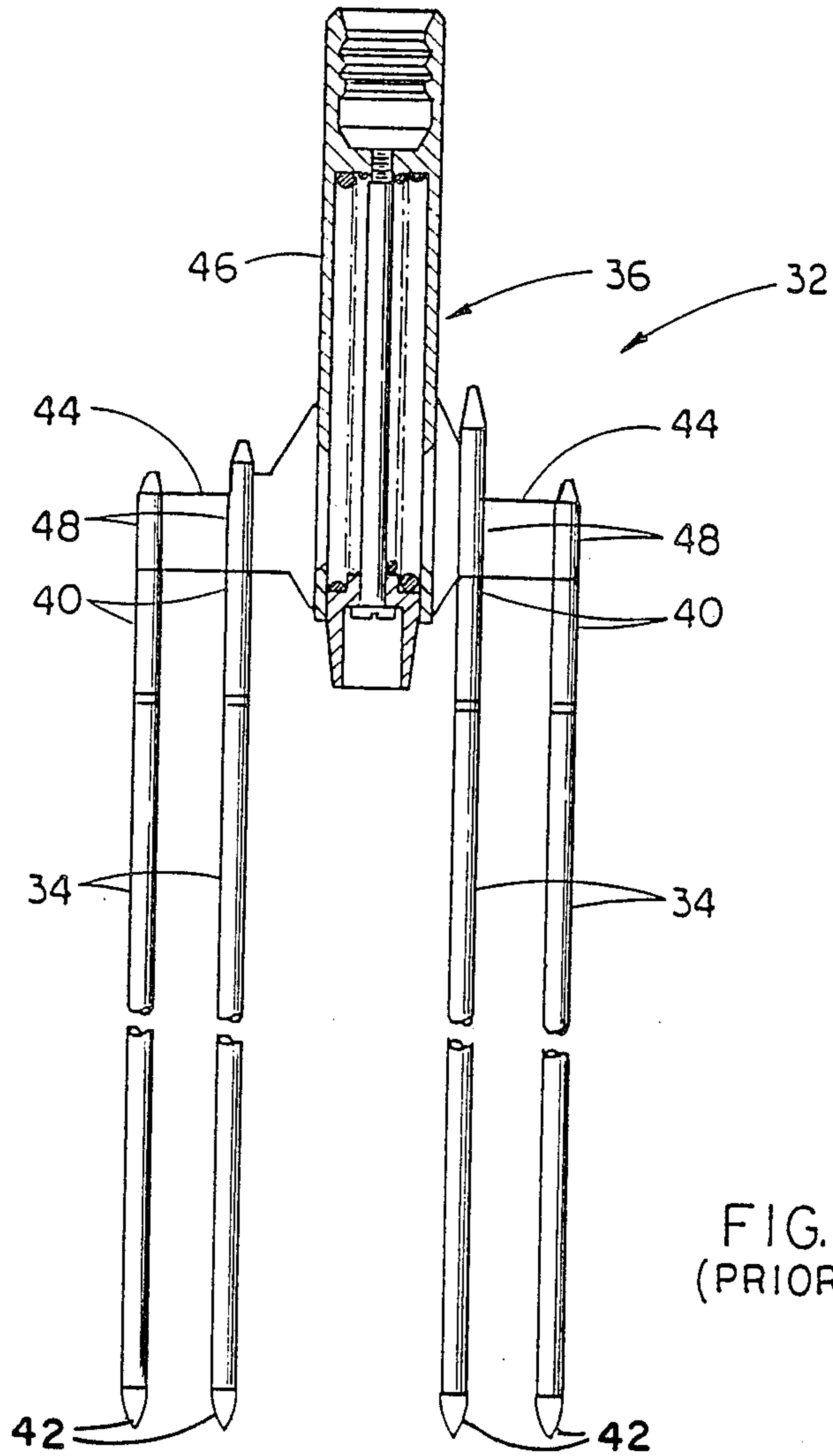
FIG. 2 (PRIOR ART)
