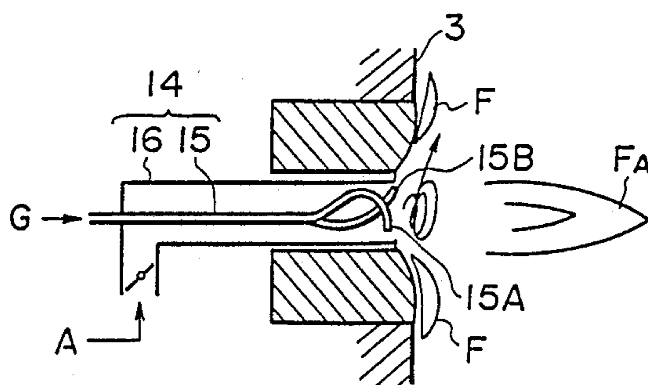
FIG-11 (PRIOR ART)
