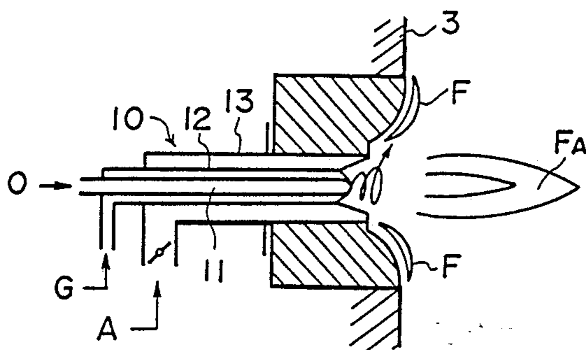
FIG-10 (PRIOR ART)
