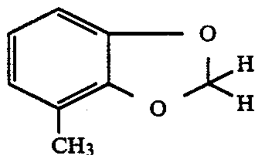
(a) 4-Methyl-1,3-benzodioxole
