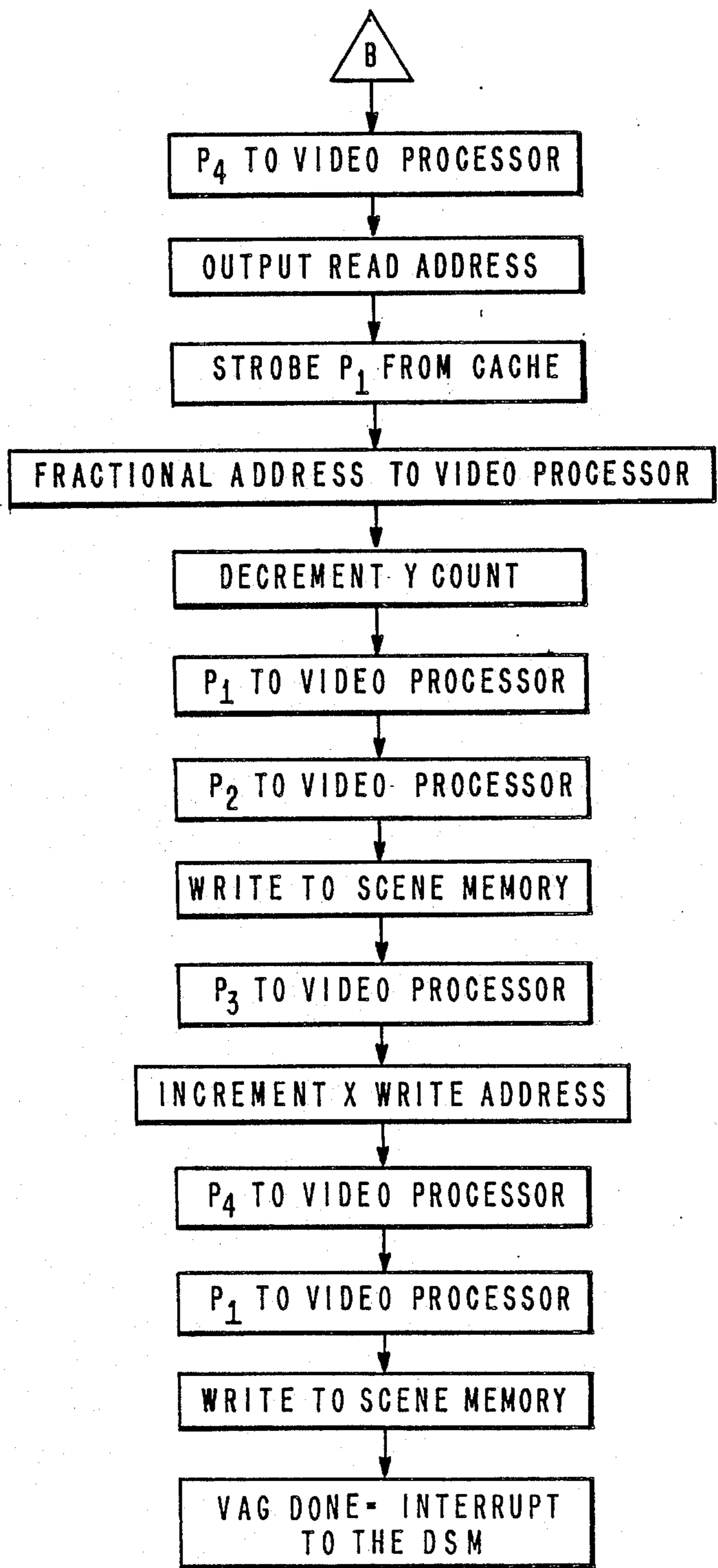
VAG CONTROL FLOW BILINEAR INTERPOLATION MODE
