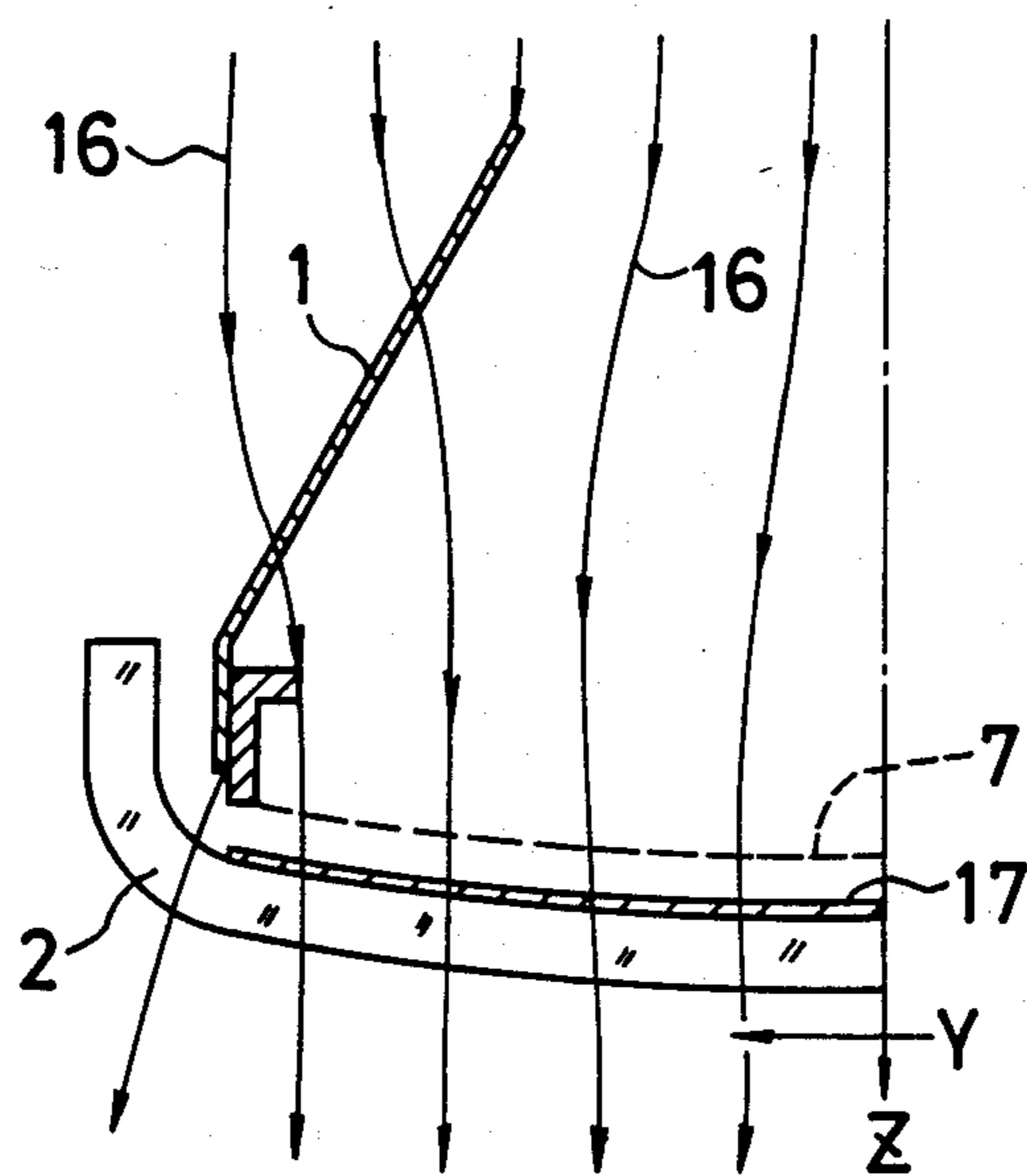
FIG. 6 (PRIOR ART)
