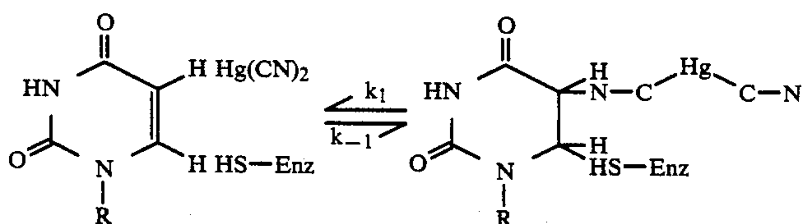
(cl UMP) R = DE OXy RiBOSE
