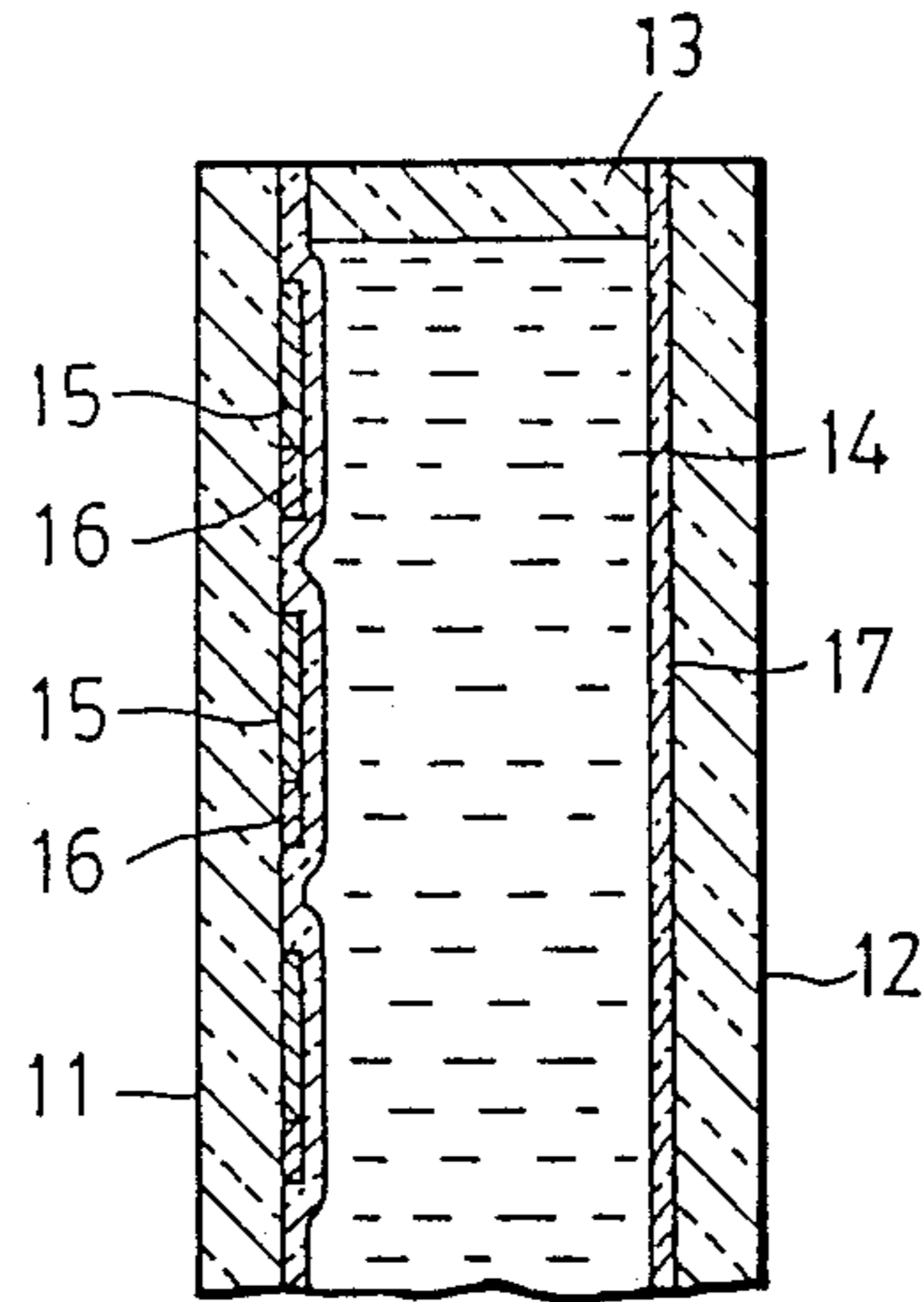
FIG. 1 PRIOR ART
