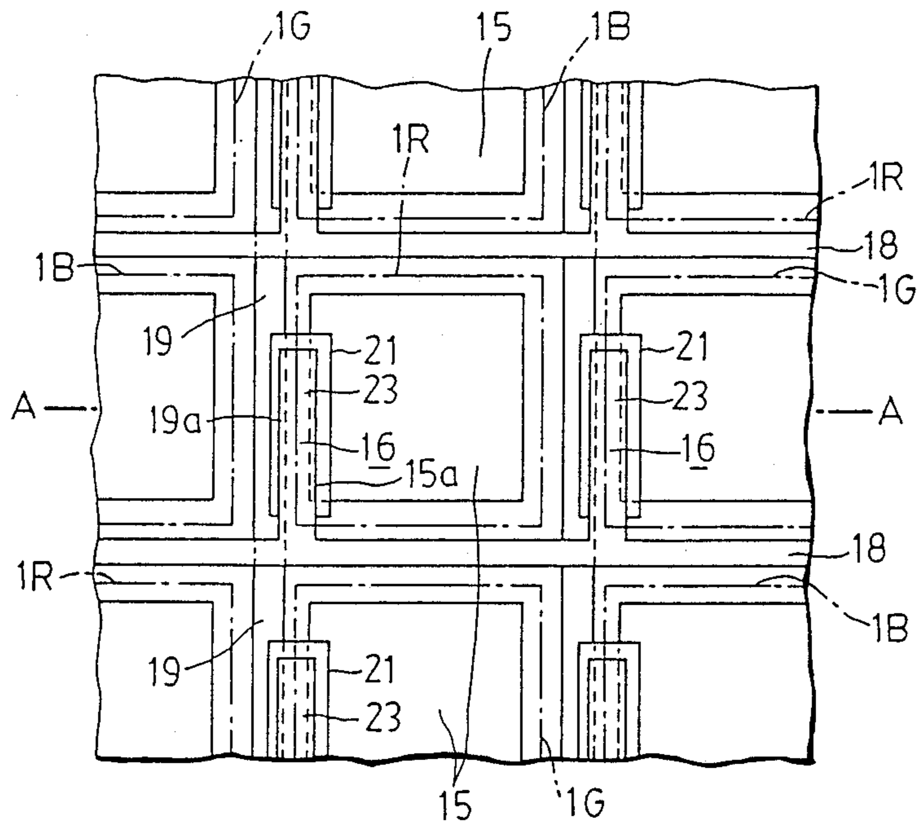
FIG. 3 PRIOR ART
