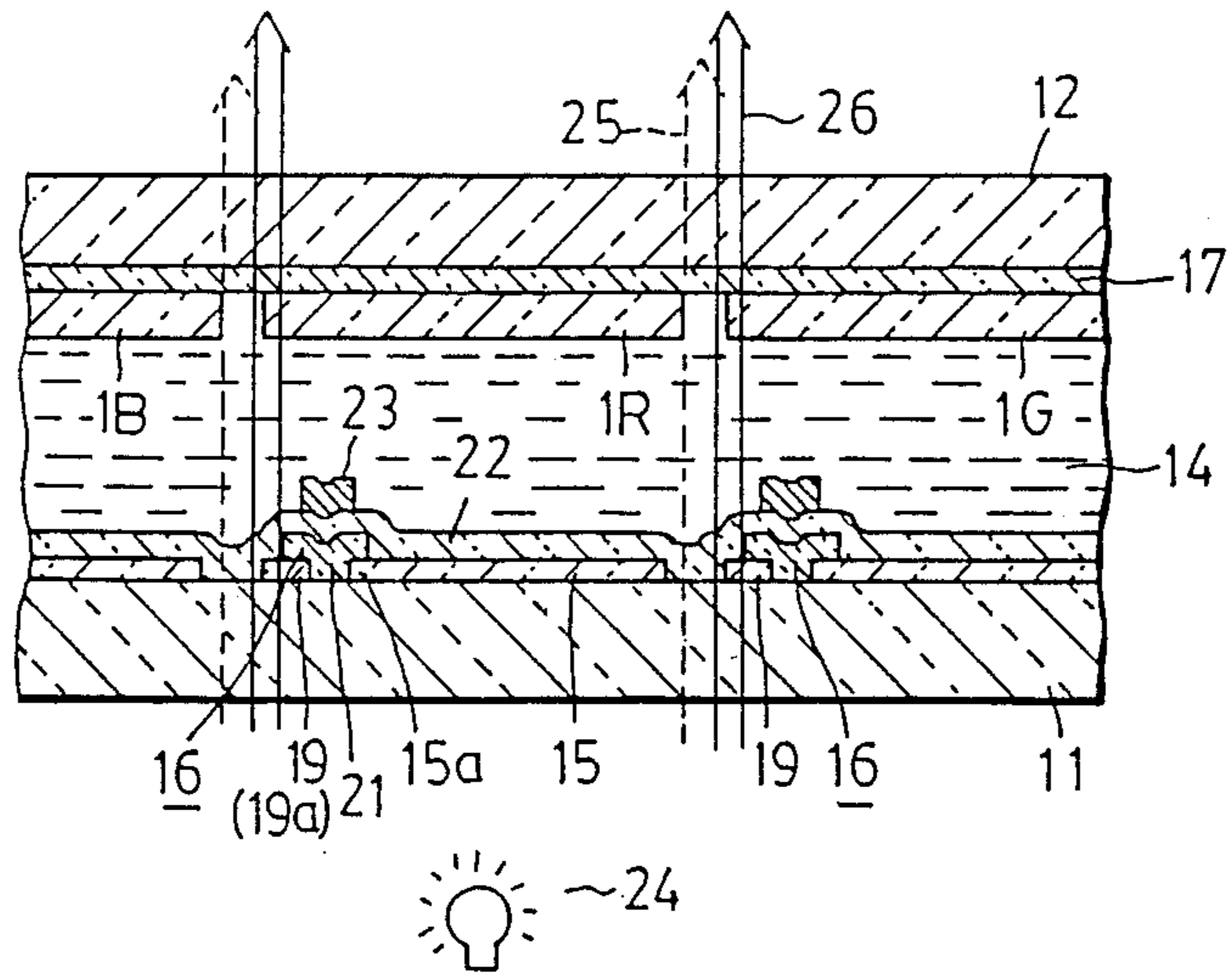
FIG. 4 PRIOR ART
