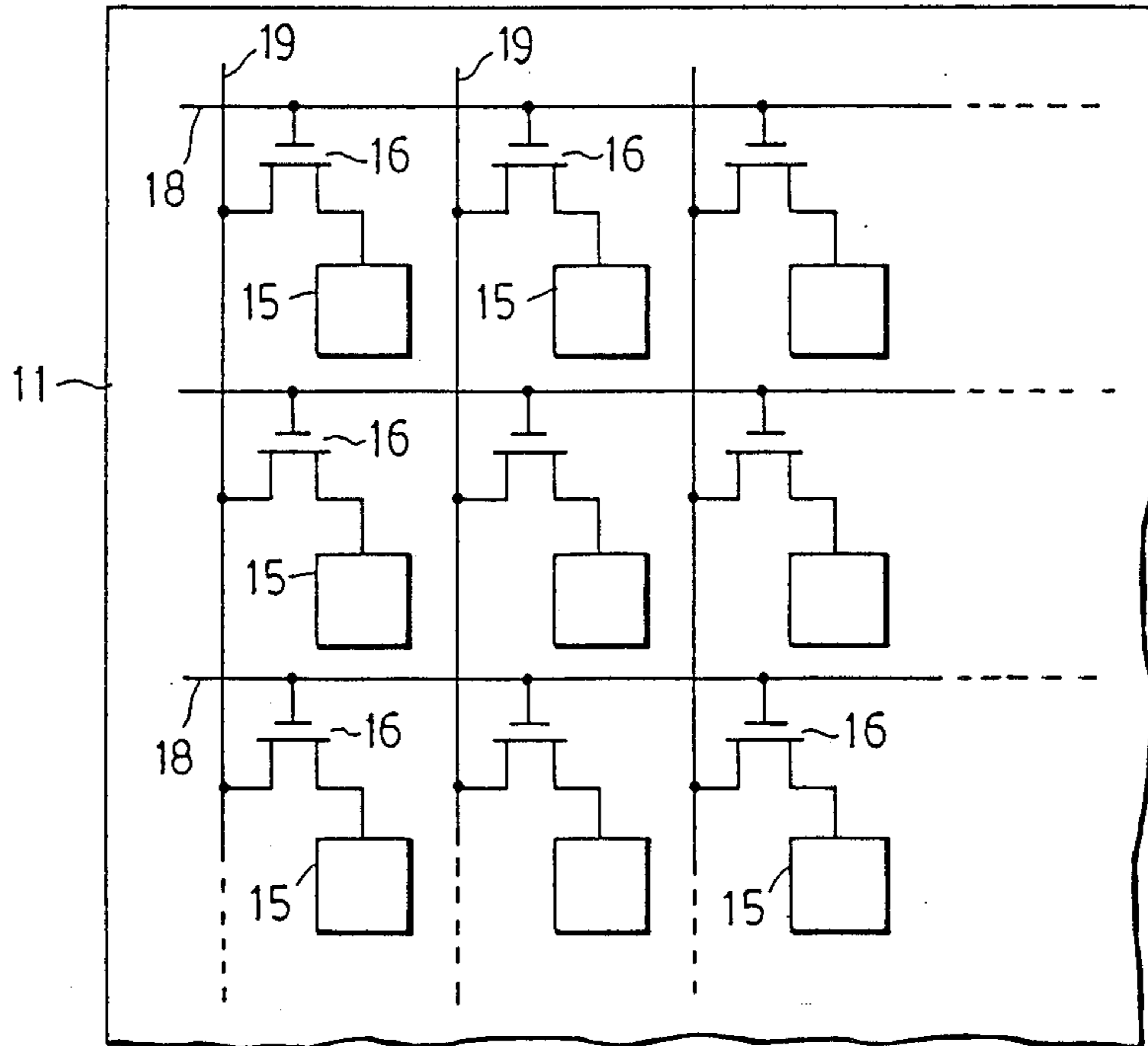
FIG. 2 PRIOR ART
