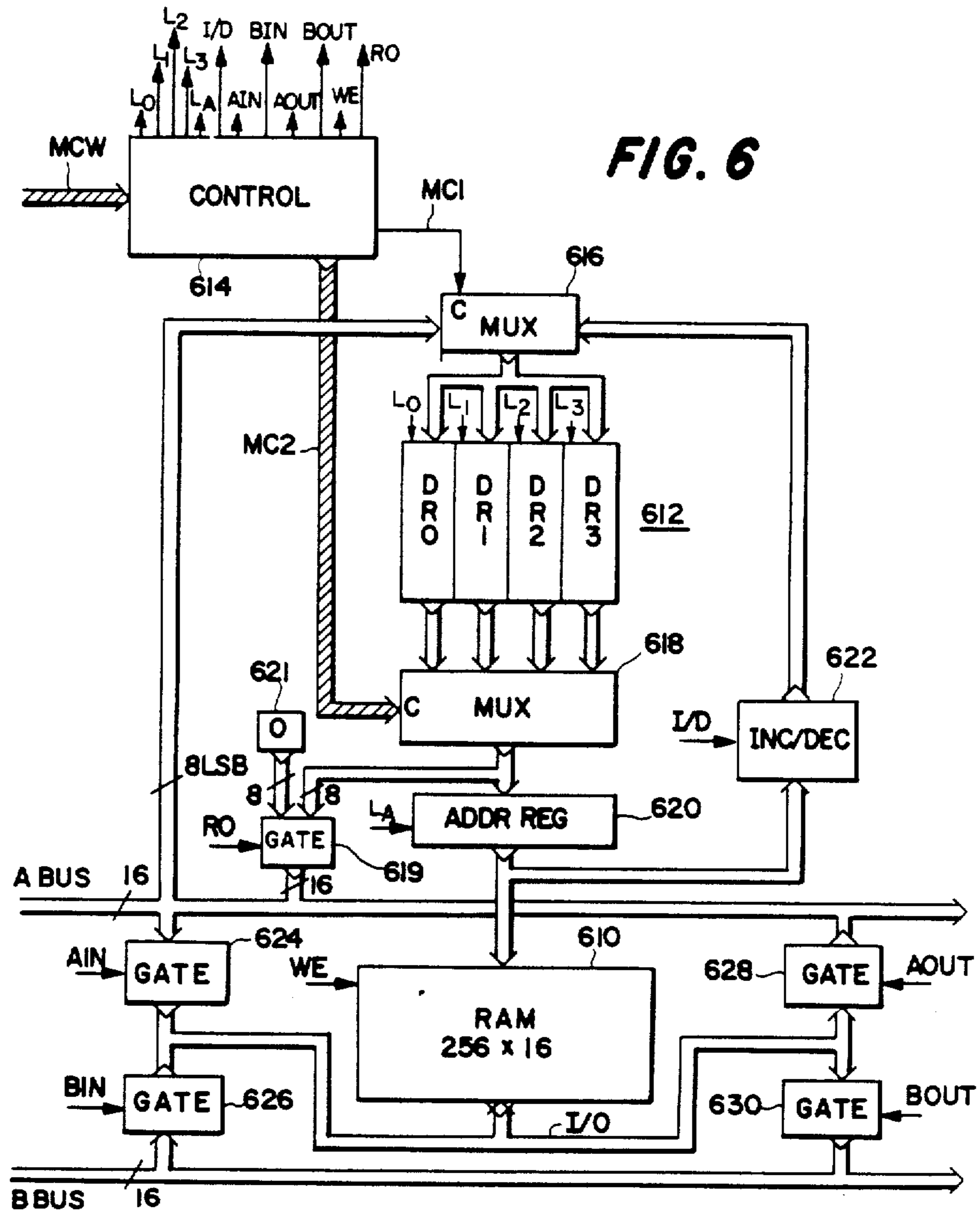
DATA RAM
