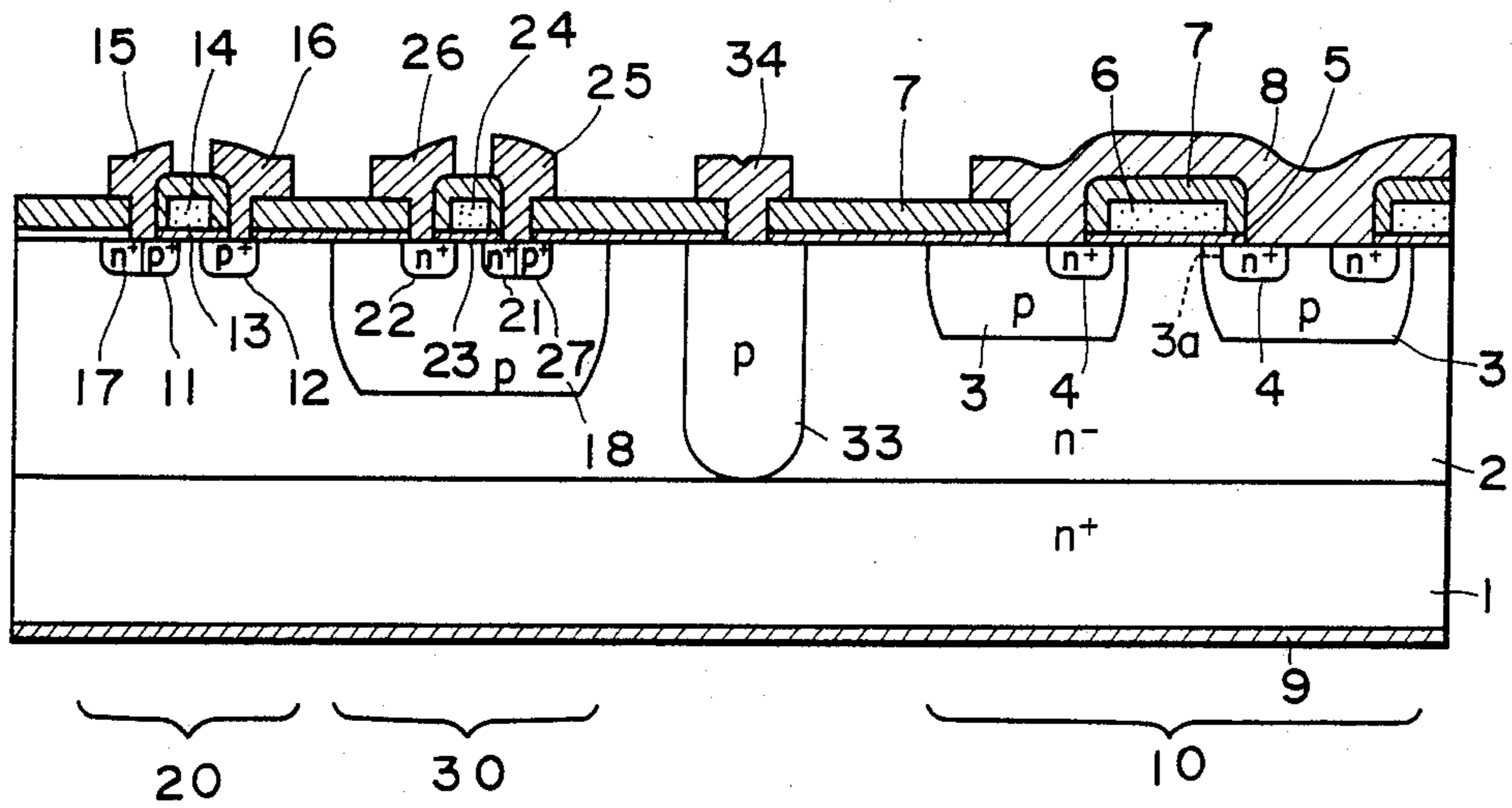
FIG. 9 (PRIOR ART)
