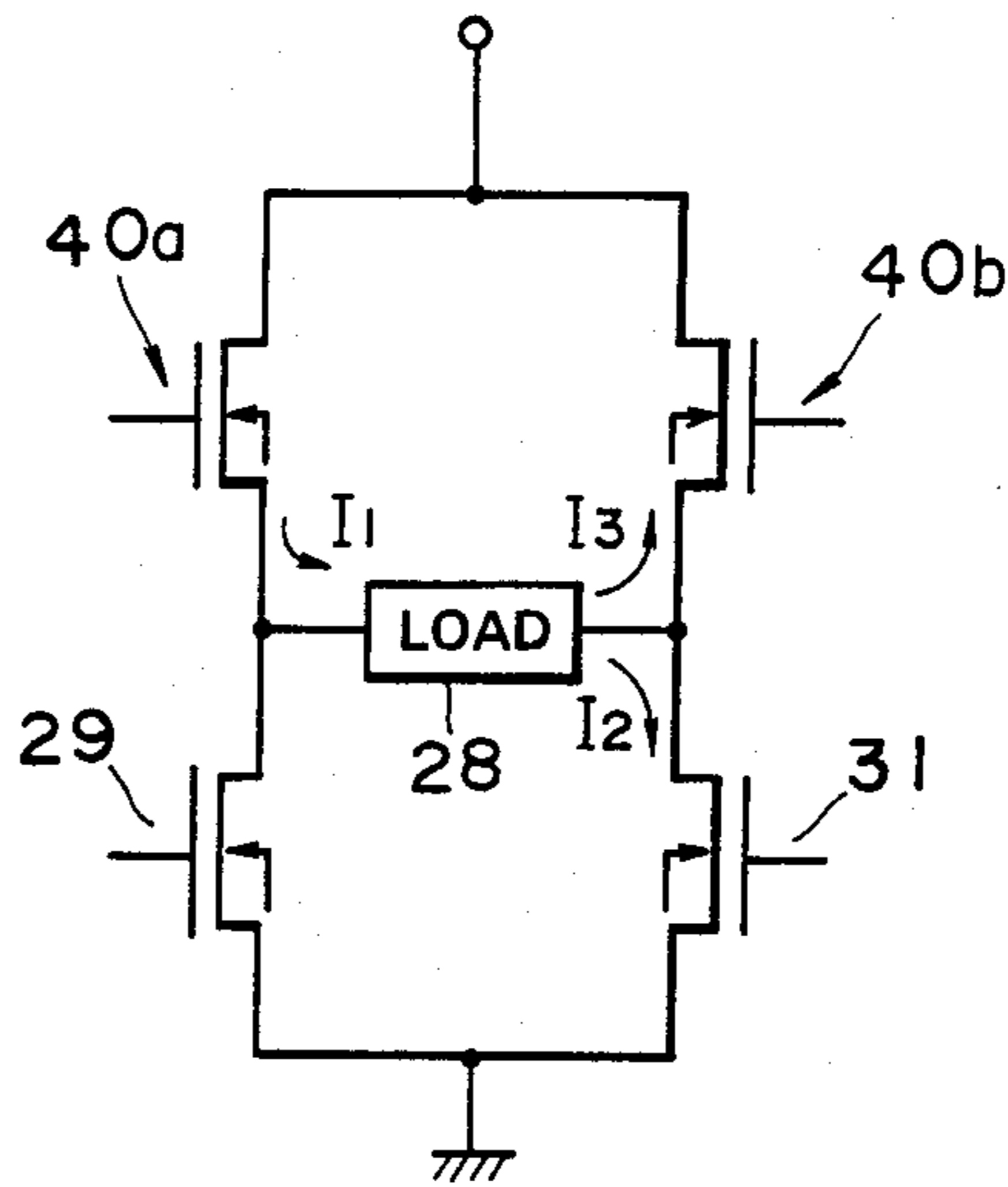
FIG. 8 (PRIOR ART)
