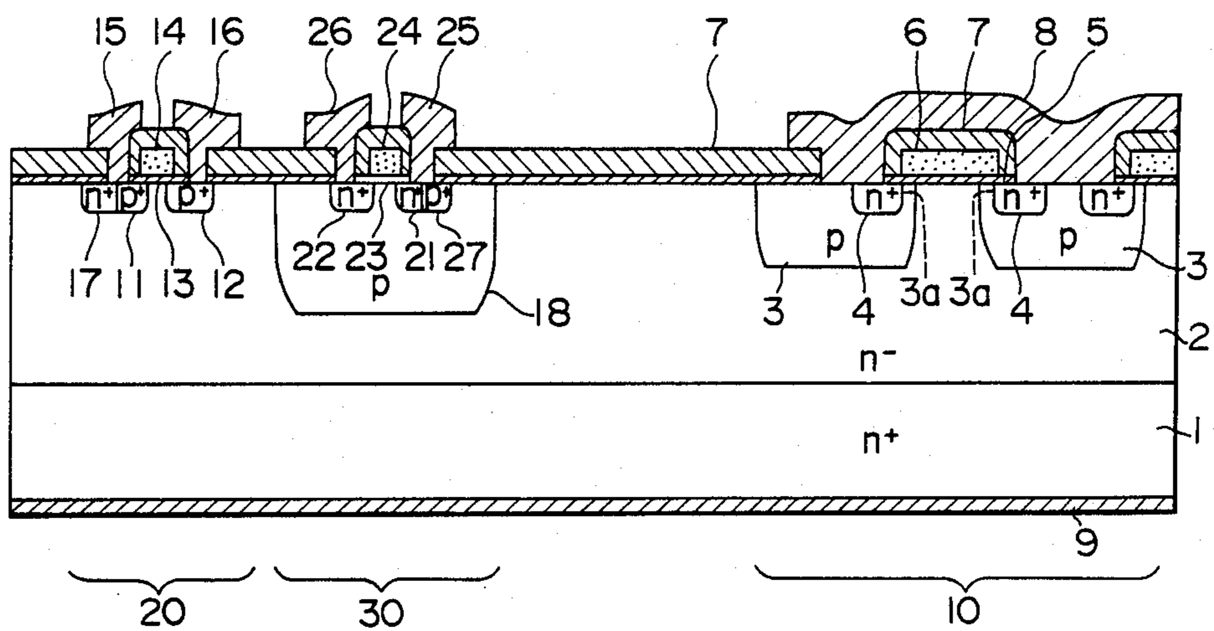
FIG. 6 (PRIOR ART)
