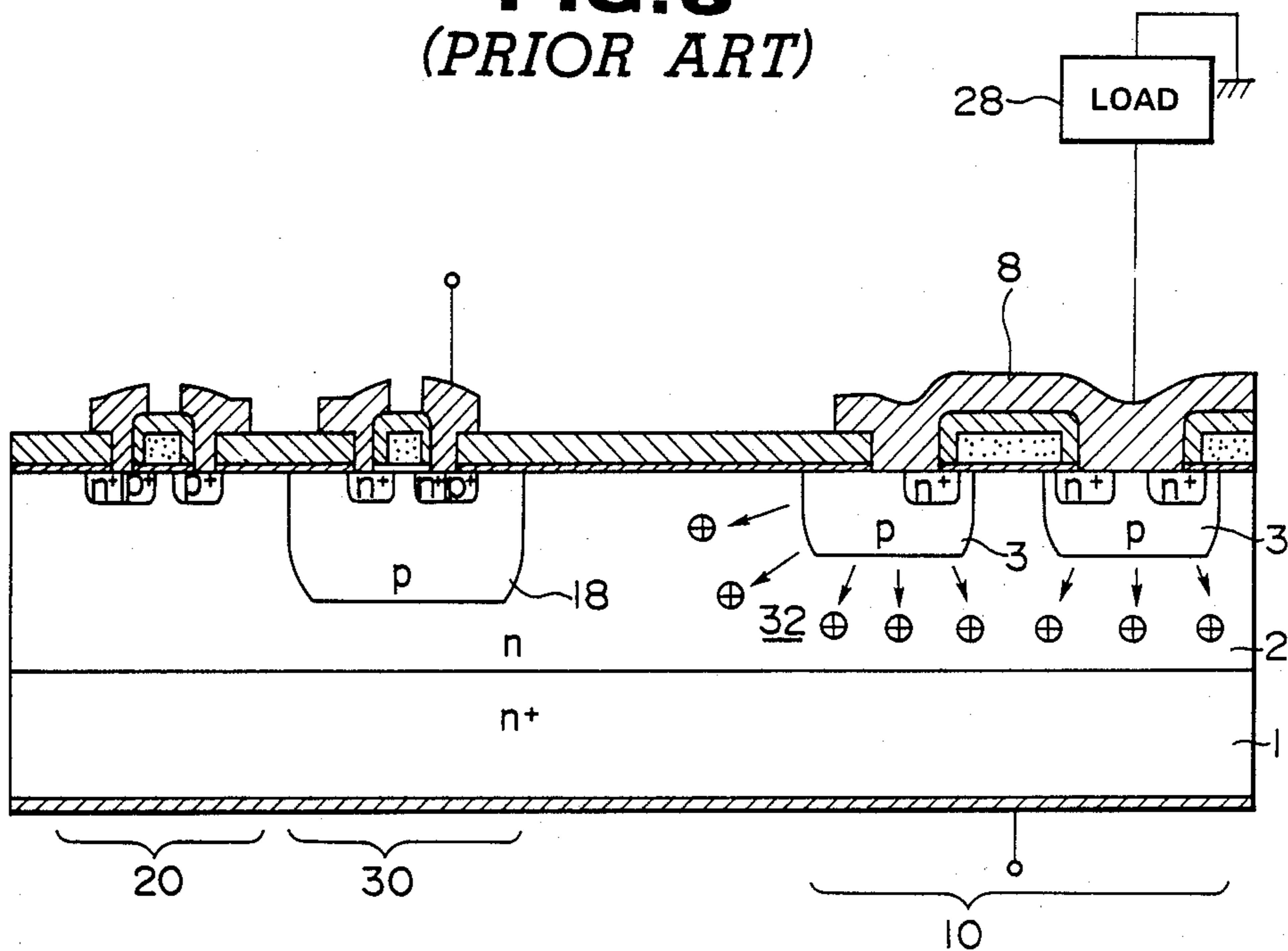
FIG. 7 (PRIOR ART)
