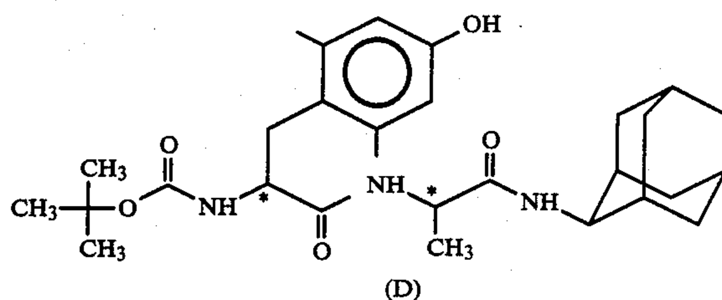
(Boc-2,6Me 2 Tyr-(D)Ala-NH 2 Ad)
