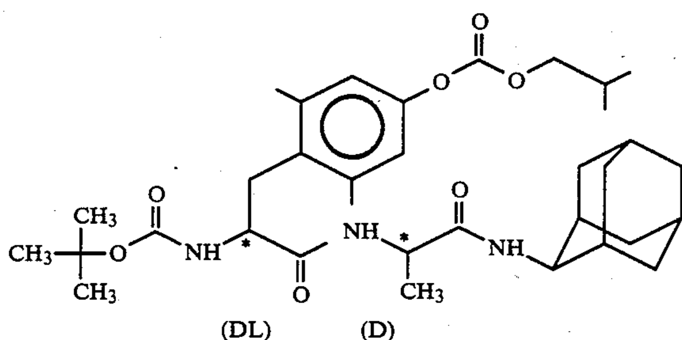
(Boc-(DL)2,6Me 2 Tyr(IBC)-(D)Ala-NH 2 Ad)
