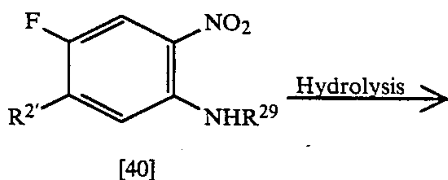
[Reaction scheme-XI]
