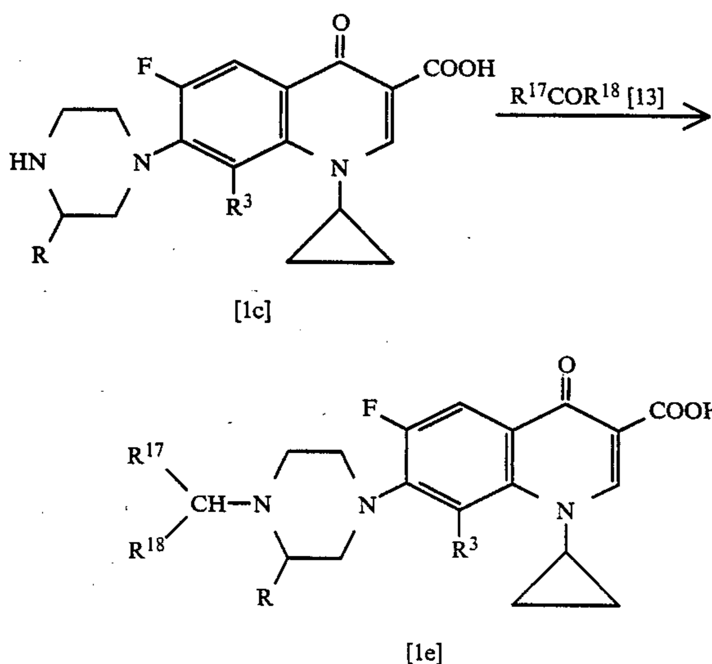
[Reaction scheme-IV]
