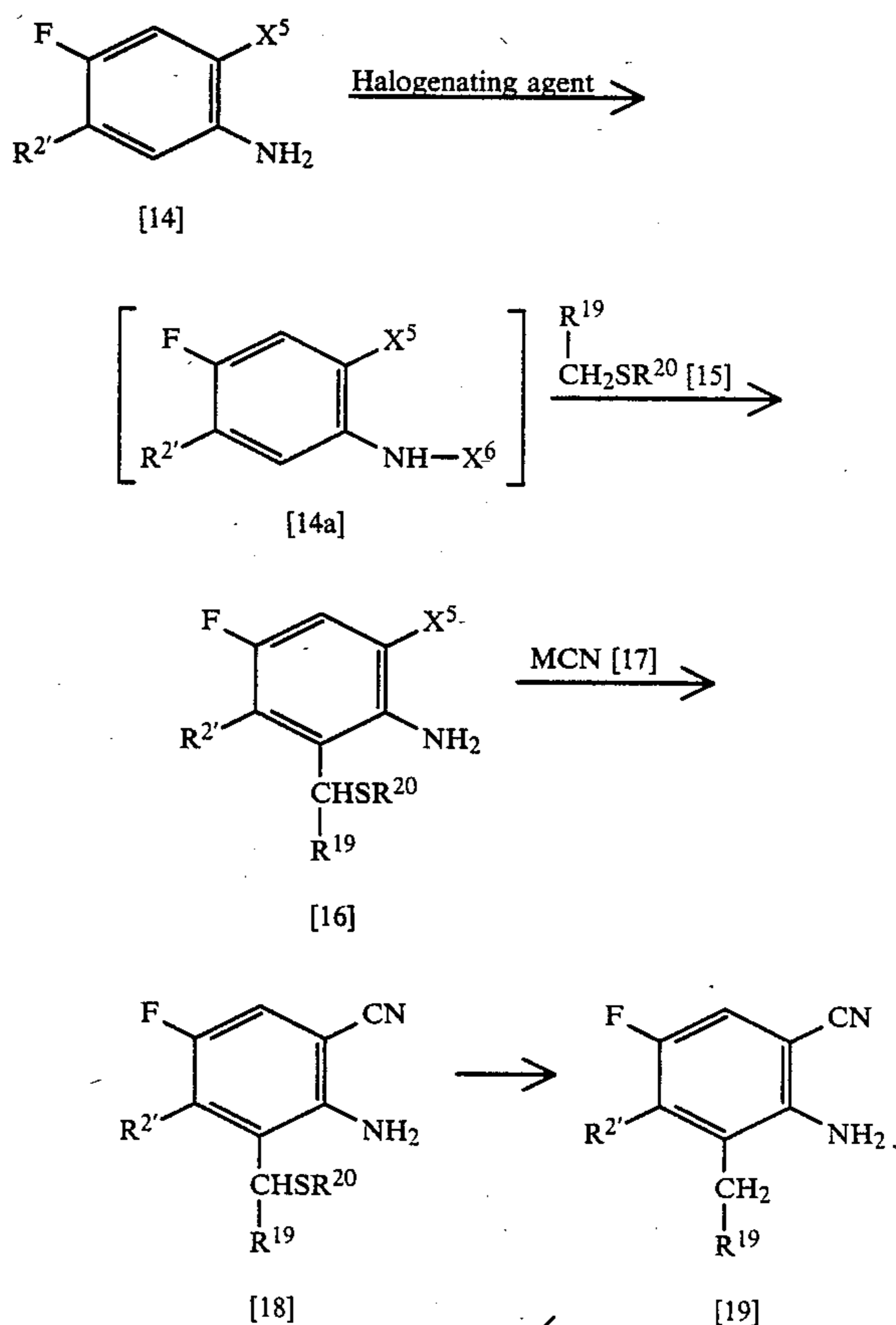
[Reaction scheme-V]
