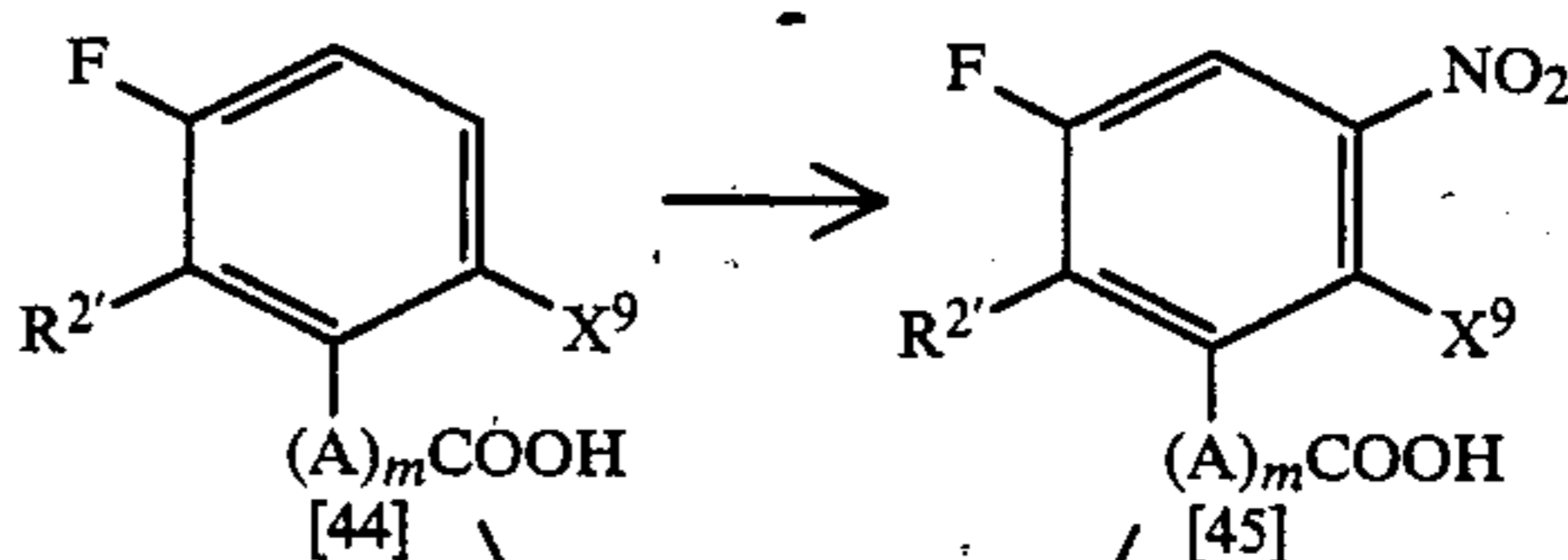
[Reaction scheme-XII]
