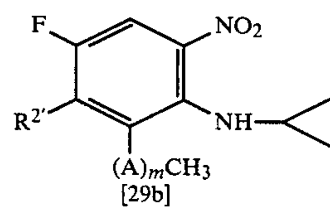
[Reaction scheme-XIII]
