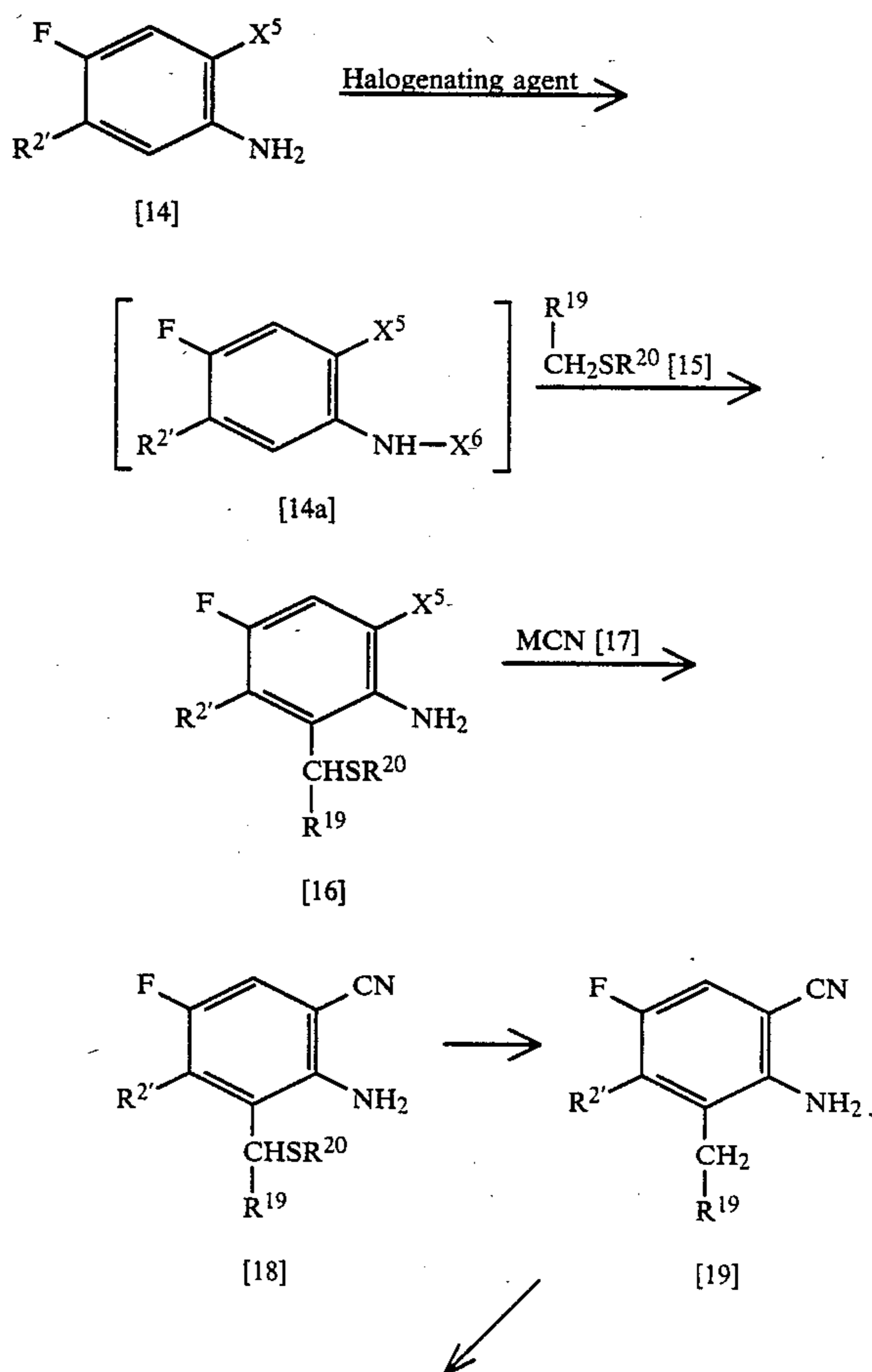
[Reaction scheme-V]
