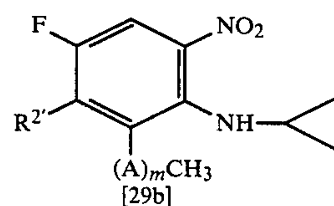
[Reaction scheme-XIII]
