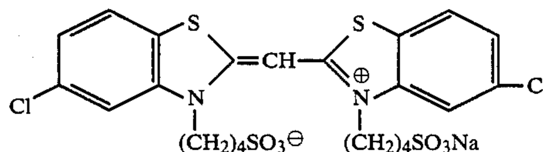
Sensitizing Dye for Blue-Sensitive Layer:
