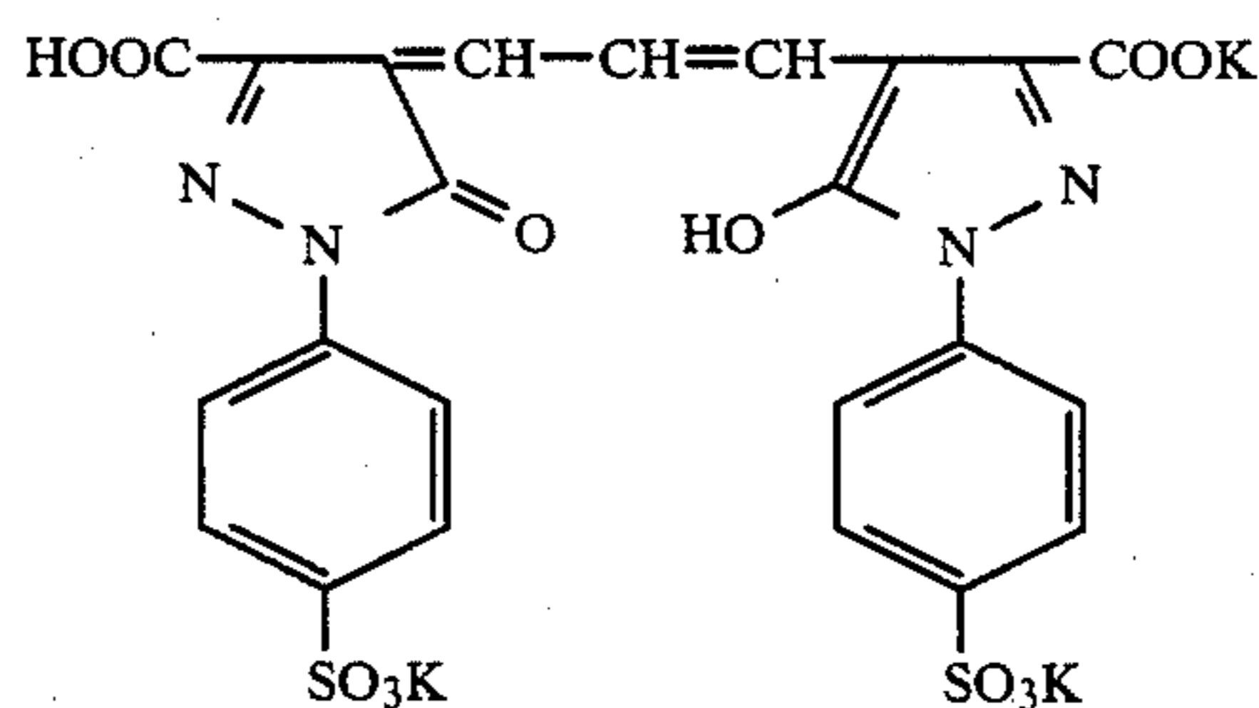
Anti-Irradiation Dye for Green-Sensitive Layer:
