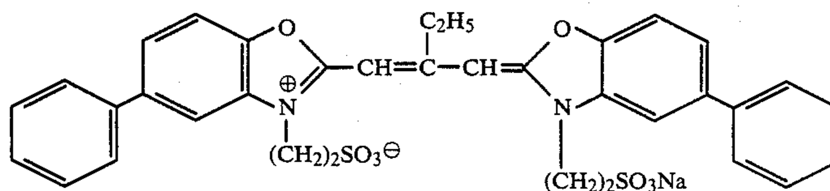
Sensitizing Dye for Green-Sensitizing Layer:
