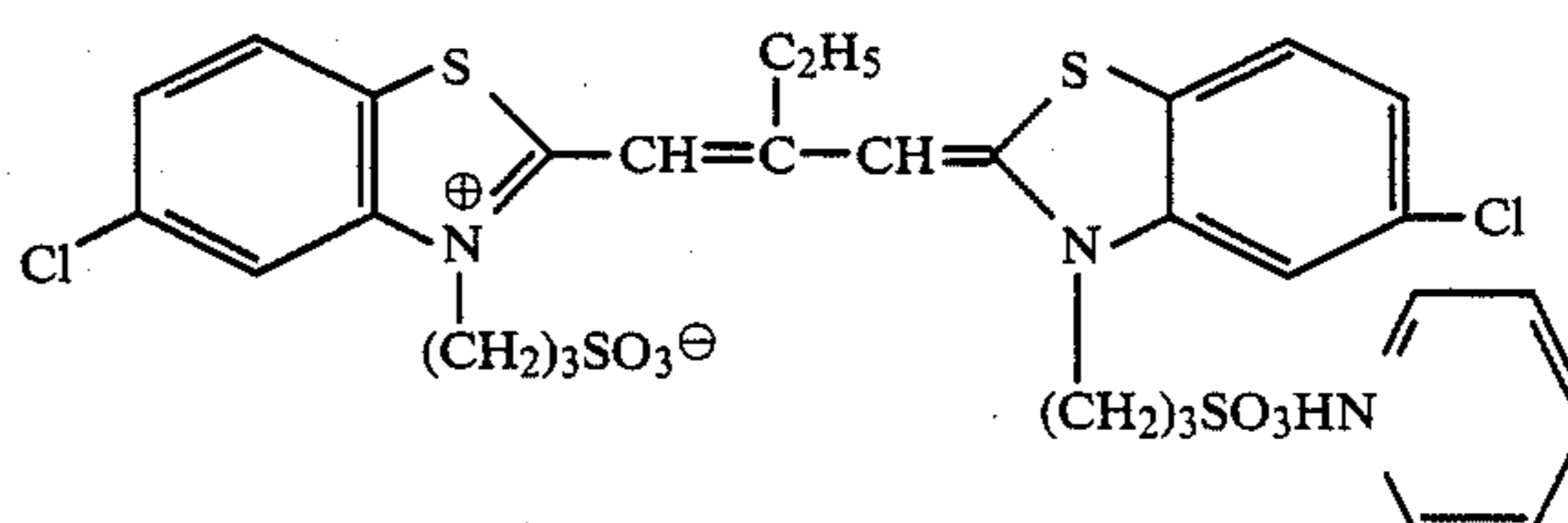
Sensitizing Dye for Red-Sensitive Layer:
