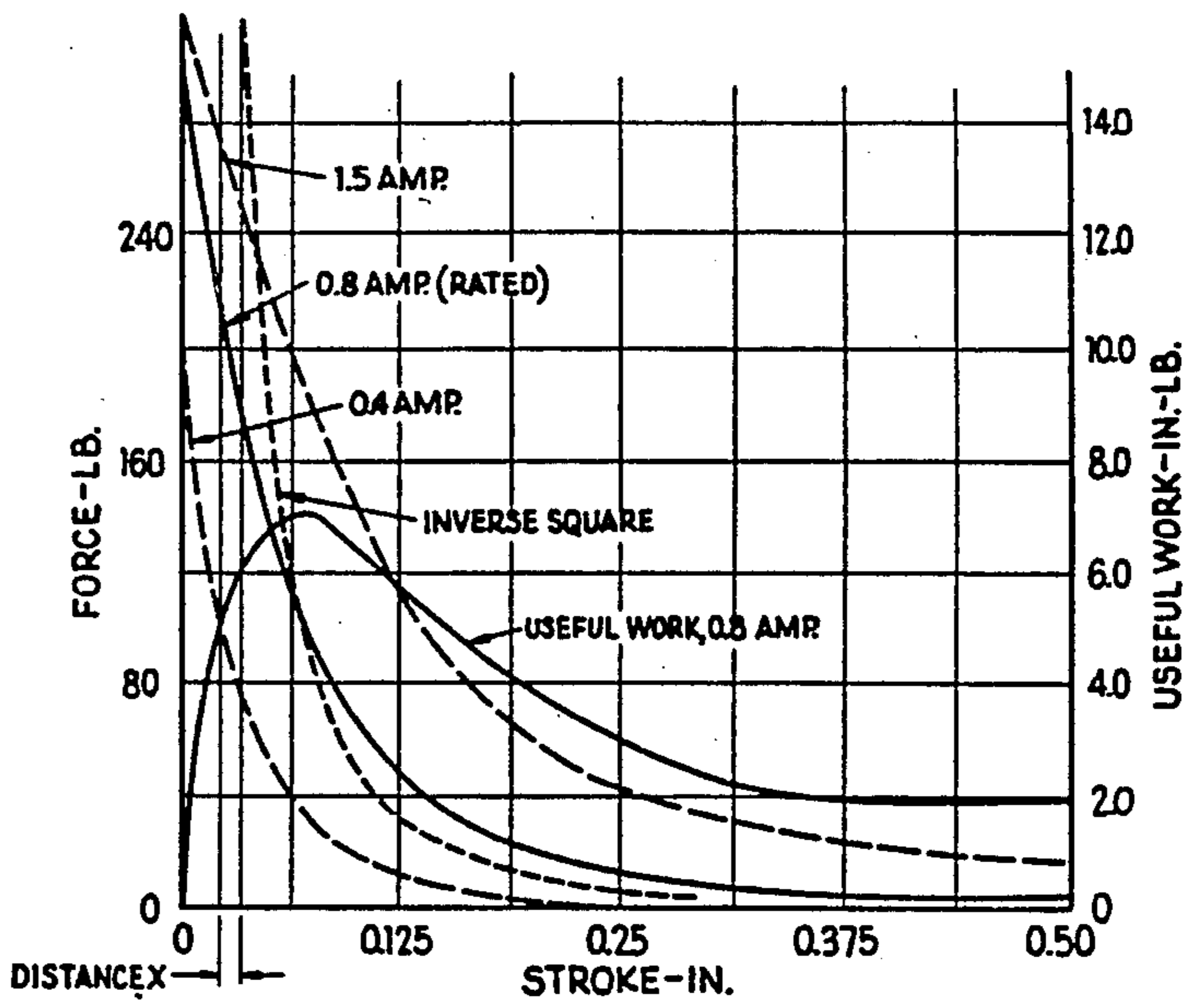
FLAT-FACED PLUNGER MAGNET AND ITS FORCE-STROKE CURVES
