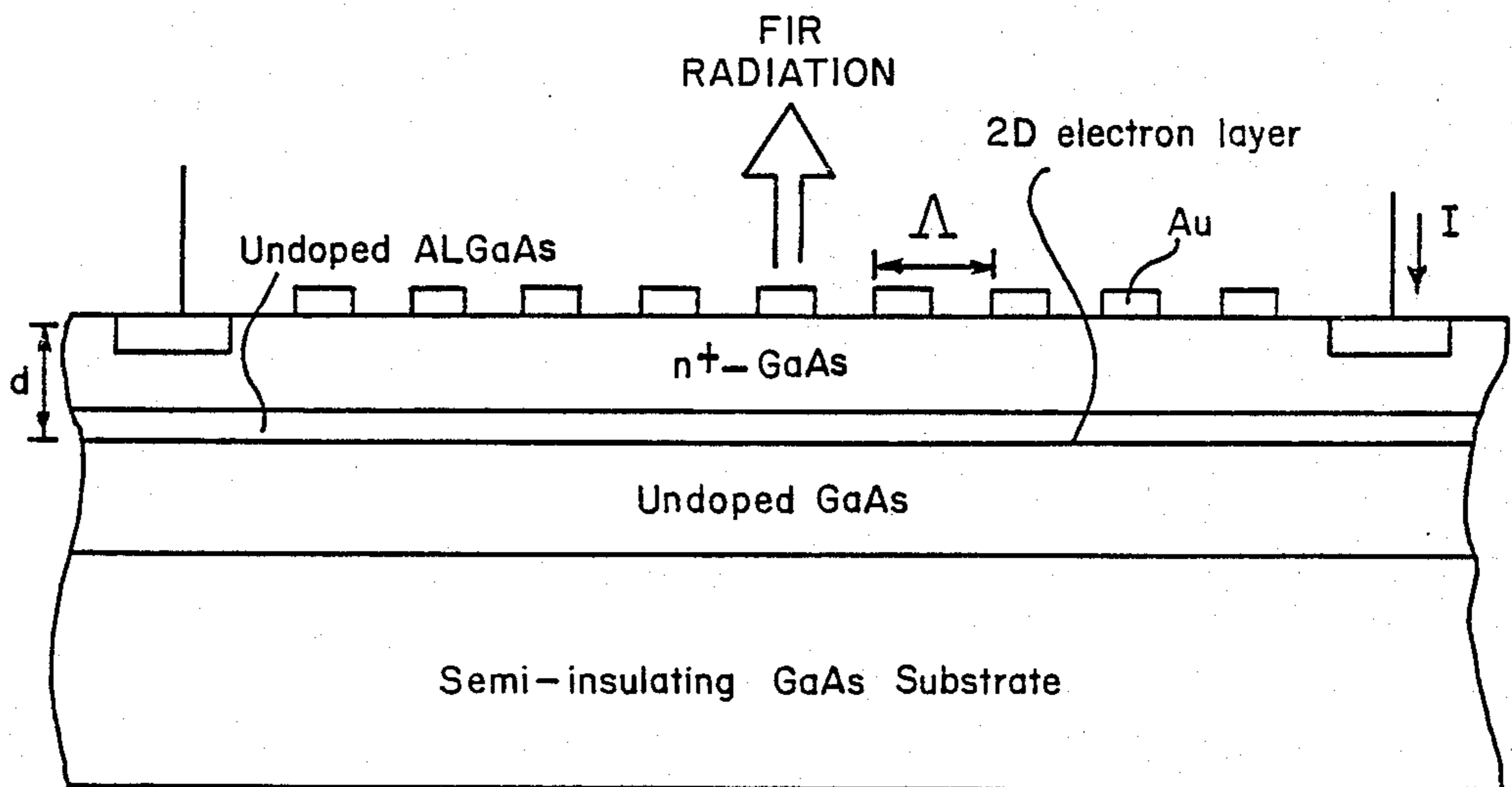
FIG. 2 (PRIOR ART)
