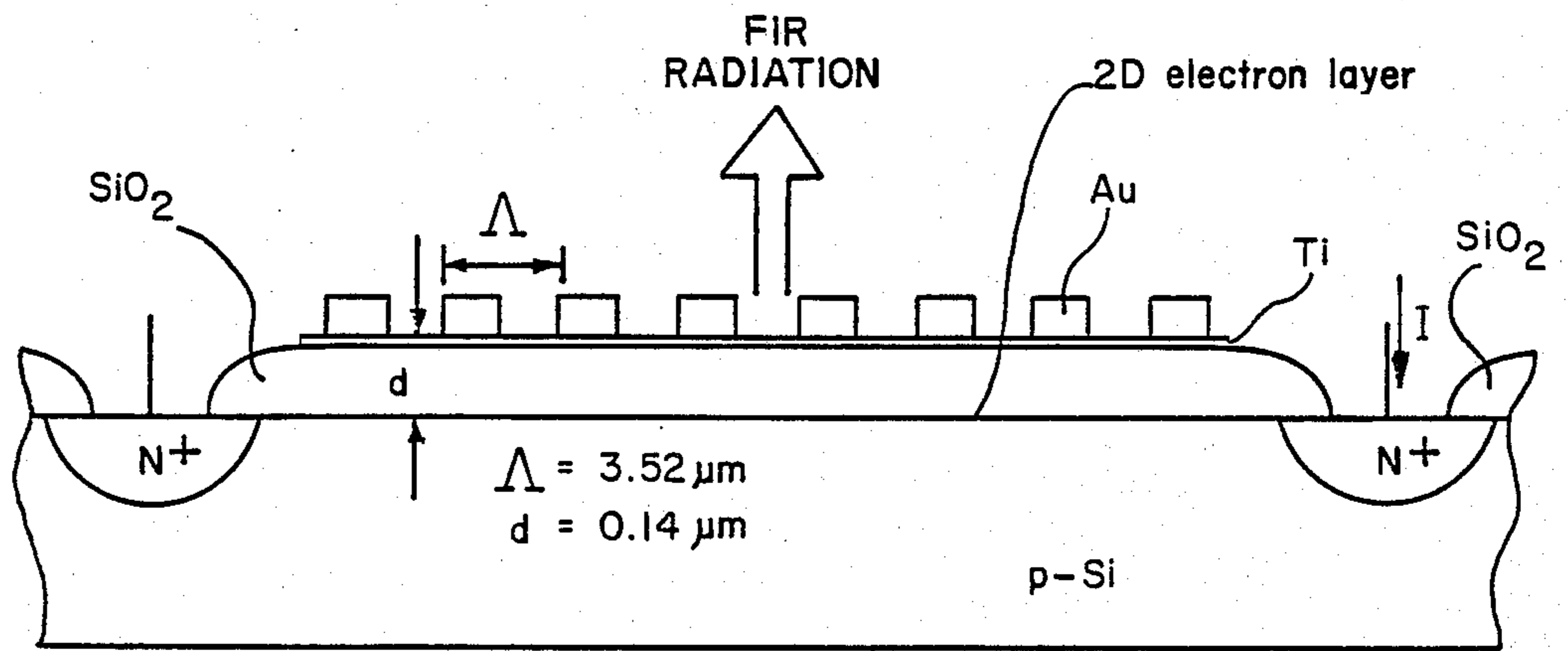
FIG. 1 (PRIOR ART)
