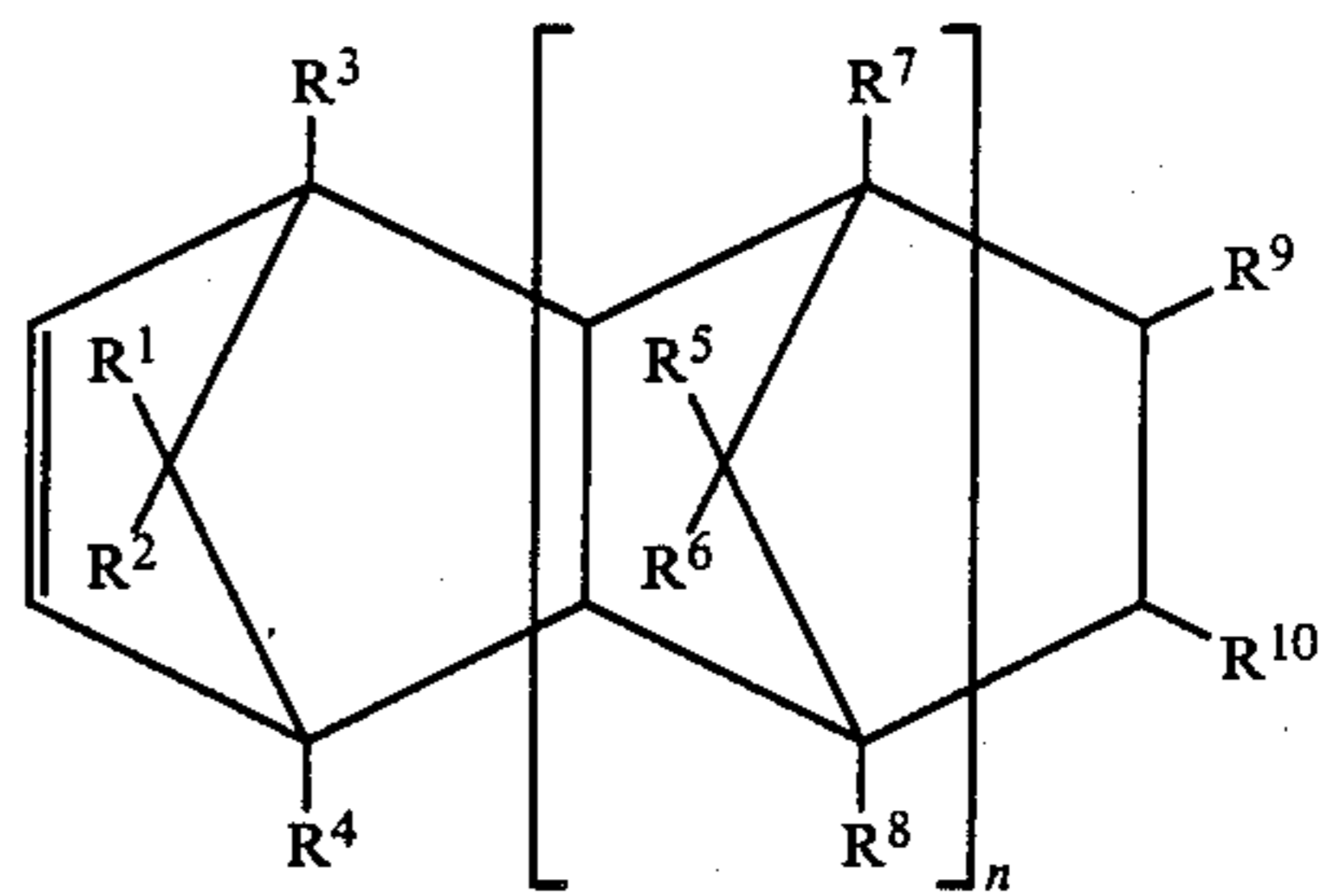
General formula
