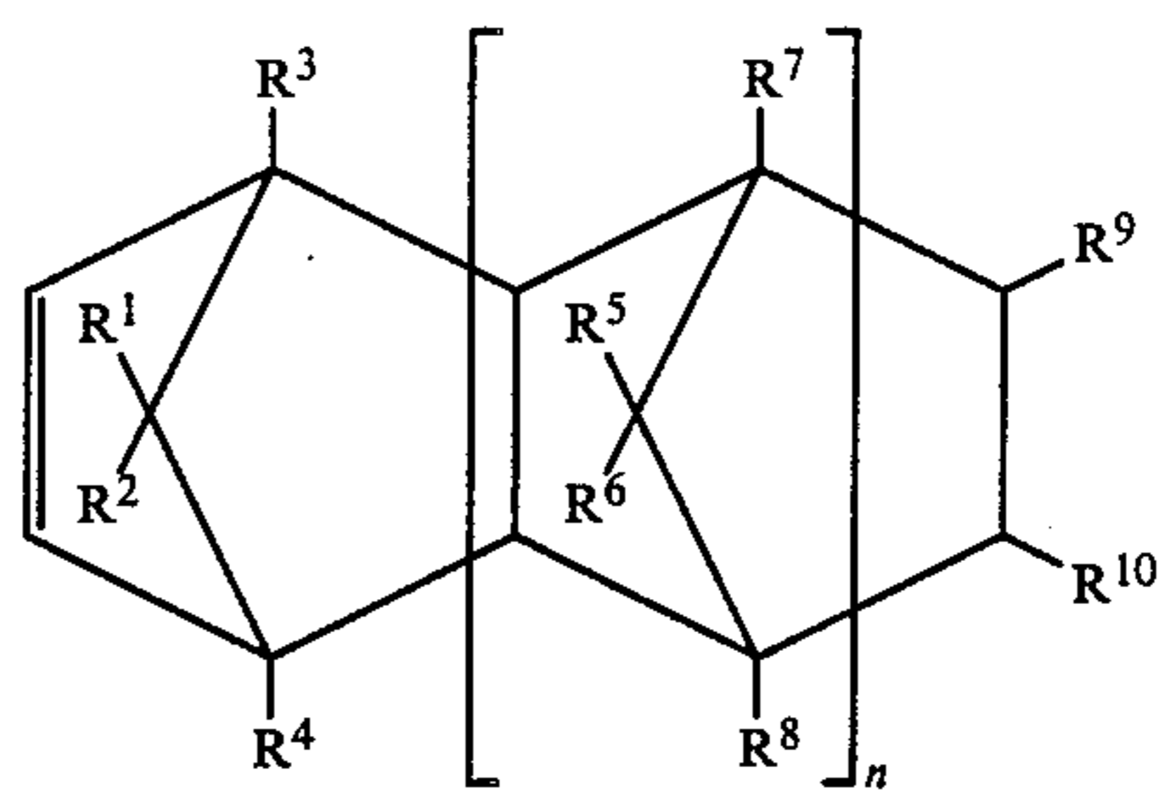
General formula
