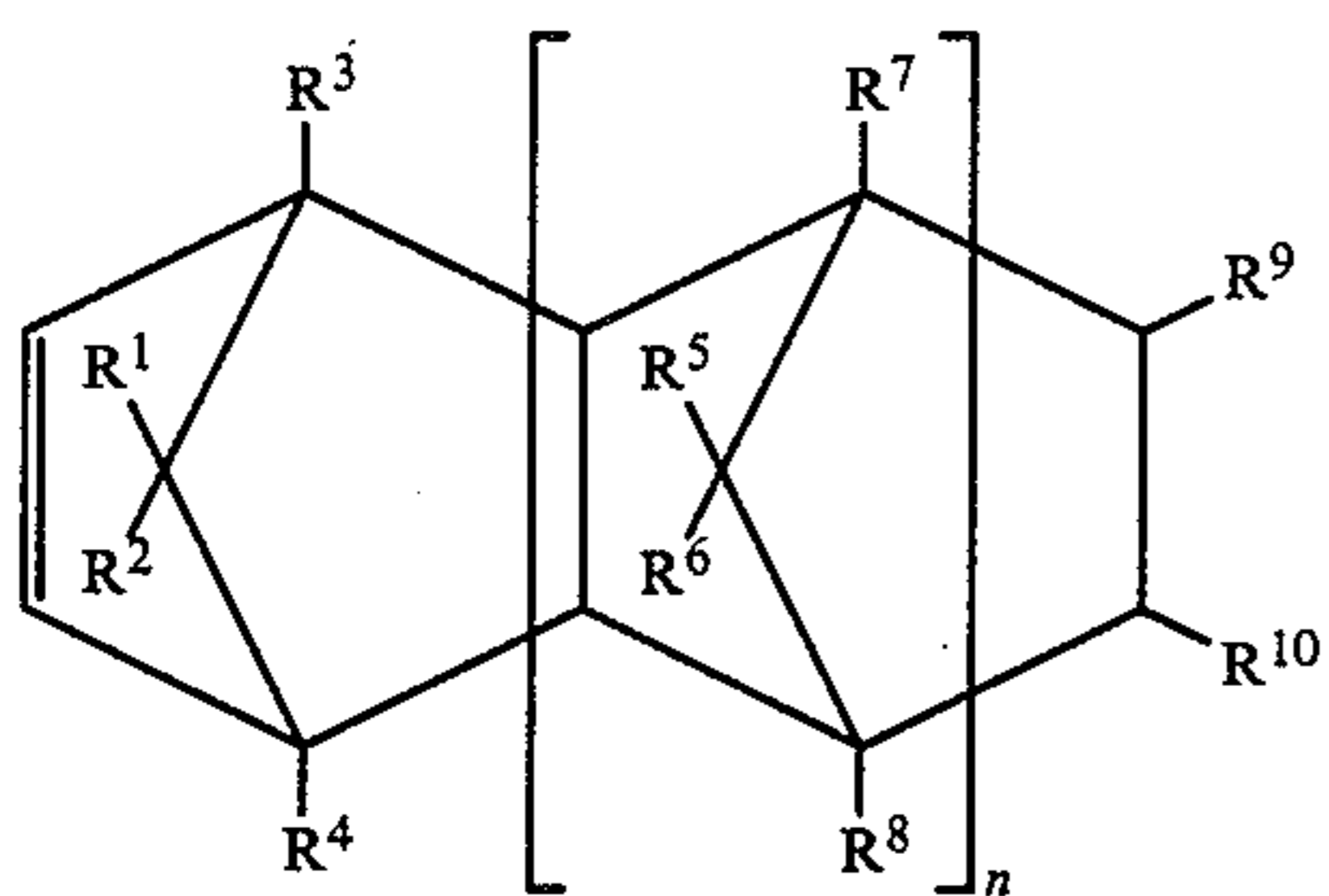
General formula
