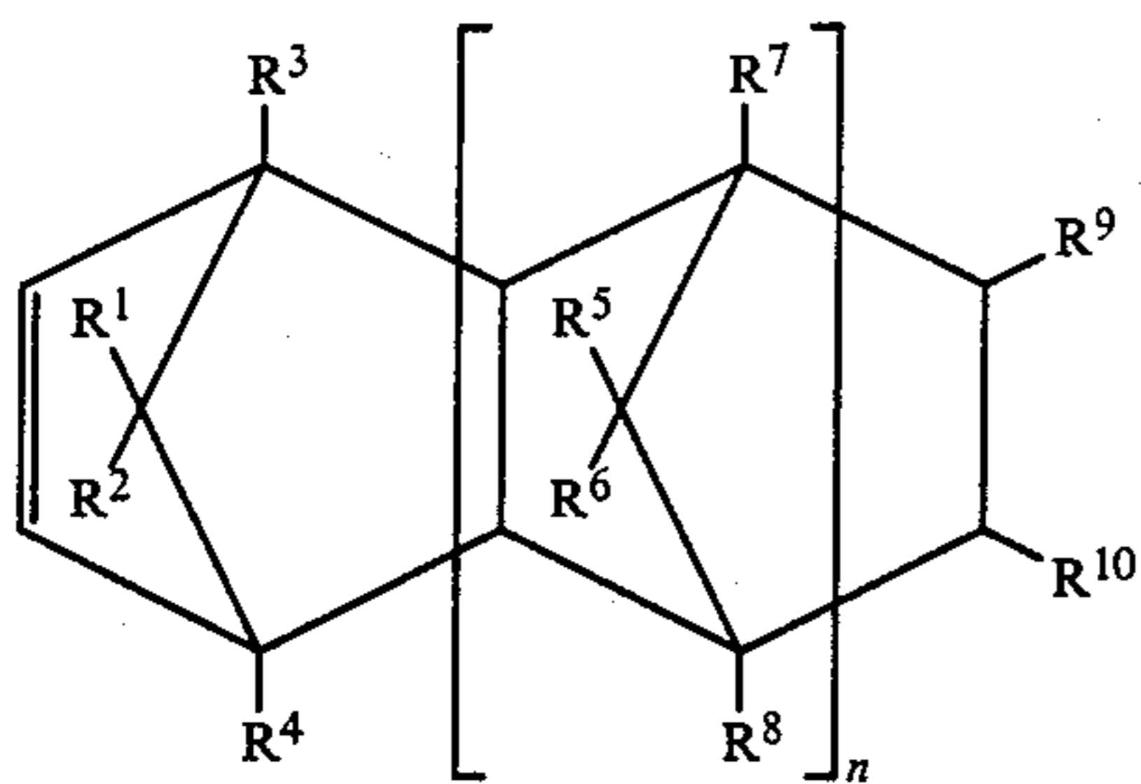
General formula
