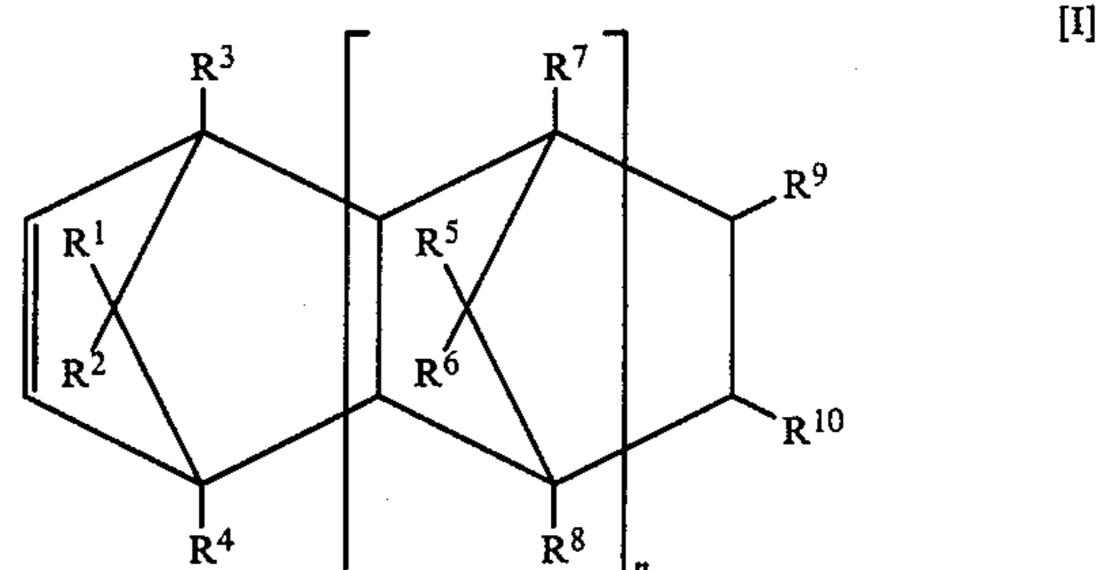
General formula
