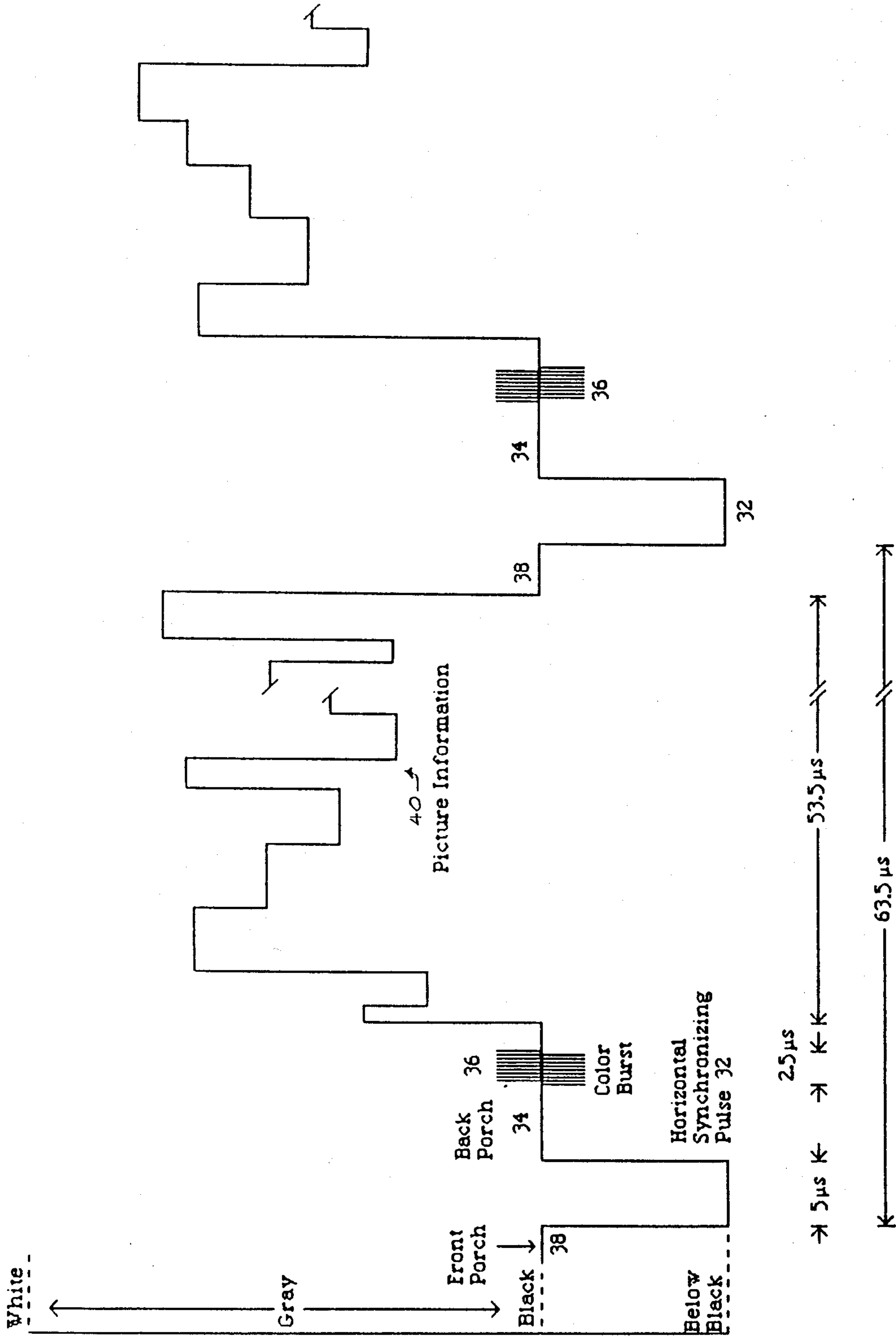
FIGURE 2 Composite Television Picture Signal (not to time scale)
