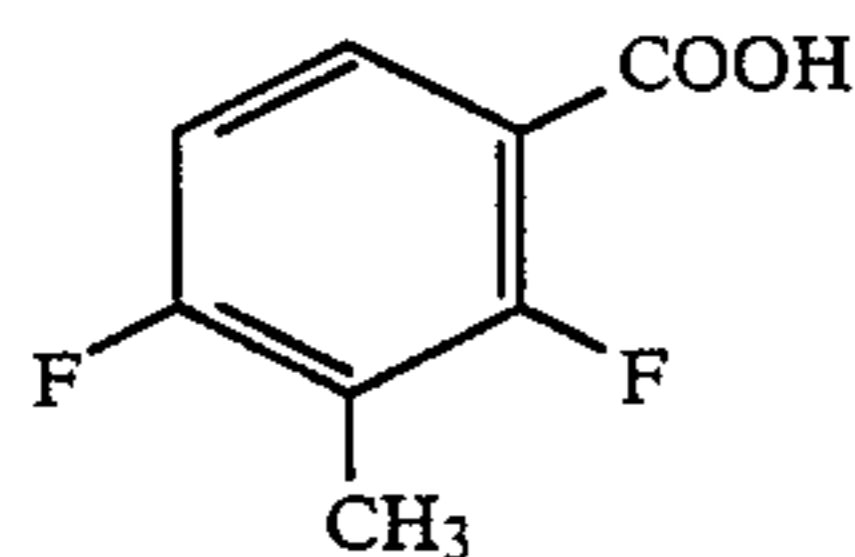
2,4-difluoro-3-methylbenzoic acid
