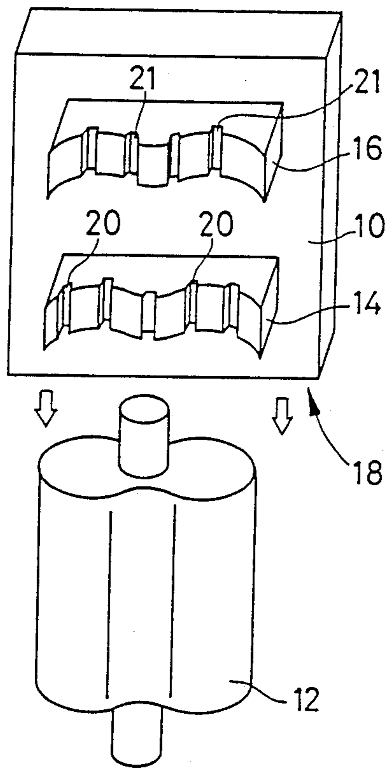
FIG. 14 PRIOR ART
