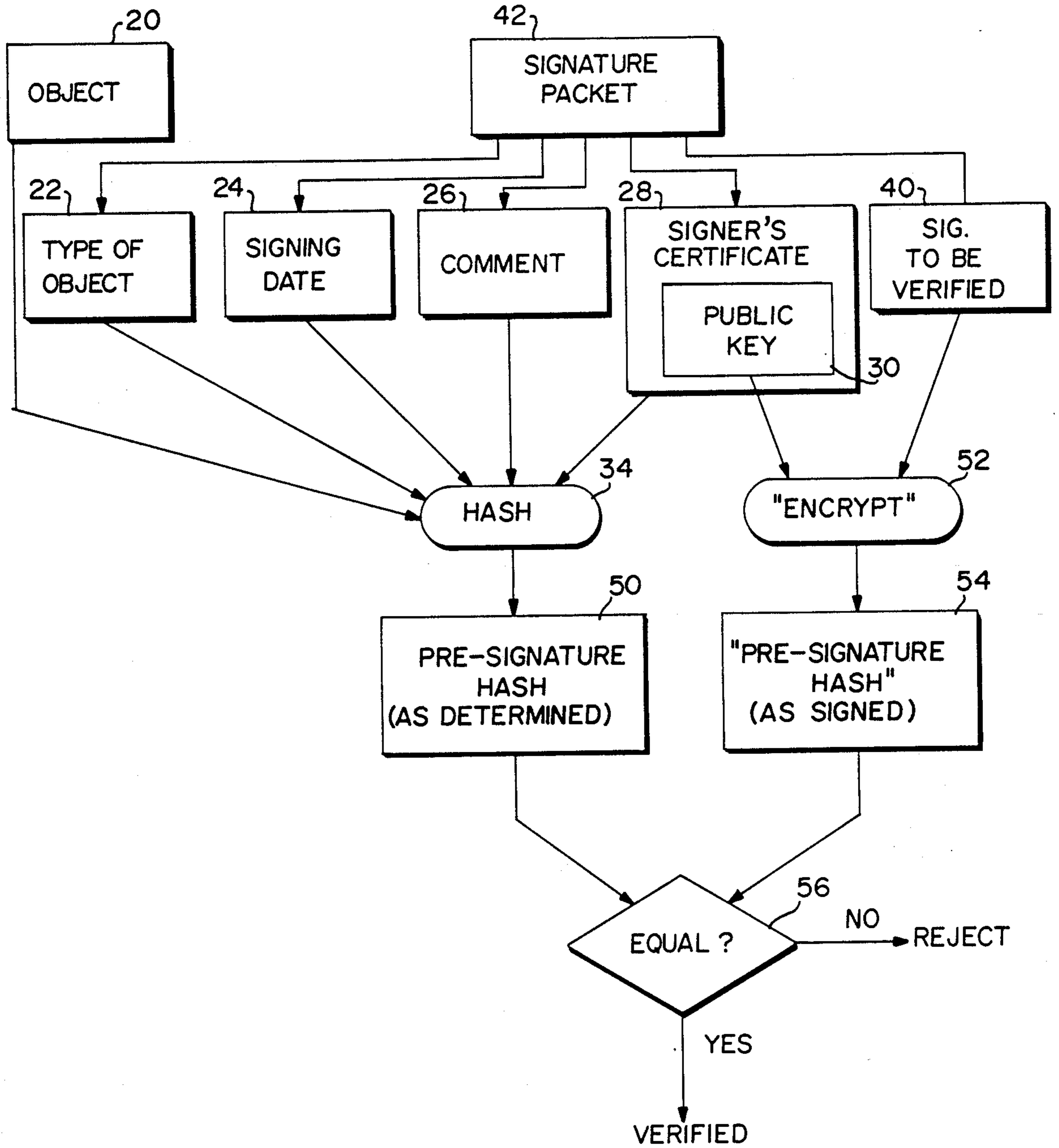
FIG. 3 VERIFY SIGNATURE
