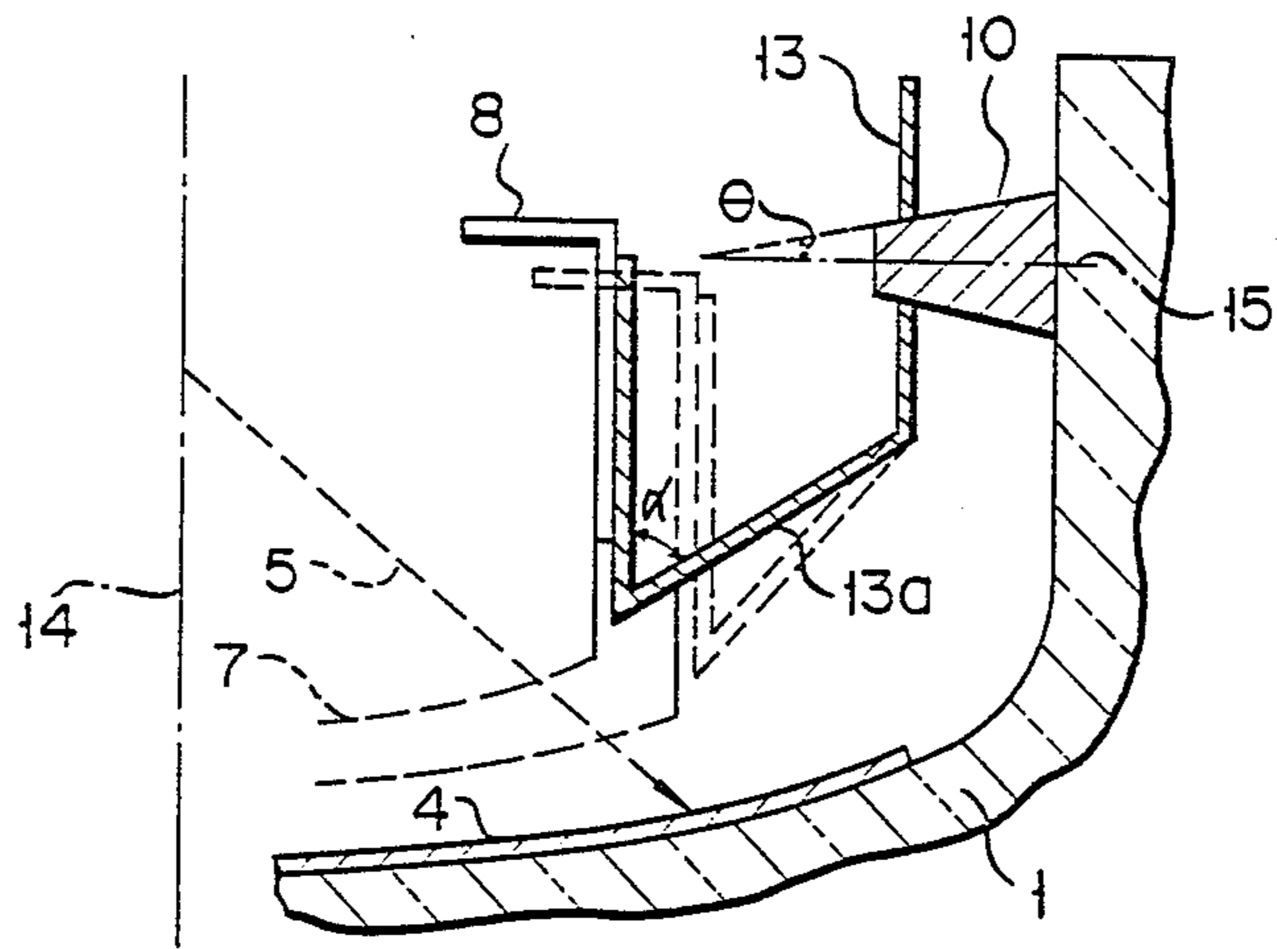
FIG. 1 (PRIOR ART)
