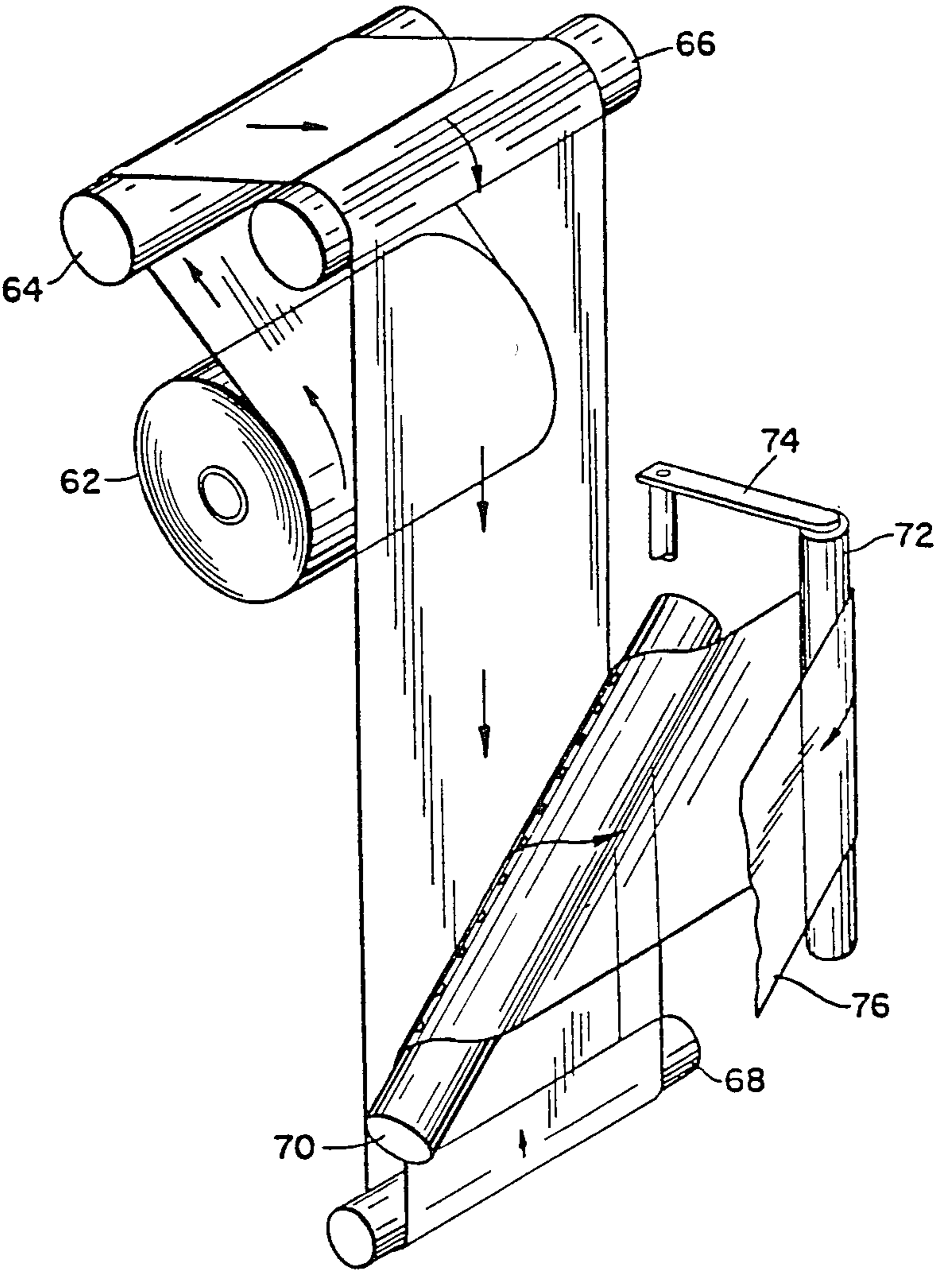
FIG. 8 PRIOR ART
