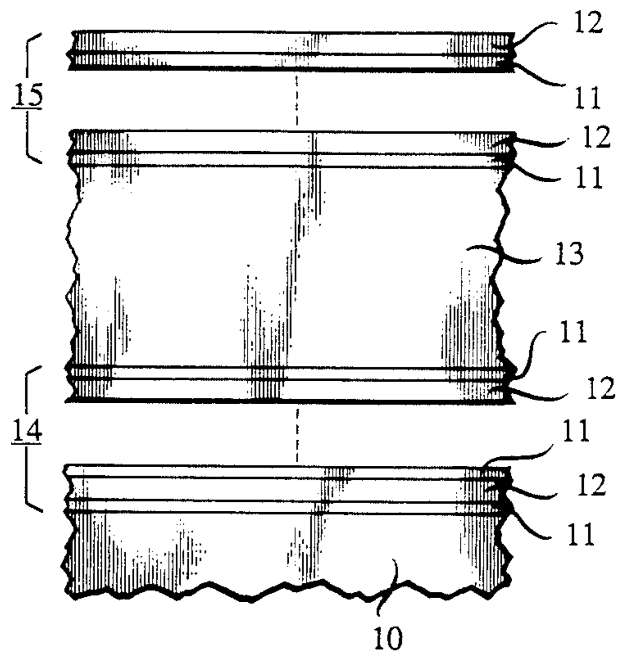
FIG. 1 (PRIOR ART)
