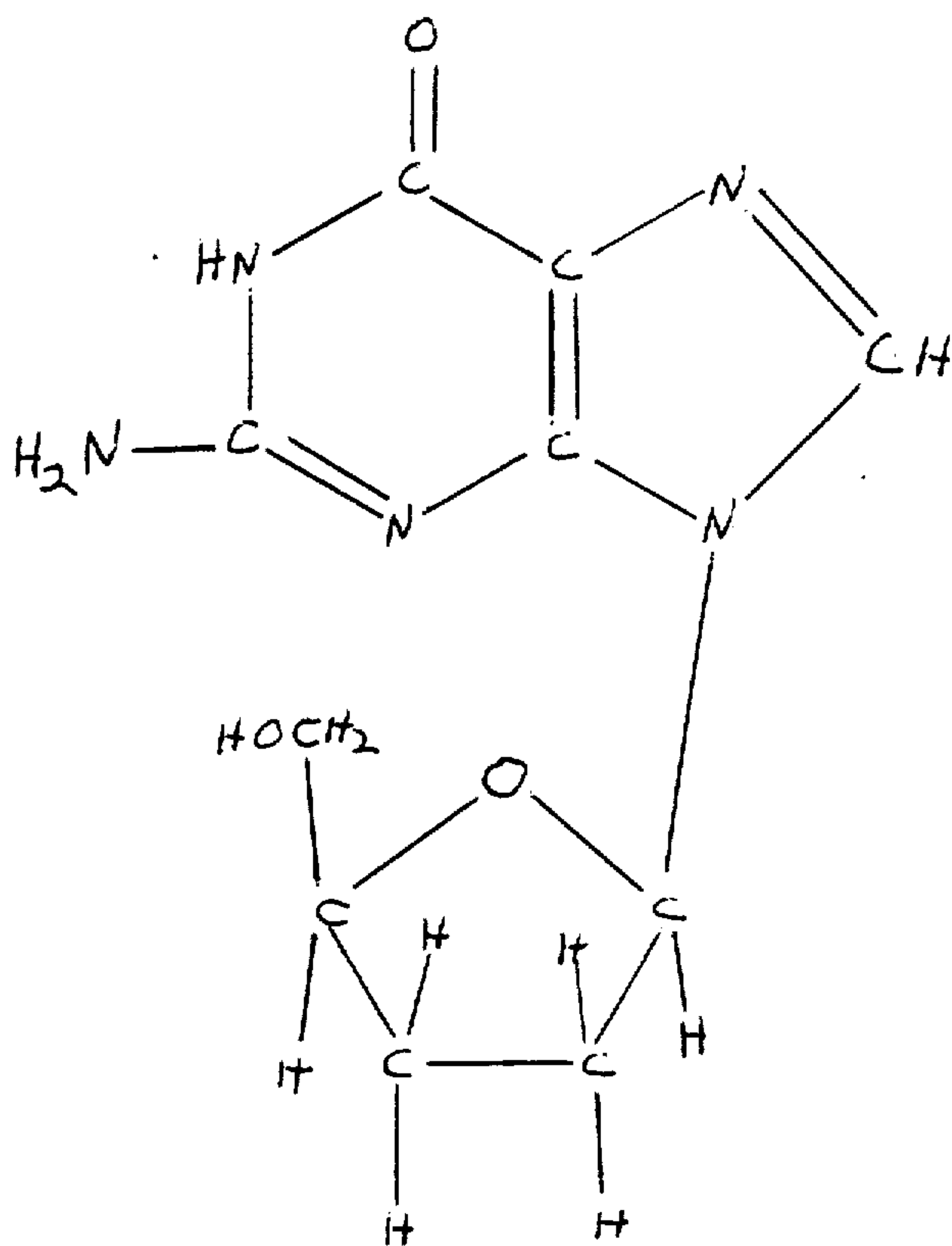
dideoxyguanosine
