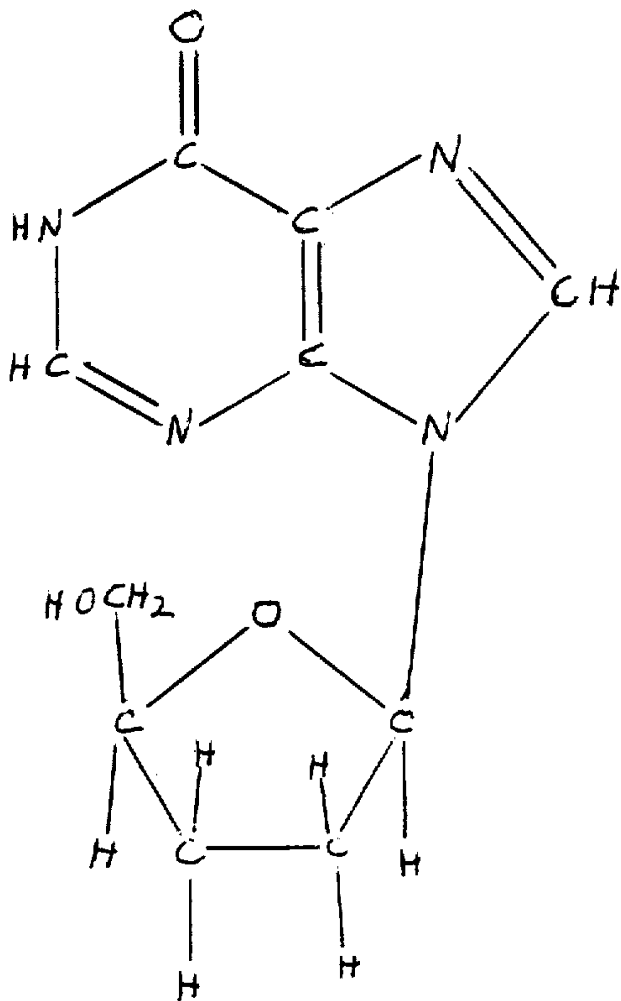
dideoxyinosine
