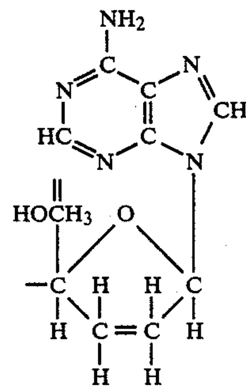
dideoxyadenosine
