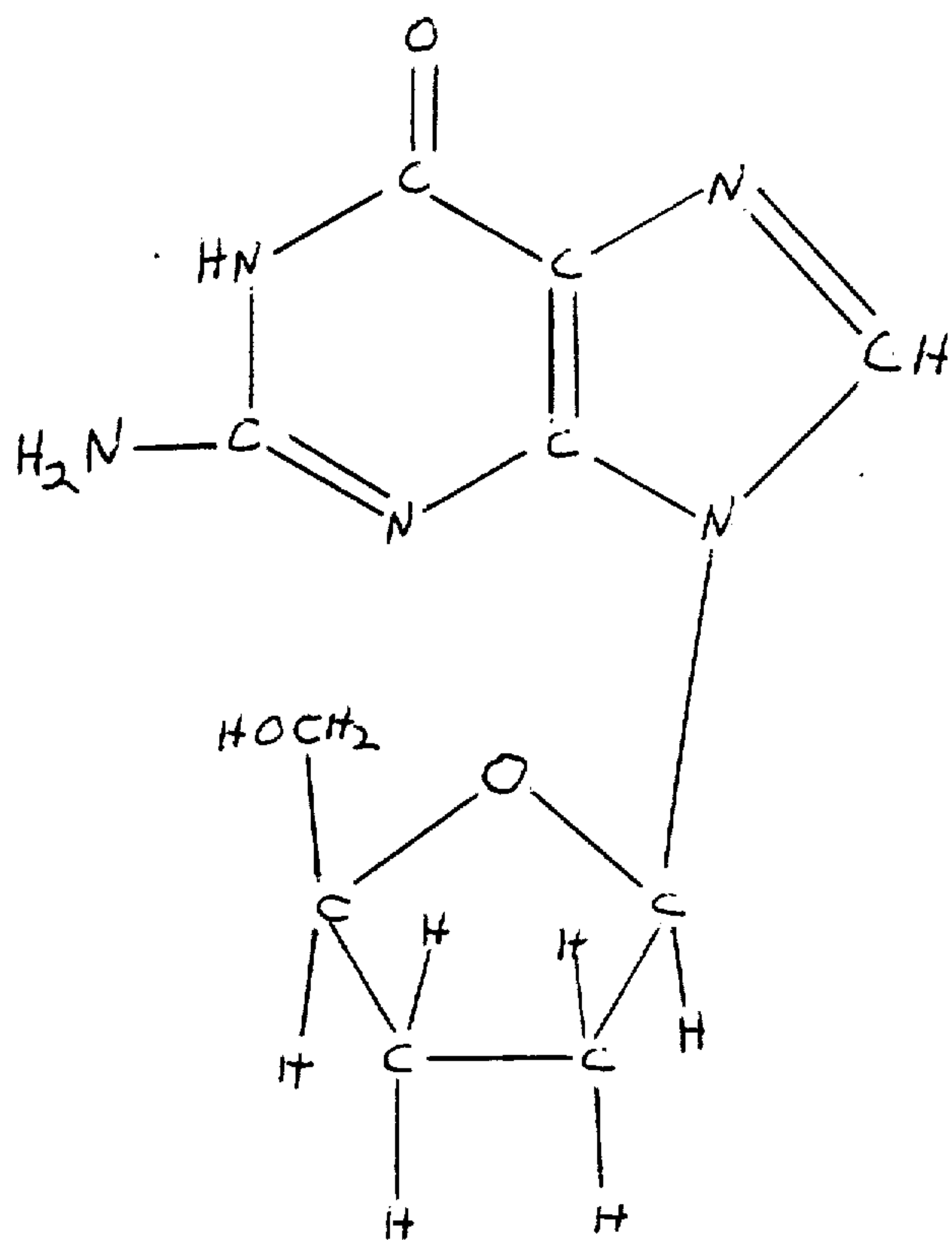
dideoxyguanosine
