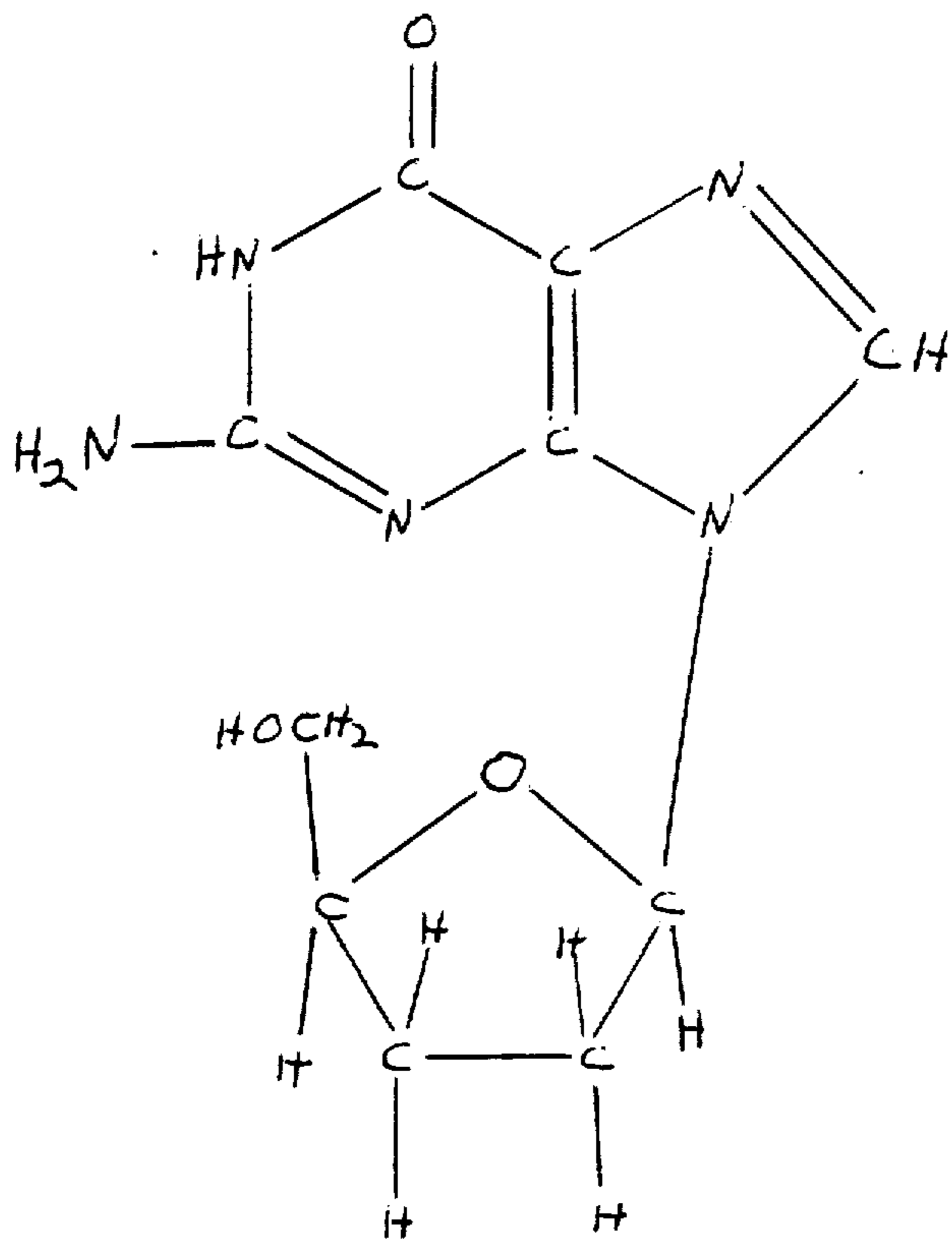
dideoxyguanosine
