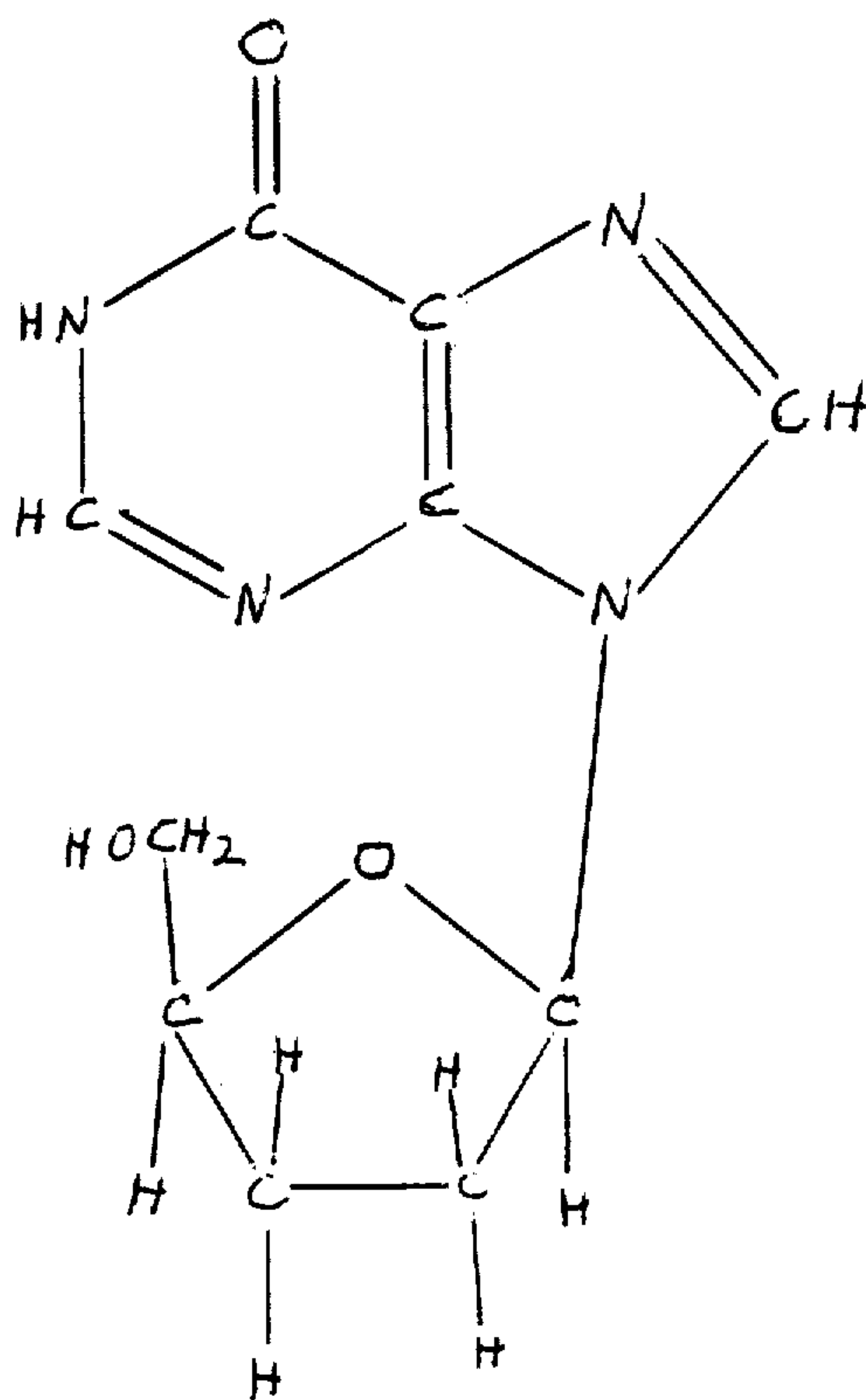
dideoxyinosine
