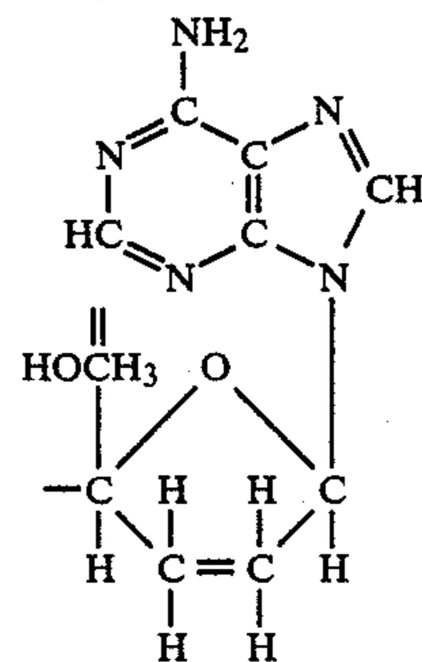
dideoxyadenosine
