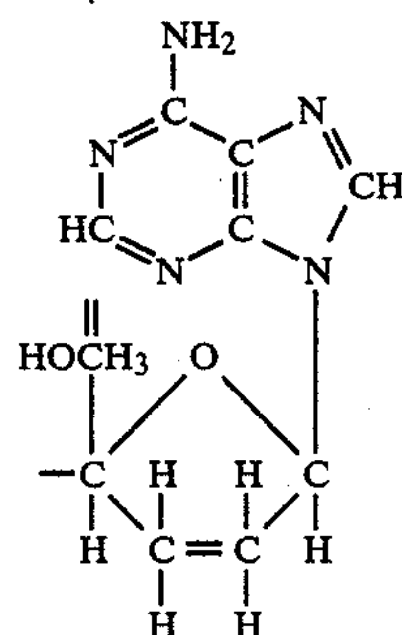
dideoxyadenosine
