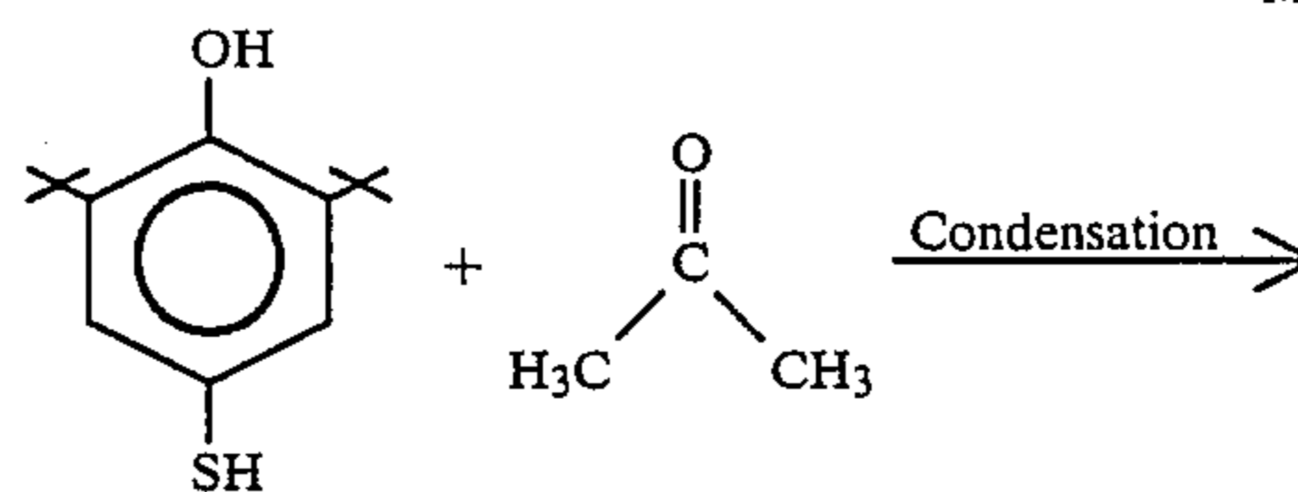
(III) Mercaptophenol
