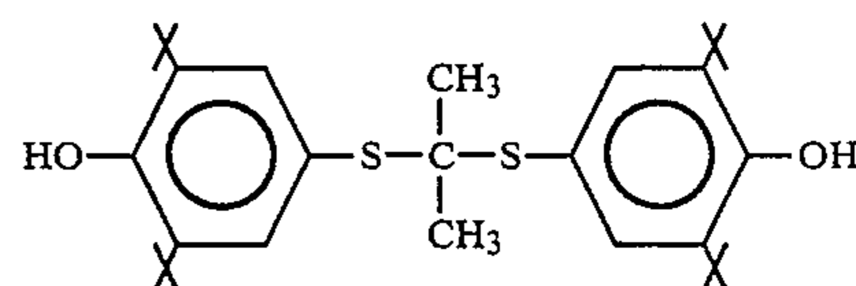
(IV) 4,4'-isopropylidenedithio- bis-(2,6-di-tertiarybutylphenol)
