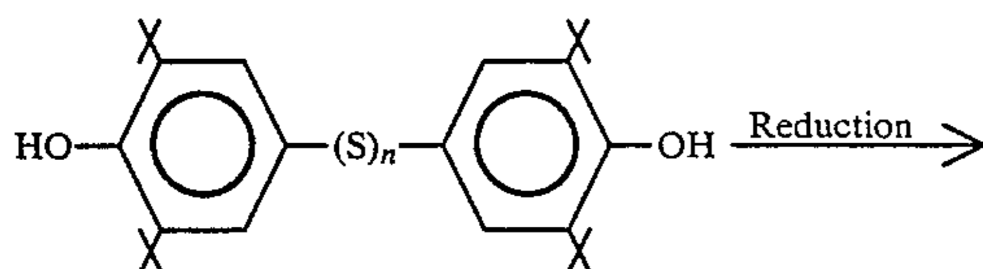
(II) Polysulfide
