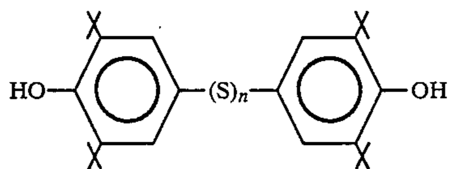
(II) Polysulfide
