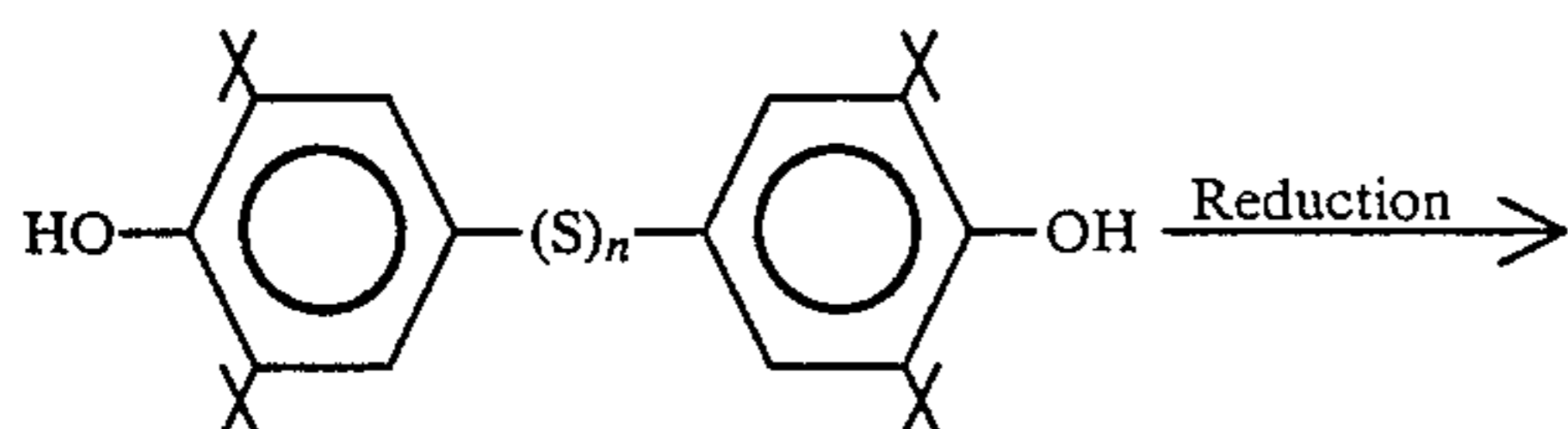
(II) Polysulfide
