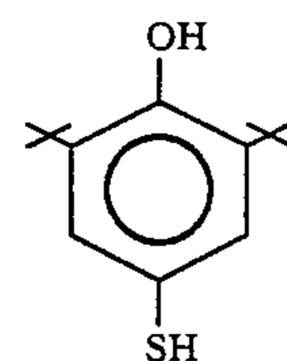
(III) Mercaptophenol
