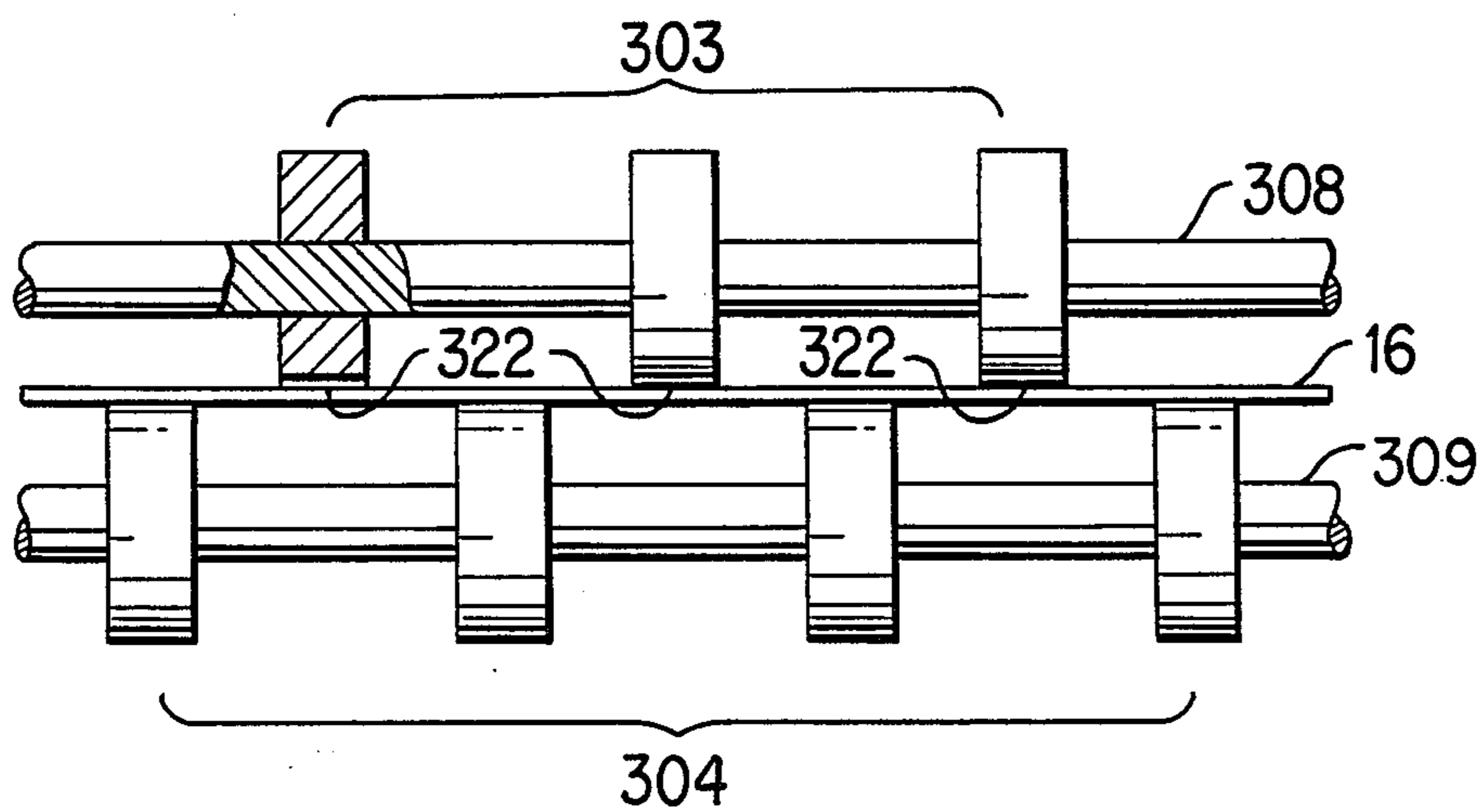
FIG. 7 PRIOR ART
