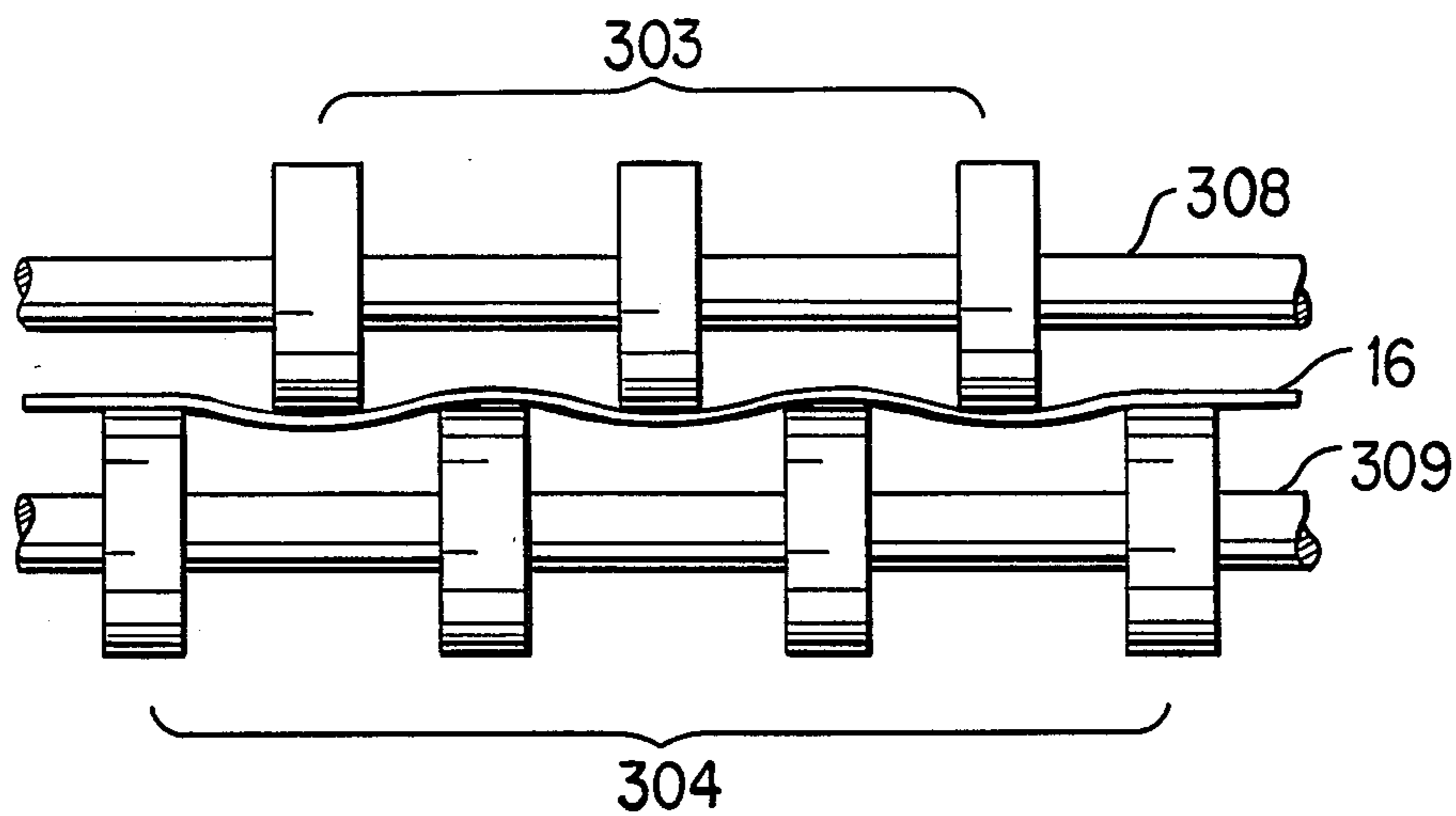
FIG. 6 PRIOR ART
