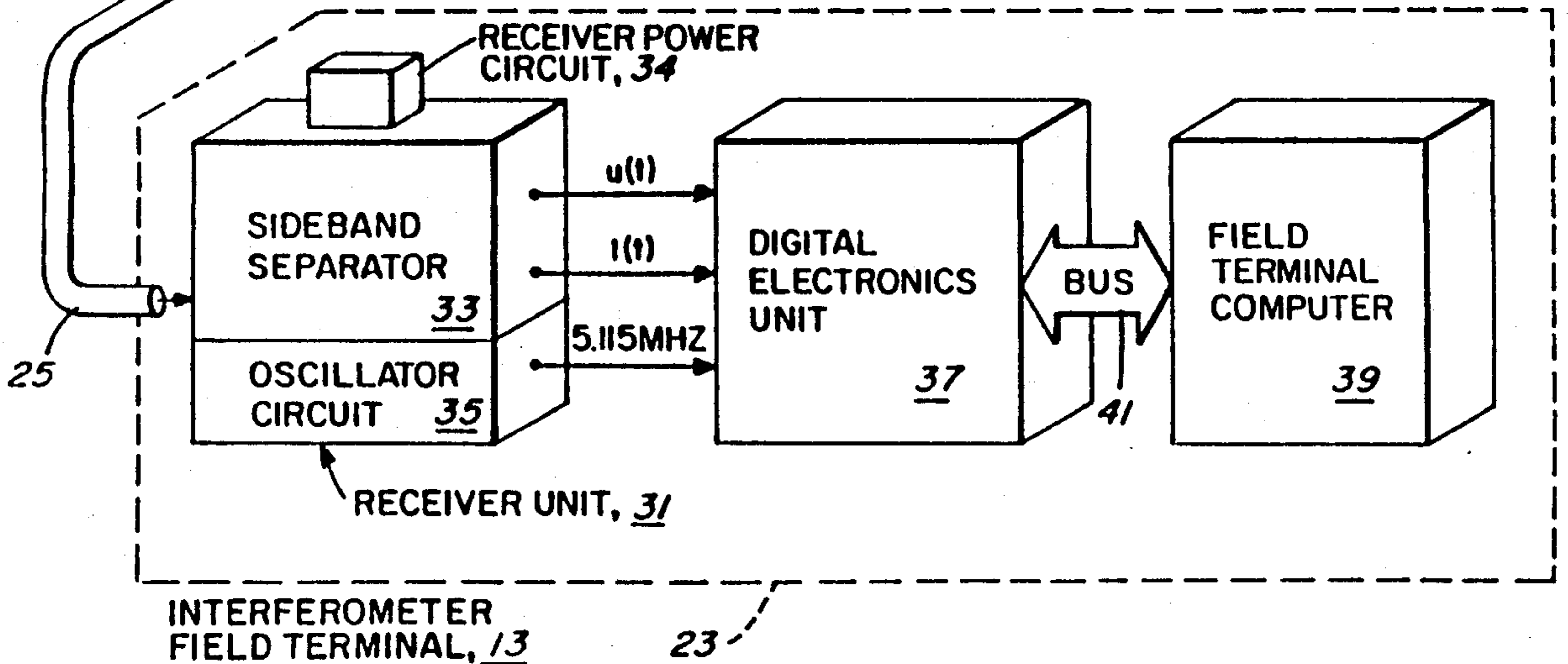
ELECTRONICS ASSEMBLY
