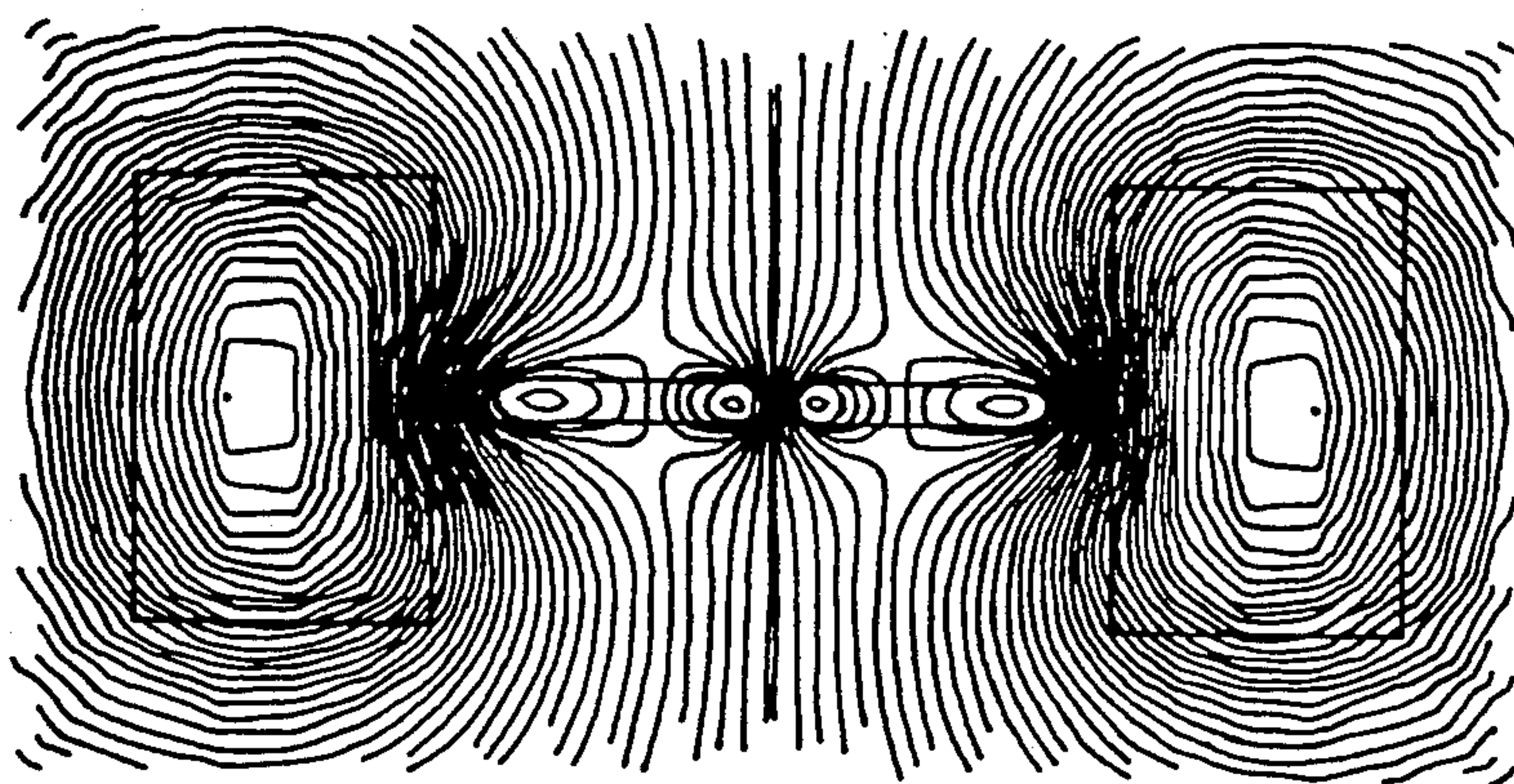
FIG. 11 PRIOR ART
