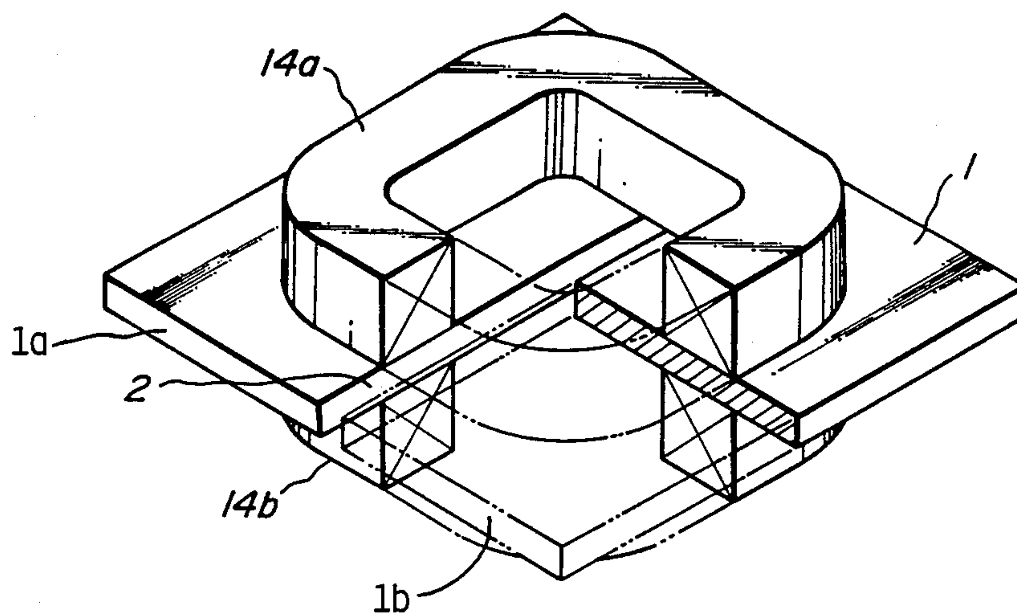
FIG. 7 PRIOR ART
