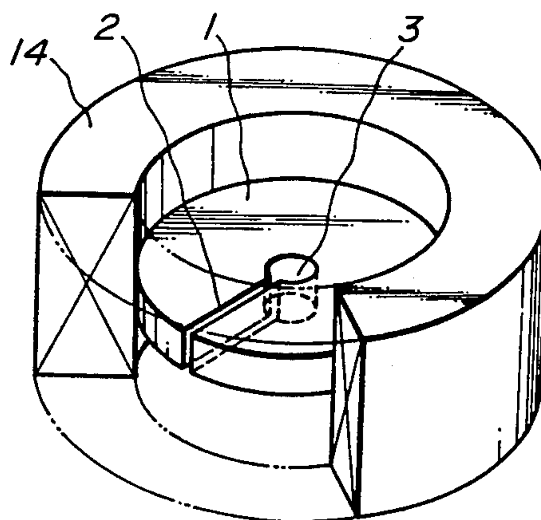
FIG. 8 PRIOR ART
