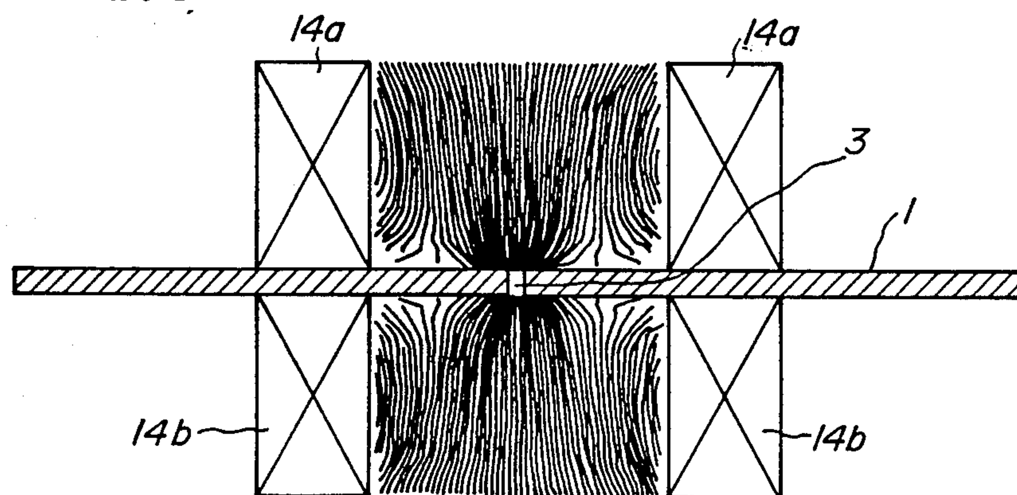
FIG. 10 PRIOR ART
