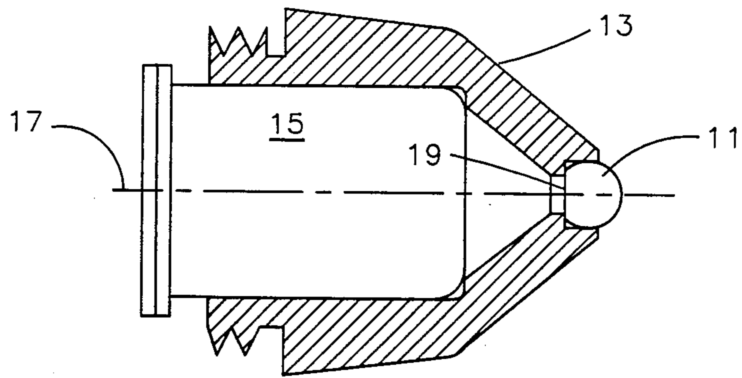
FIG 1 (PRIOR ART)
