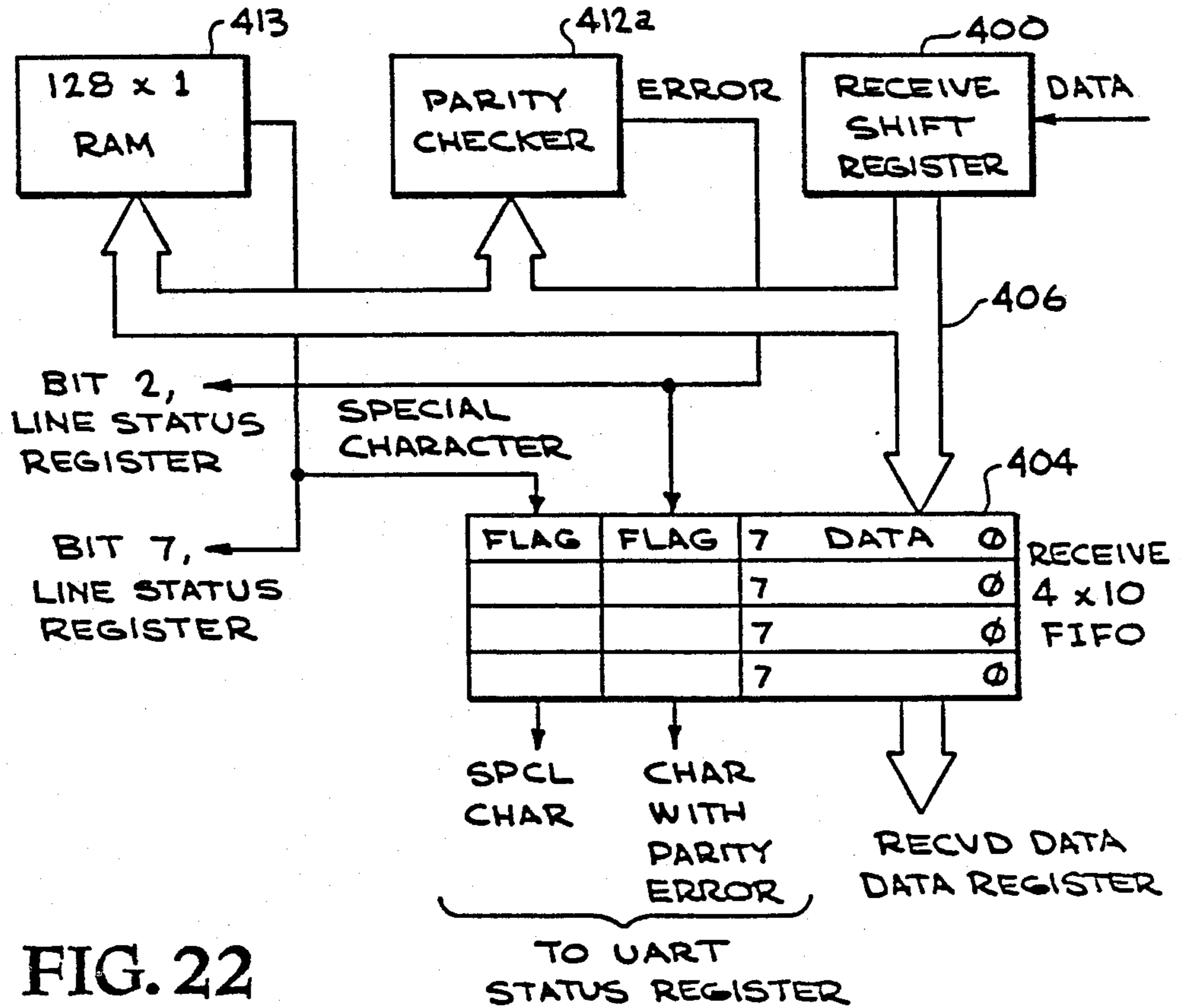
UART PARITY/SPECIAL CHARACTER UNIT
