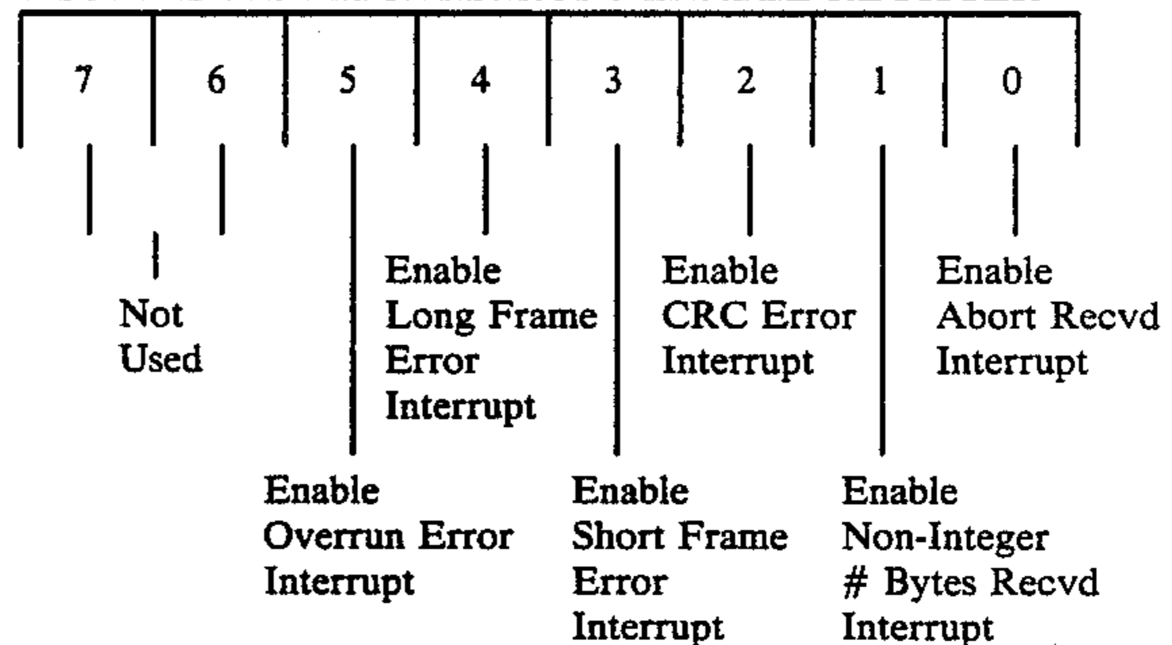
RECEIVE FRAME INTERRUPT ENABLE REGISTER
