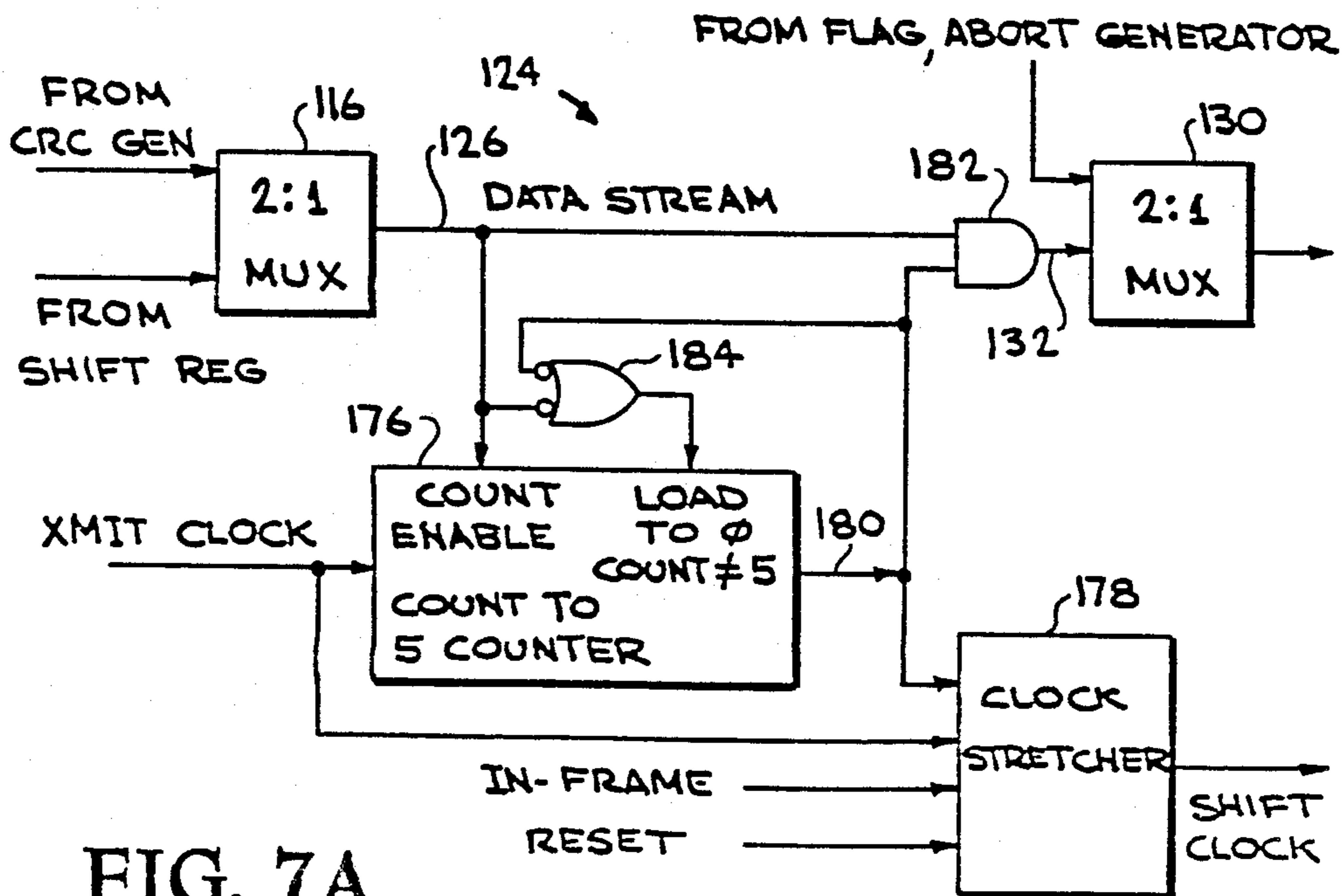
ZERO-BIT INSERTION UNIT
