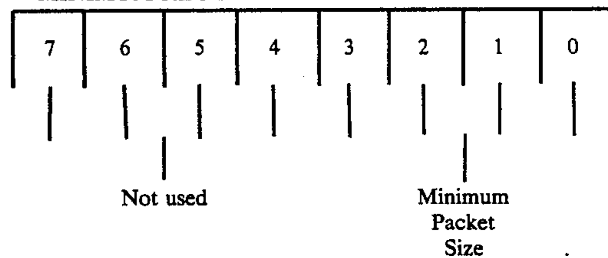
MINIMUM RECEIVE PACKET SIZE REGISTER
