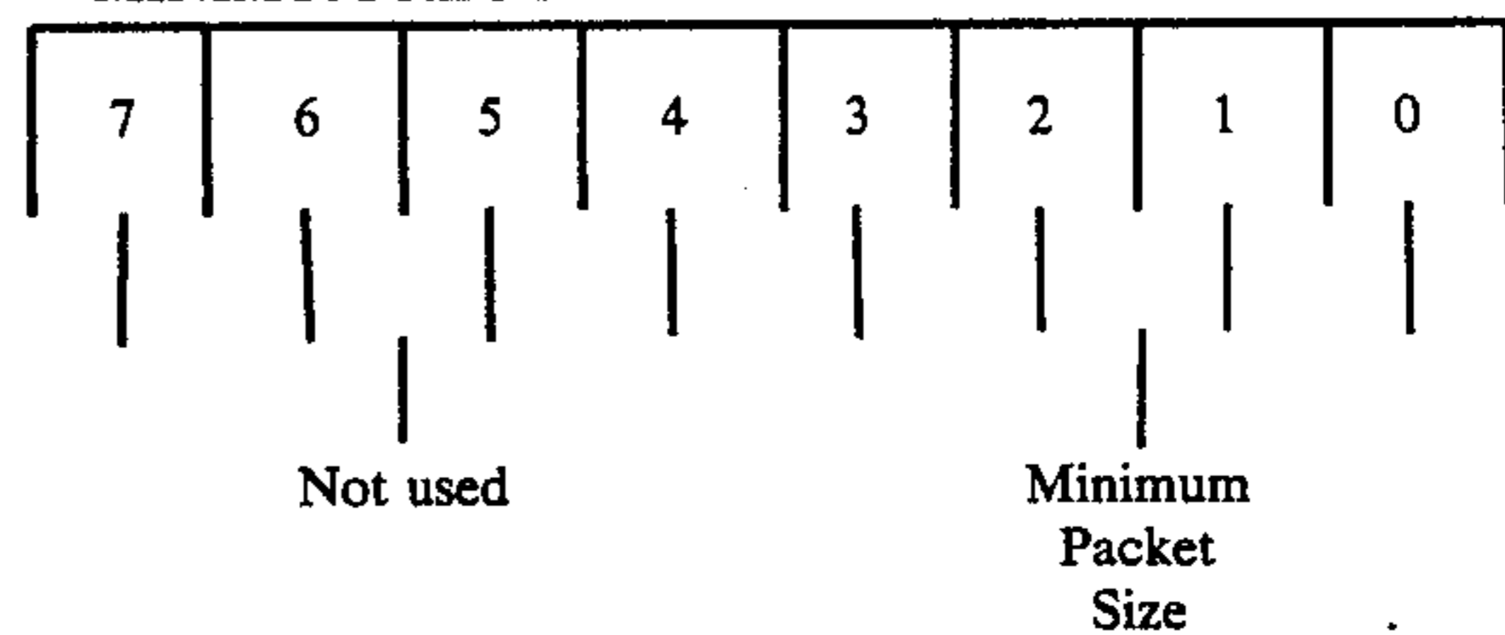
MINIMUM RECEIVE PACKET SIZE REGISTER
