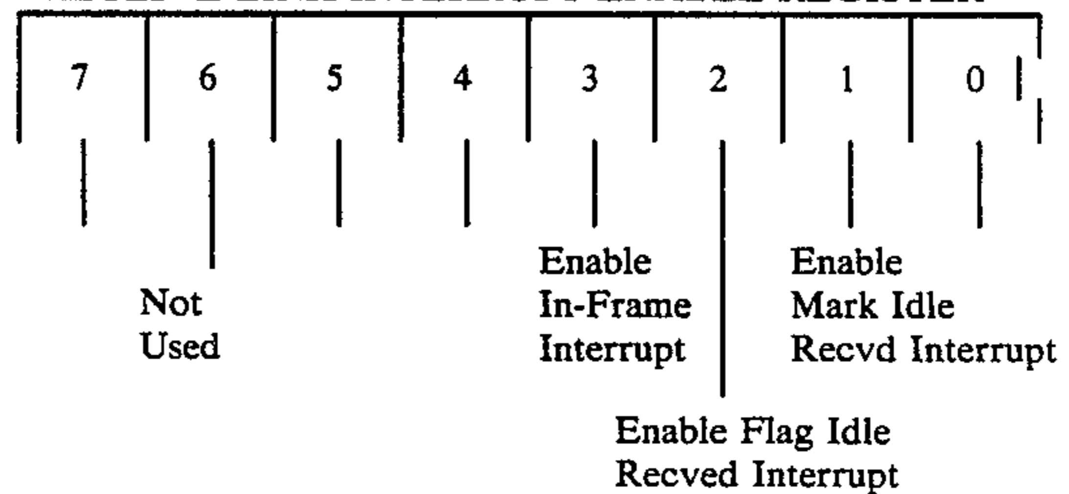
RECEIVE LINK INTERRUPT ENABLE REGISTER
