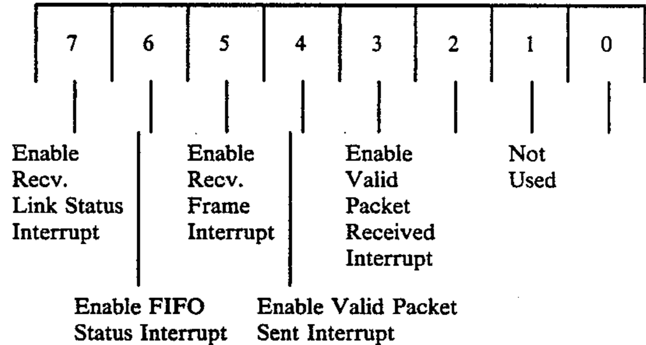
INTERRUPT SOURCE INTERRUPT ENABLE REGISTER
