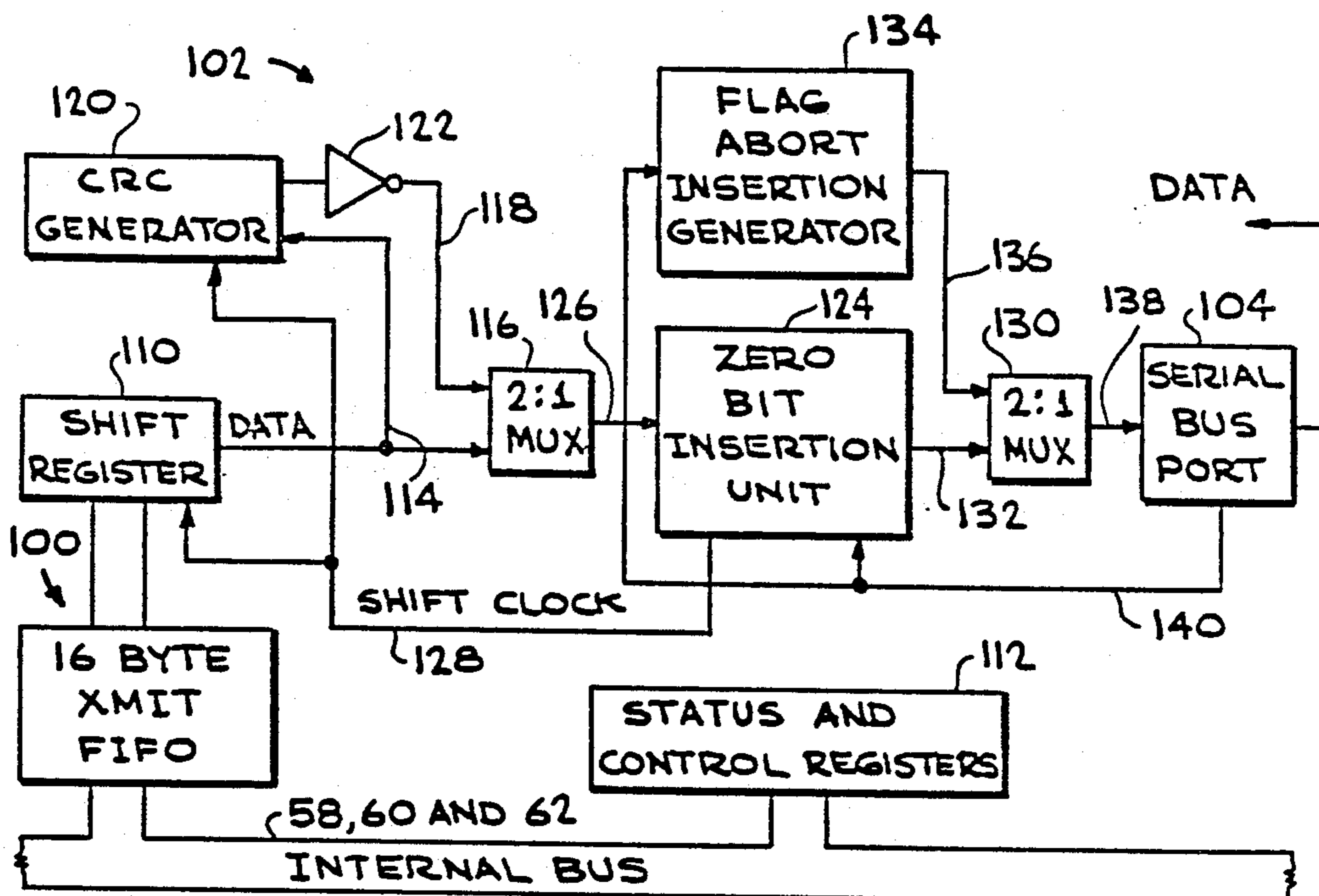
DLC TRANSMITTER
