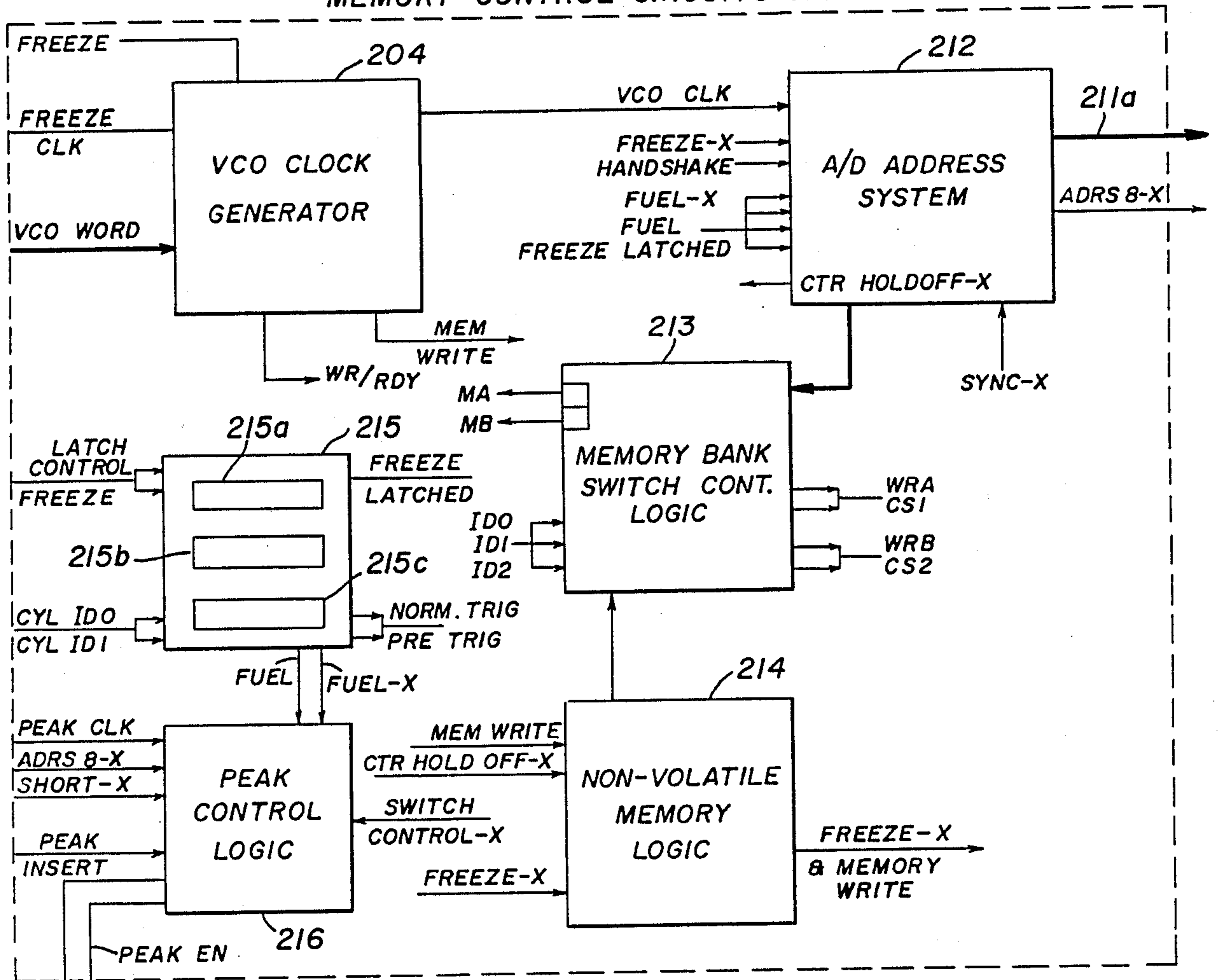
MEMORY CONTROL CIRCUITS 160
