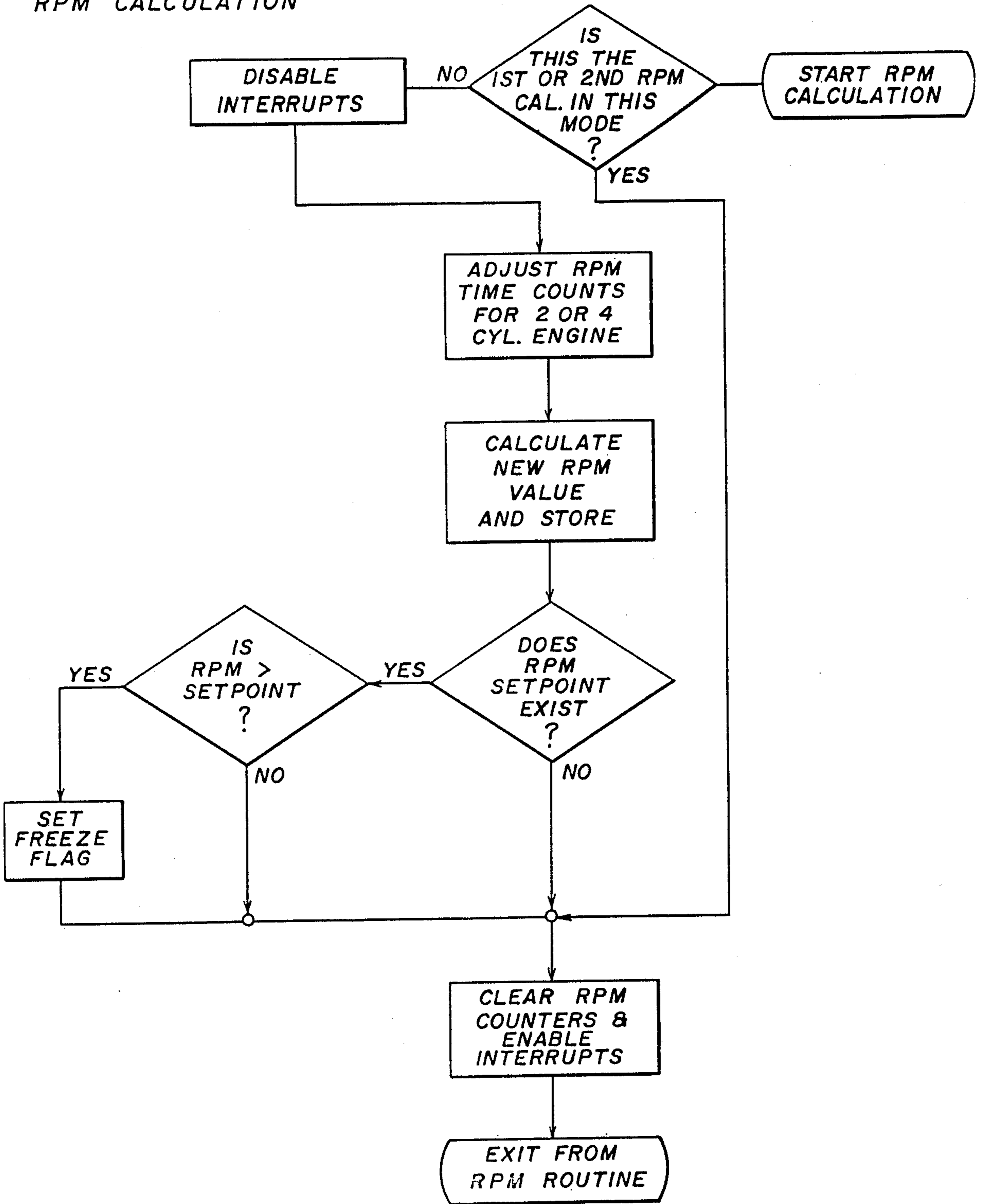
FIG. 41C RPM CALCULATION
