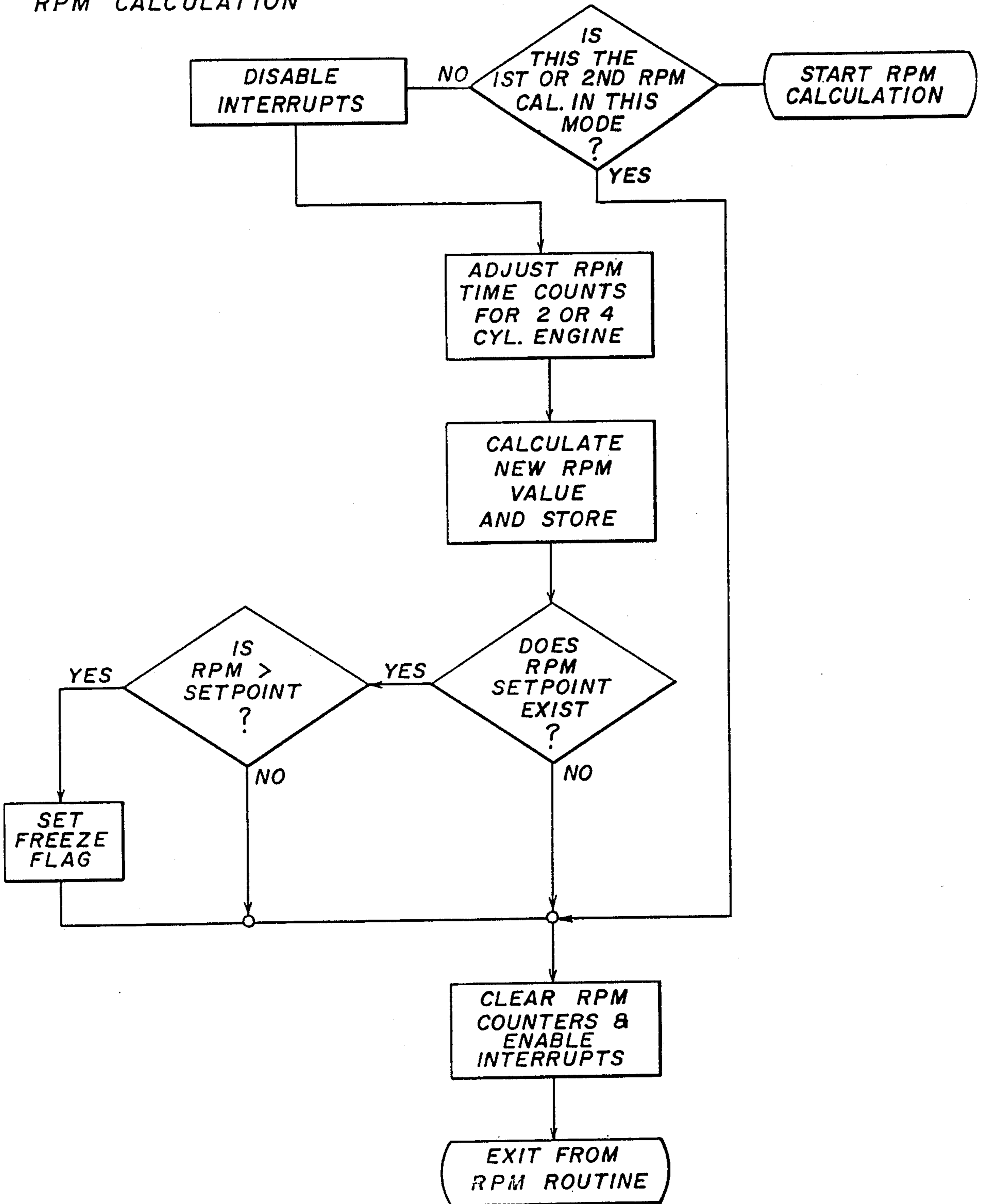
FIG. 41C RPM CALCULATION
