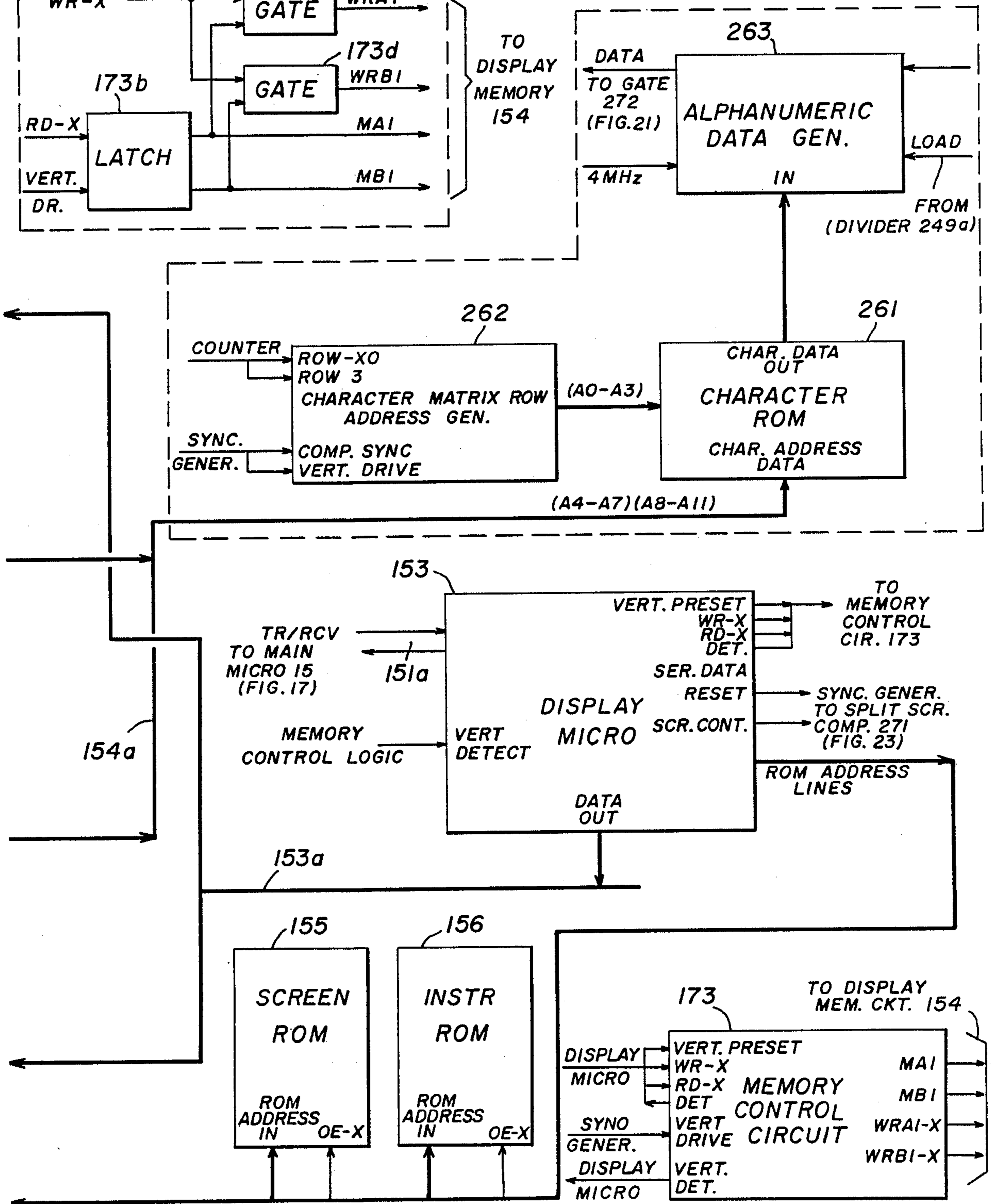
CHARACTER GENERATOR 157
