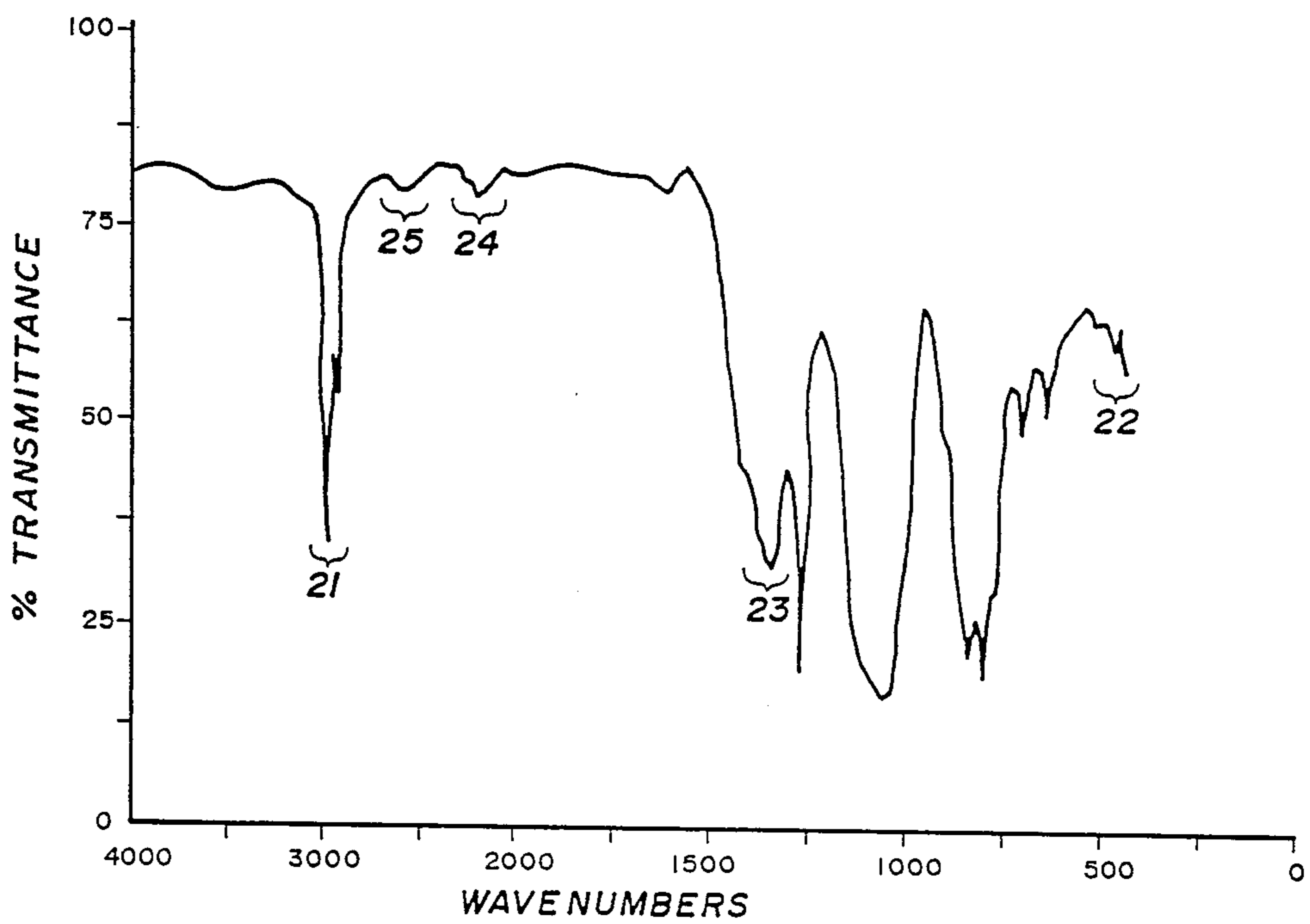
FIGURE 2 FTIR of POLYMER II
