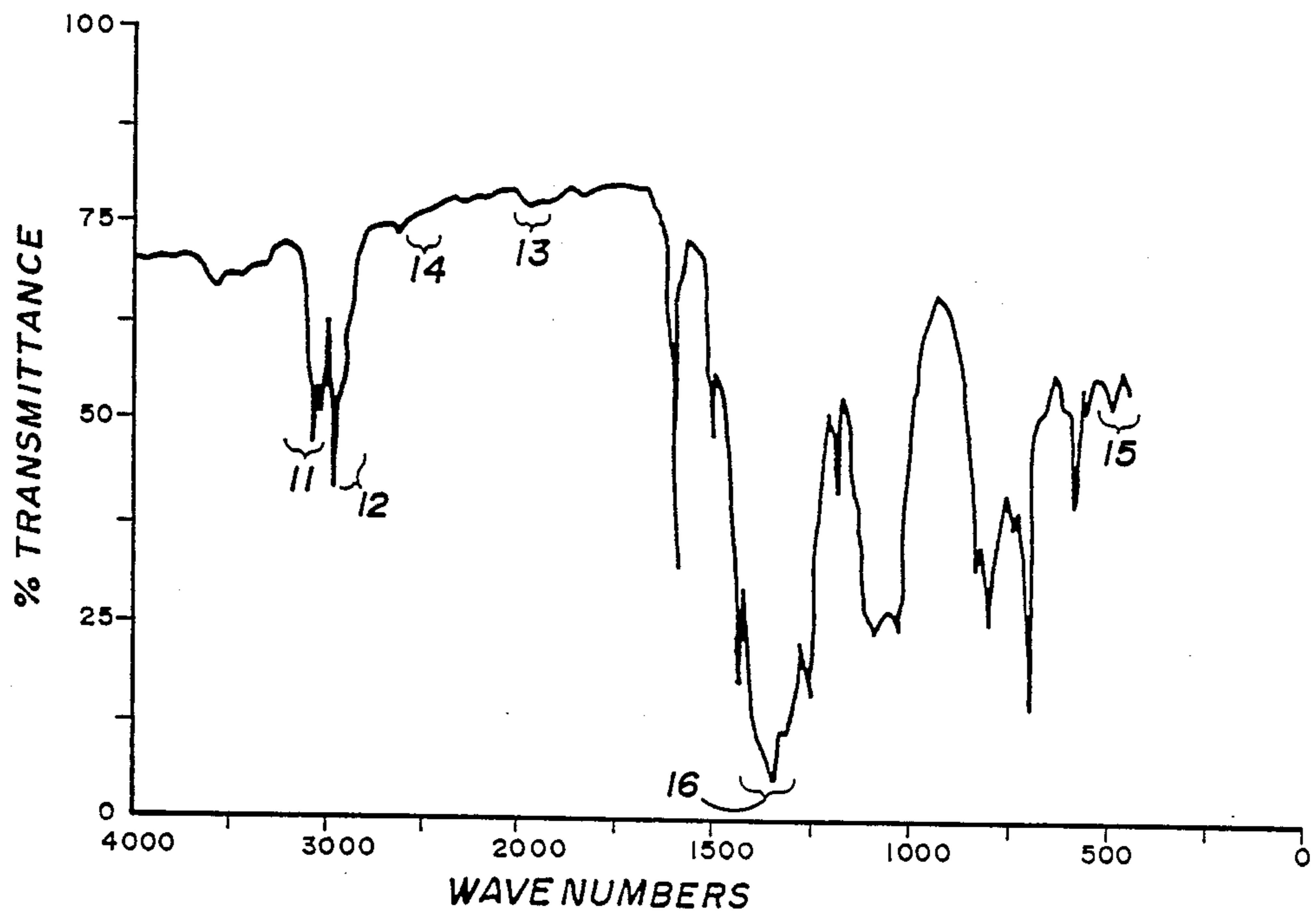
FIGURE 1 FTIR of POLYMER I
