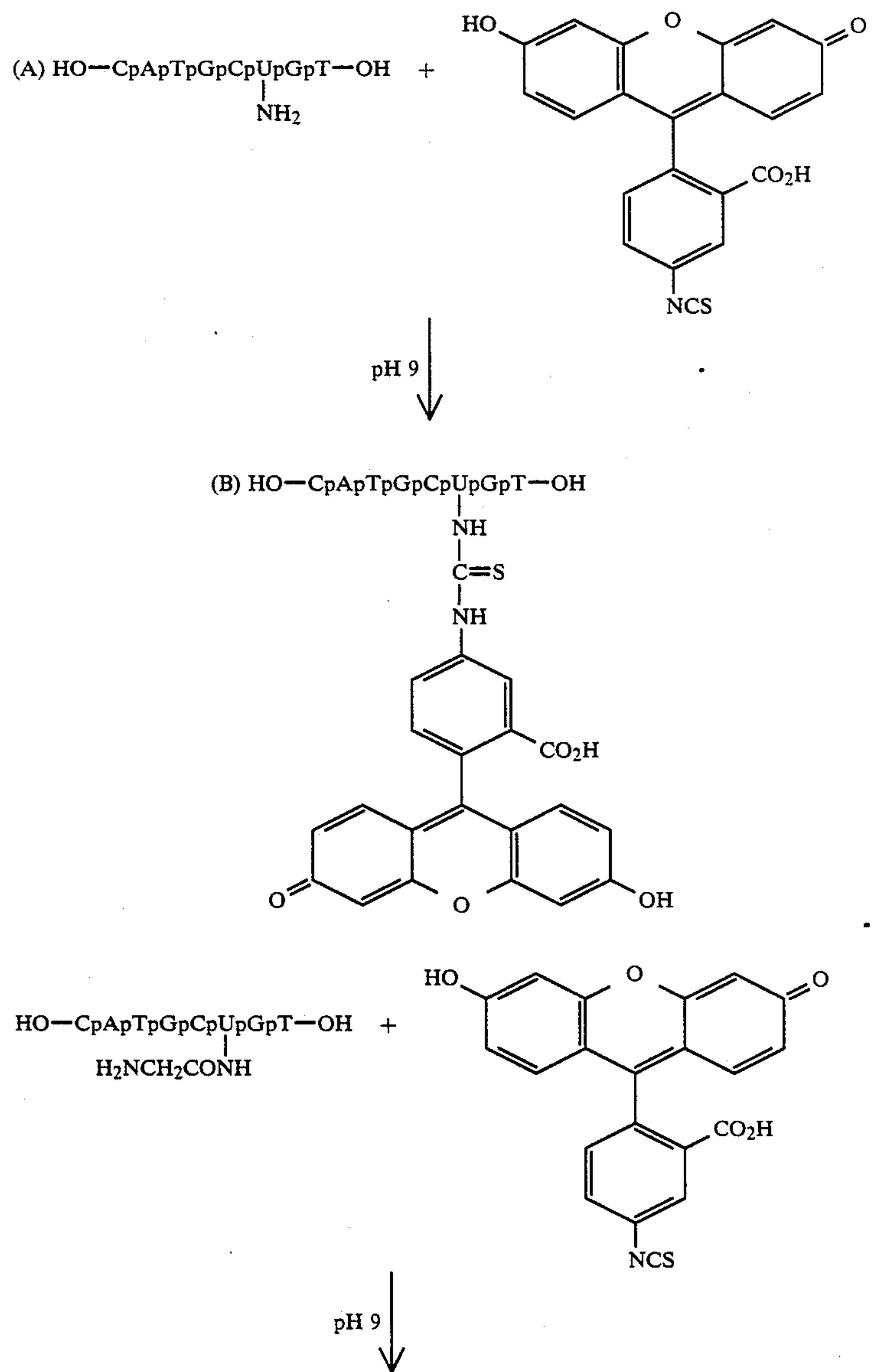
Reaction Scheme for Example 15
