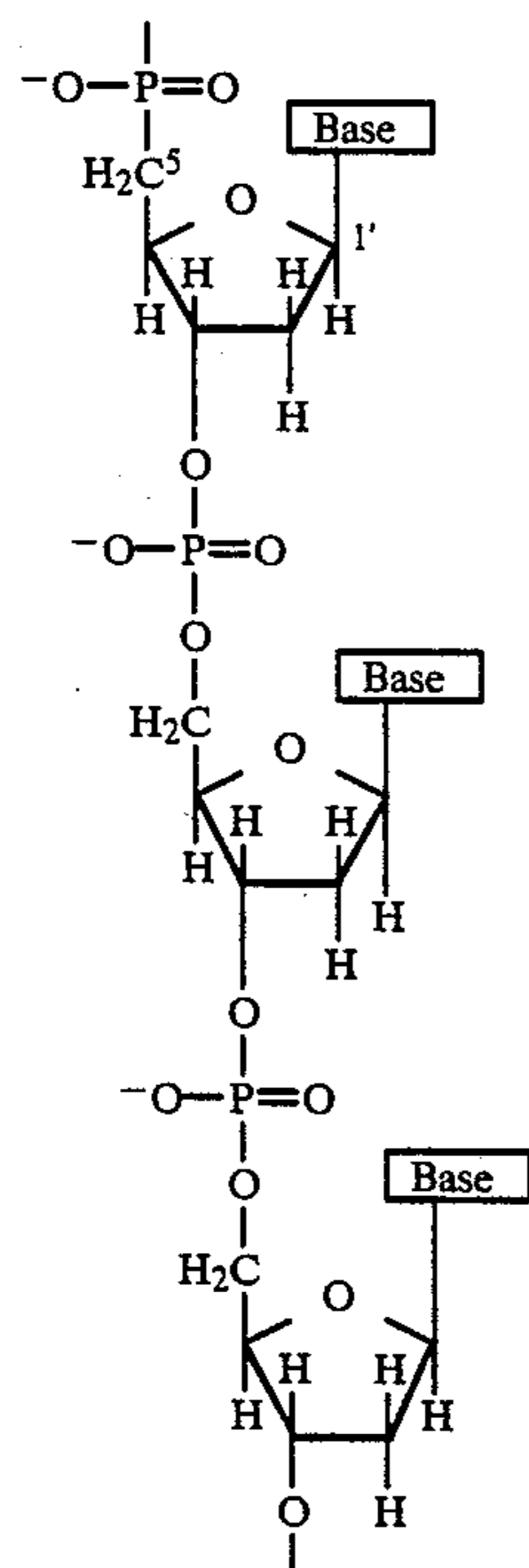
Figure 1 Structure of part of a DNA chain.
