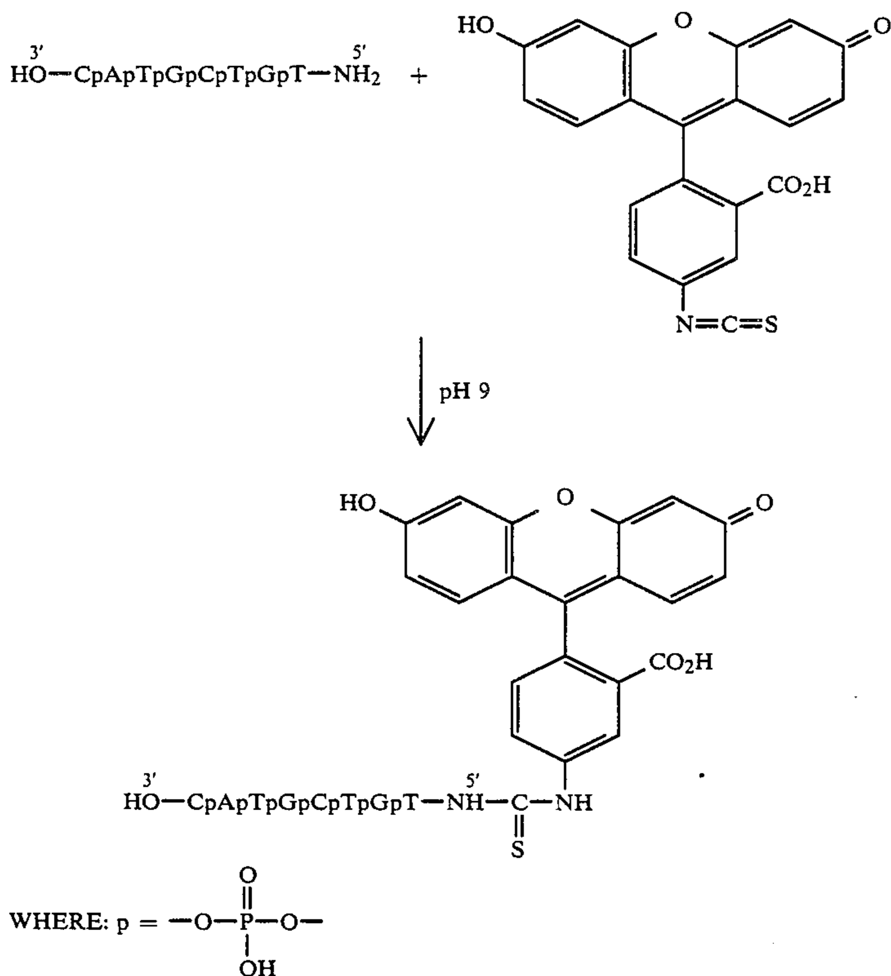
Reaction Scheme For Example 12
